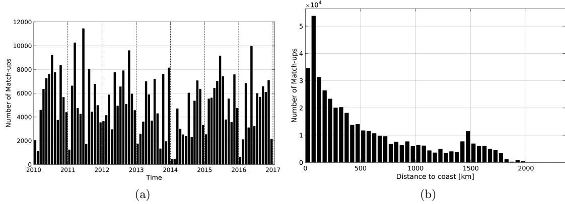
Figure 1: Number of match-ups between TSG-LEGOS-DM and SMOS-L3-CATDS-CPDC-V3-MONTHLY-25KM SSS as a function of time (a) and as function of the distance to coast (b) over the North Atlantic Ocean Pi-MEP region and for the full satellite product period.
