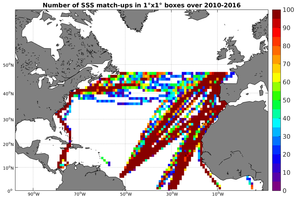
Figure 4: Number of SSS match-ups between TSG-LEGOS-DM SSS and the SMOS-L3-CATDS-CPDC-V3-MONTHLY-25KM SSS product for the North Atlantic Ocean Pi-MEP region over 1°x1° boxes and for the full satellite product period.
