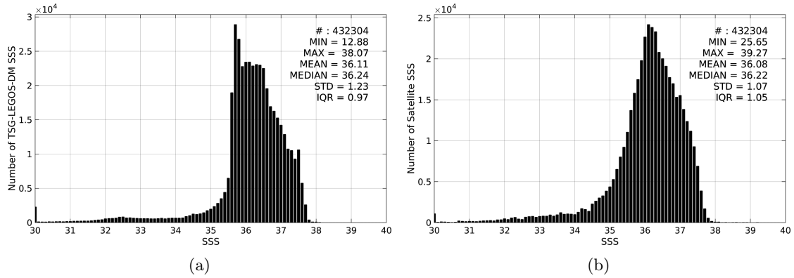
Figure 2: Histograms of SSS from TSG-LEGOS-DM (a) and SMOS-L3-CATDS-CPDC-V3-MONTHLY-25KM (b) considering all match-up pairs per bins of 0.1 over the North Atlantic Ocean Pi-MEP region and for the full satellite product period.
