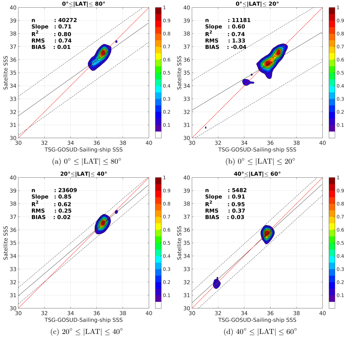
Figure 9: Contour maps of the concentration of SMOS-L3-CATDS-CPDC-V3-MONTHLY-25KM SSS (y-axis) versus TSG-GOSUD-Sailing-ship SSS (x-axis) at match-up pairs for different latitude bands. For each plot, the red line shows x=y . The black thin and dashed lines indicate a linear fit through the data cloud and the \pm 95\% confidence levels, respectively. The number match-up pairs n , the slope and R^2 coefficient of the linear fit, the root mean square (RMS) and the mean bias between satellite and in situ data are indicated for each latitude band in each plots.
