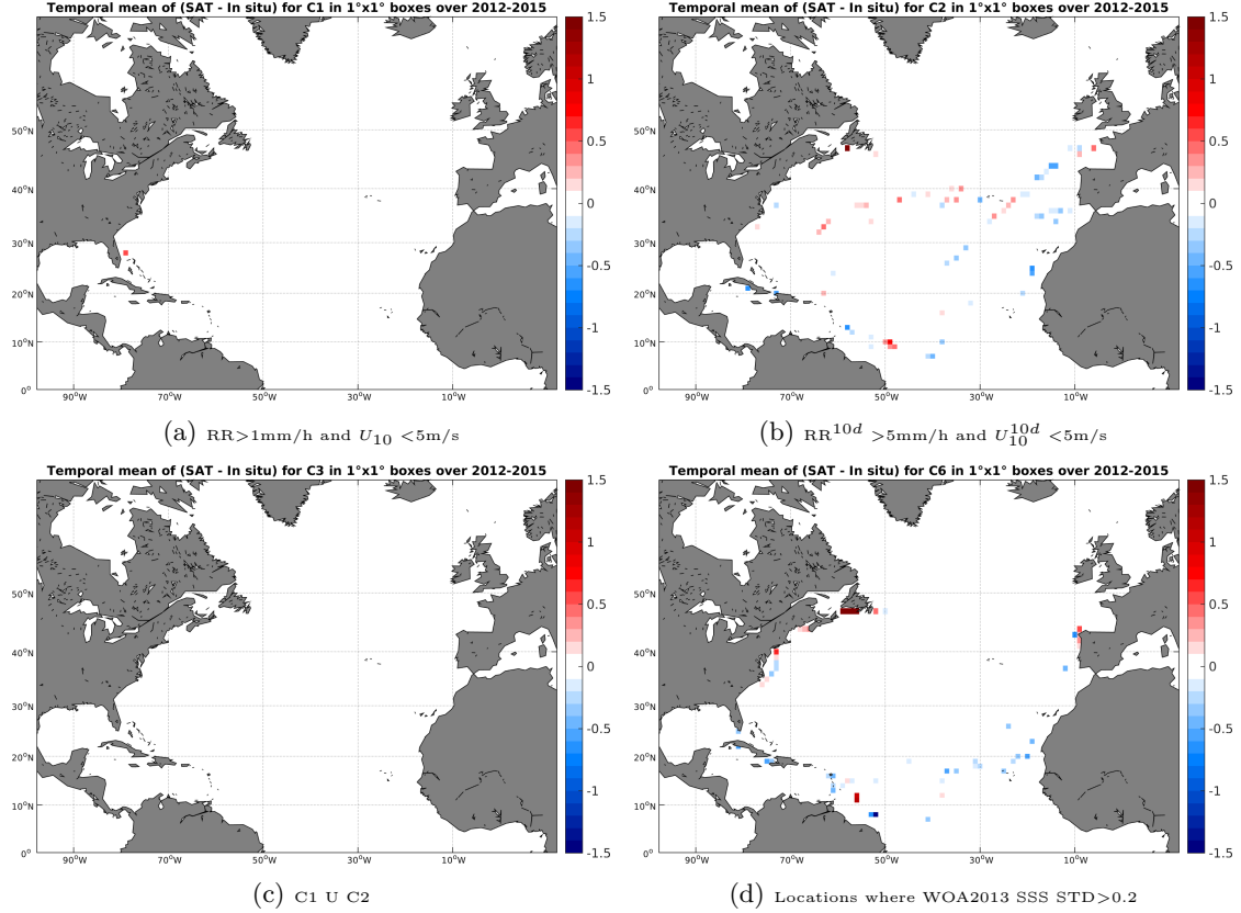
Figure 12: Temporal mean gridded over spatial boxes of size 1^\circ \times 1^\circ of \Delta SSS (SMOS-L3-CATDS-CPDC-V3-MONTHLY-25KM - TSG-GOSUD-Sailing-ship) for 4 different subdatasets corresponding to: RR > 1mm/h and U_{10} < 5 m/s (a), RR^{10d} > 5 mm/h and U_{10}^{10d} < 5 m/s (b), C1 U C2 (c), Locations where WOA2013 SSS STD > 0.2 (d).
