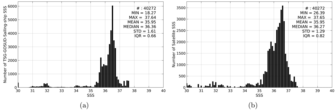
Figure 2: Histograms of SSS from TSG-GOSUD-Sailing-ship (a) and SMOS-L3-CATDS-CPDC-V3-MONTHLY-25KM (b) considering all match-up pairs per bins of 0.1 over the North Atlantic Ocean Pi-MEP region and for the full satellite product period.
