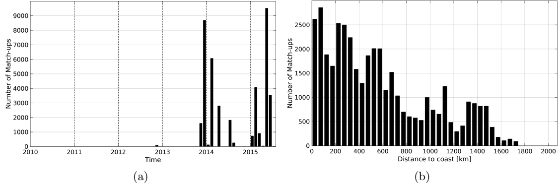
Figure 1: Number of match-ups between TSG-GOSUD-Sailing-ship and SMOS-L3-CATDS-CPDC-V3-MONTHLY-25KM SSS as a function of time (a) and as function of the distance to coast (b) over the North Atlantic Ocean Pi-MEP region and for the full satellite product period.
