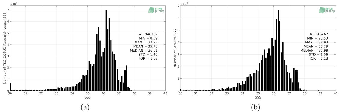
Figure 2: Histograms of SSS from TSG-GOSUD-Research-vessel (a) and SMOS-L3-CATDS-CPDC-V3-MONTHLY-25KM (b) considering all match-up pairs per bins of 0.1 over the North Atlantic Ocean Pi-MEP region and for the full satellite product period.
