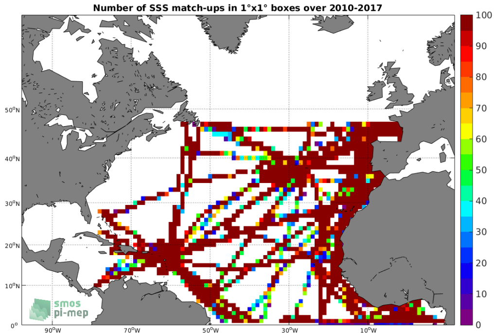
Figure 4: Number of SSS match-ups between TSG-GOSUD-Research-vessel SSS and the SMOS-L3-CATDS-CPDC-V3-MONTHLY-25KM SSS product for the North Atlantic Ocean Pi-MEP region over 1^\circ \times 1^\circ boxes and for the full satellite product period.
