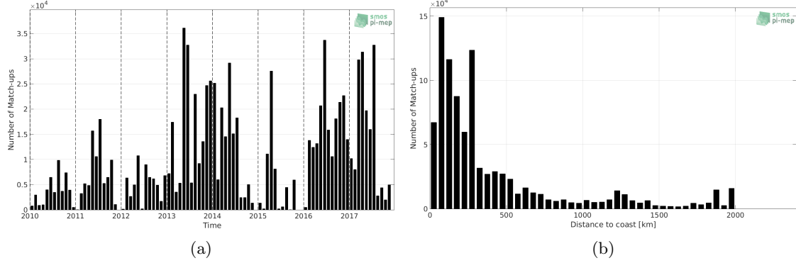
Figure 1: Number of match-ups between TSG-GOSUD-Research-vessel and SMOS-L3-CATDS-CPDC-V3-MONTHLY-25KM SSS as a function of time (a) and as function of the distance to coast (b) over the North Atlantic Ocean Pi-MEP region and for the full satellite product period.
