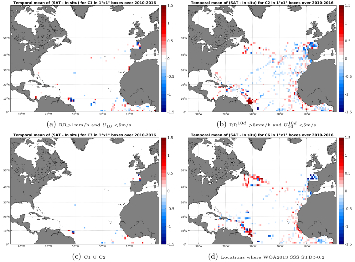
Figure 12: Temporal mean gridded over spatial boxes of size 1^\circ \times 1^\circ of \Delta SSS (SMOS-L3-CATDS-CPDC-V3-MONTHLY-25KM - TSG-GOSUD-Research-vessel) for 4 different subdatasets corresponding to: RR > 1mm/h and U_{10} < 5 m/s (a), RR^{10d} > 5 mm/h and U_{10}^{10d} < 5 m/s (b), C1 U C2 (c), Locations where WOA2013 SSS STD > 0.2 (d).
