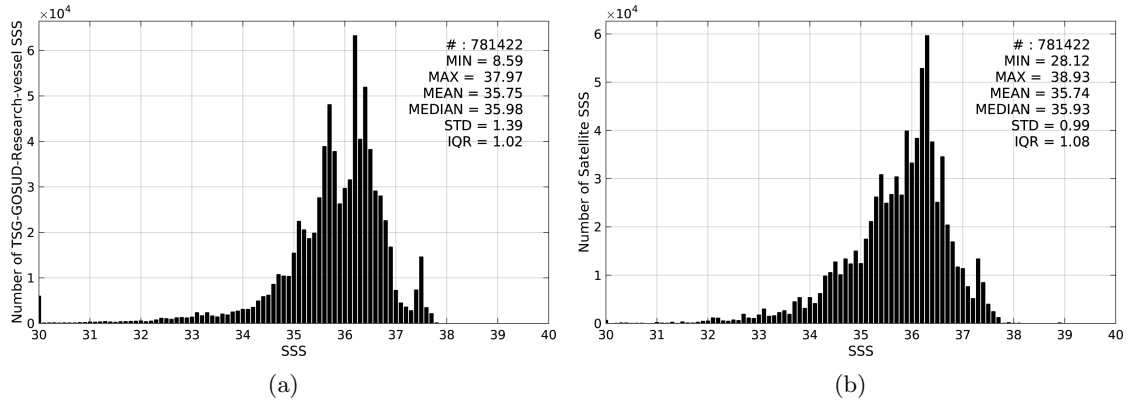
Figure 2: Histograms of SSS from TSG-GOSUD-Research-vessel (a) and SMOS-L3-CATDS-CPDC-V3-MONTHLY-25KM (b) considering all match-up pairs per bins of 0.1 over the North Atlantic Ocean Pi-MEP region and for the full satellite product period.
