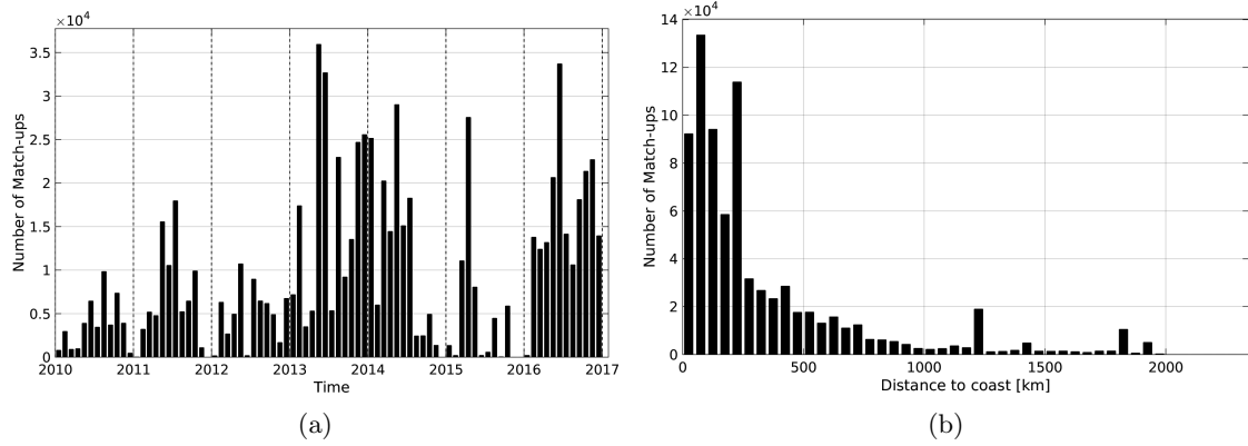
Figure 1: Number of match-ups between TSG-GOSUD-Research-vessel and SMOS-L3-CATDS-CPDC-V3-MONTHLY-25KM SSS as a function of time (a) and as function of the distance to coast (b) over the North Atlantic Ocean Pi-MEP region and for the full satellite product period.
