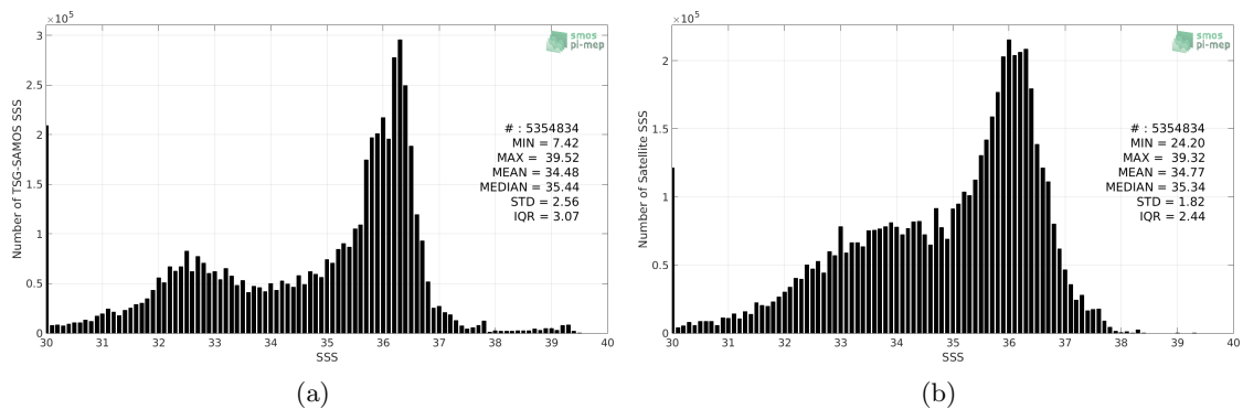
Figure 2: Histograms of SSS from TSG-SAMOS (a) and SMOS-L3-CATDS-CPDC-V3-10DAYS-25KM (b) considering all match-up pairs per bins of 0.1 over the North Atlantic Ocean Pi-MEP region and for the full satellite product period.
