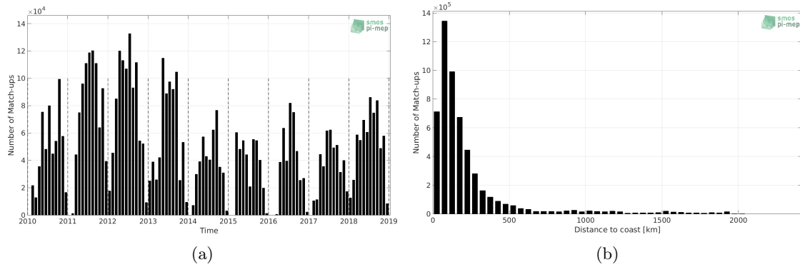
Figure 1: Number of match-ups between TSG-SAMOS and SMOS-L3-CATDS-CPDC-V3-10DAYS-25KM SSS as a function of time (a) and as function of the distance to coast (b) over the North Atlantic Ocean Pi-MEP region and for the full satellite product period.
