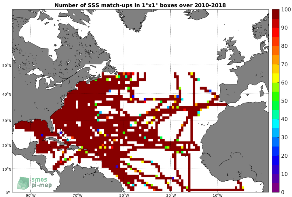
Figure 4: Number of SSS match-ups between TSG-SAMOS SSS and the SMOS-L3-CATDS-CPDC-V3-10DAYS-25KM SSS product for the North Atlantic Ocean Pi-MEP region over 1^\circ \times 1^\circ boxes and for the full satellite product period.
