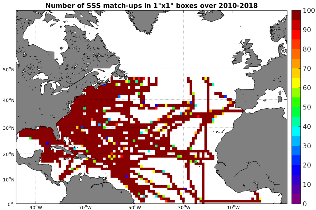
Figure 4: Number of SSS match-ups between TSG-SAMOS SSS and the SMOS-L3-CATDS-CPDC-V3-10DAYS-25KM SSS product for the North Atlantic Ocean Pi-MEP region over 1°x1° boxes and for the full satellite product period.
