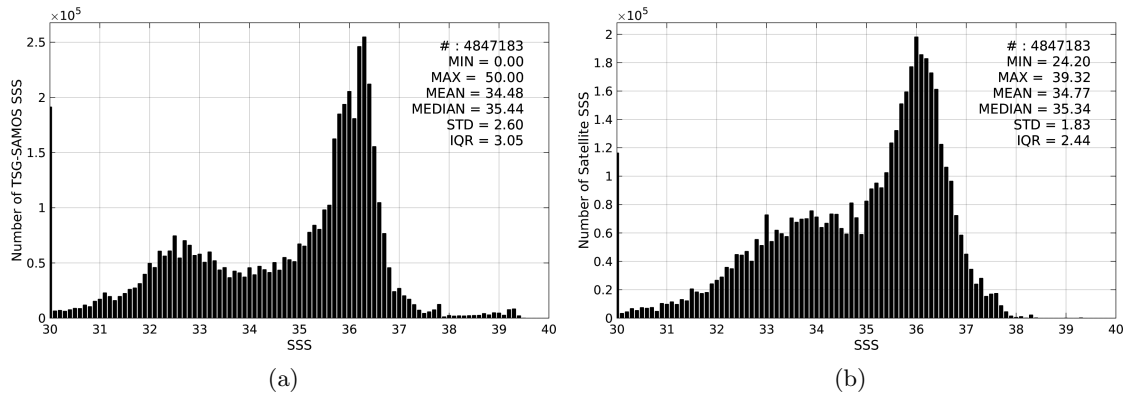
Figure 2: Histograms of SSS from TSG-SAMOS (a) and SMOS-L3-CATDS-CPDC-V3-10DAYS-25KM (b) considering all match-up pairs per bins of 0.1 over the North Atlantic Ocean Pi-MEP region and for the full satellite product period.
