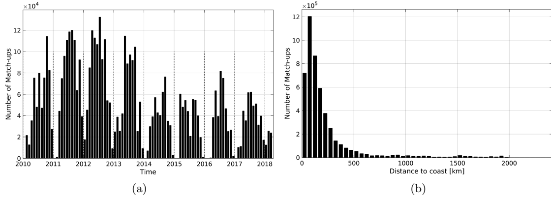
Figure 1: Number of match-ups between TSG-SAMOS and SMOS-L3-CATDS-CPDC-V3-10DAYS-25KM SSS as a function of time (a) and as function of the distance to coast (b) over the North Atlantic Ocean Pi-MEP region and for the full satellite product period.
