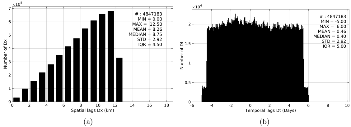
Figure 5: Histograms of the spatial (a) and temporal (b) lags between the time of the TSG-SAMOS measurements and the date of the corresponding SMOS-L3-CATDS-CPDC-V3-10DAYS-25KM SSS product.
