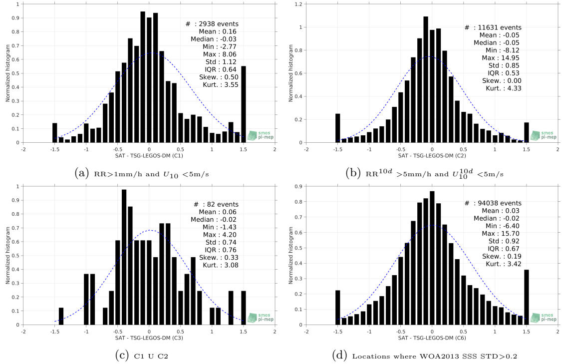
Figure 13: Normalized histogram of \Delta SSS (SMOS-L3-CATDS-CPDC-V3-10DAYS-25KM - TSG-LEGOS-DM) for 6 different subdatasets corresponding to: RR > 1\text{mm/h} and U_{10} < 5\text{m/s} (a), RR^{10d} > 5\text{mm/h} and U_{10}^{10d} < 5\text{m/s} (b), C1 U C2 (c), Locations where WOA2013 SSS STD > 0.2 (d).
