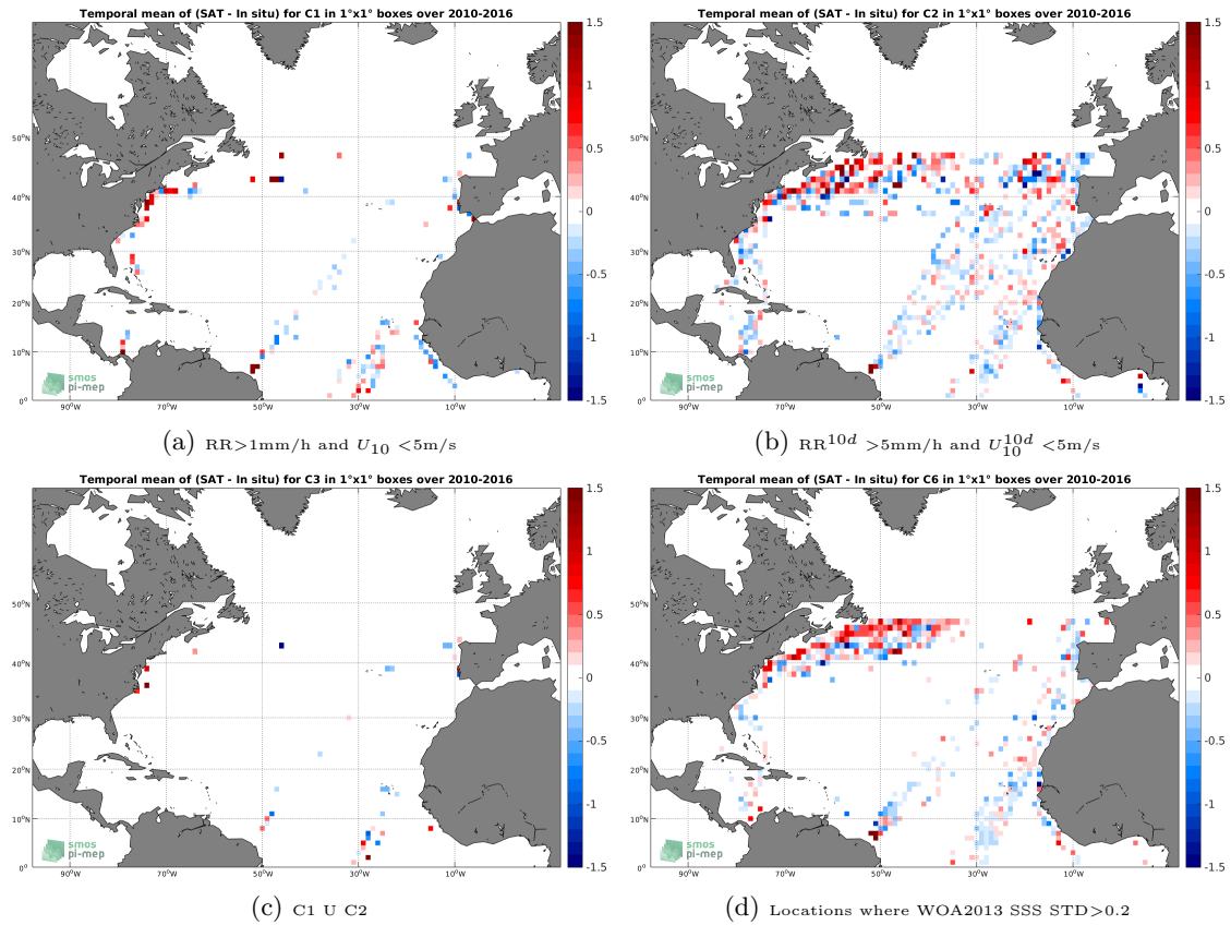
Figure 12: Temporal mean gridded over spatial boxes of size 1^\circ \times 1^\circ of \Delta SSS (SMOS-L3-CATDS-CPDC-V3-10DAYS-25KM - TSG-LEGOS-DM) for 4 different subdatasets corresponding to: RR > 1\text{mm/h} and U_{10} < 5\text{m/s} (a), RR^{10d} > 5\text{mm/h} and U_{10}^{10d} < 5\text{m/s} (b), C1 U C2 (c), Locations where WOA2013 SSS STD > 0.2 (d).
