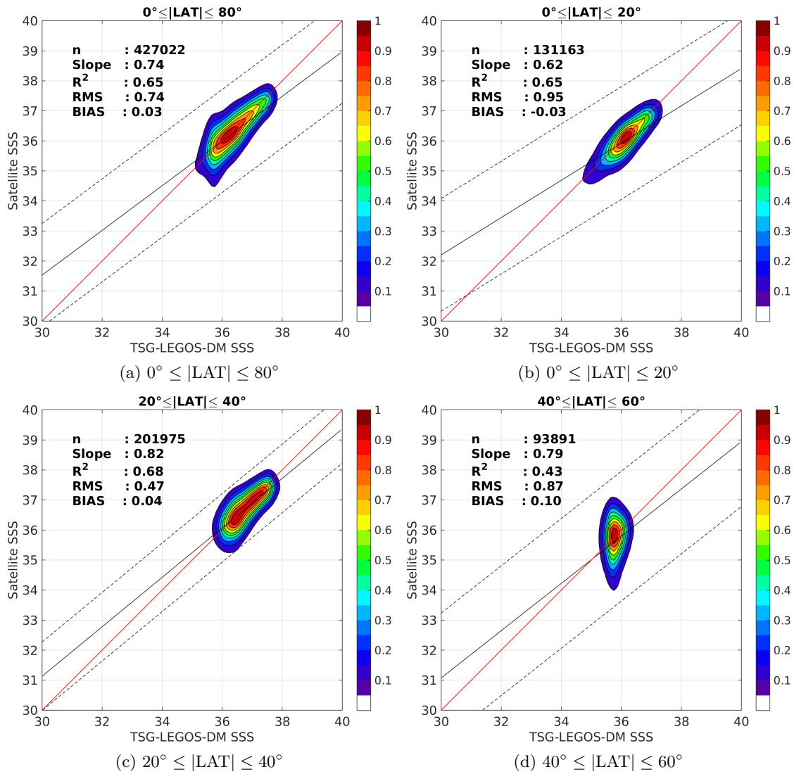
Figure 9: Contour maps of the concentration of SMOS-L3-CATDS-CPDC-V3-10DAYS-25KM SSS (y-axis) versus TSG-LEGOS-DM SSS (x-axis) at match-up pairs for different latitude bands. For each plot, the red line shows x=y . The black thin and dashed lines indicate a linear fit through the data cloud and the \pm 95\% confidence levels, respectively. The number match-up pairs n , the slope and R^2 coefficient of the linear fit, the root mean square (RMS) and the mean bias between satellite and in situ data are indicated for each latitude band in each plots.
