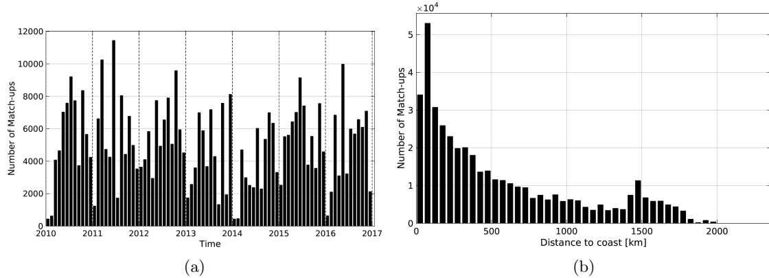
Figure 1: Number of match-ups between TSG-LEGOS-DM and SMOS-L3-CATDS-CPDC-V3-10DAYS-25KM SSS as a function of time (a) and as function of the distance to coast (b) over the North Atlantic Ocean Pi-MEP region and for the full satellite product period.
