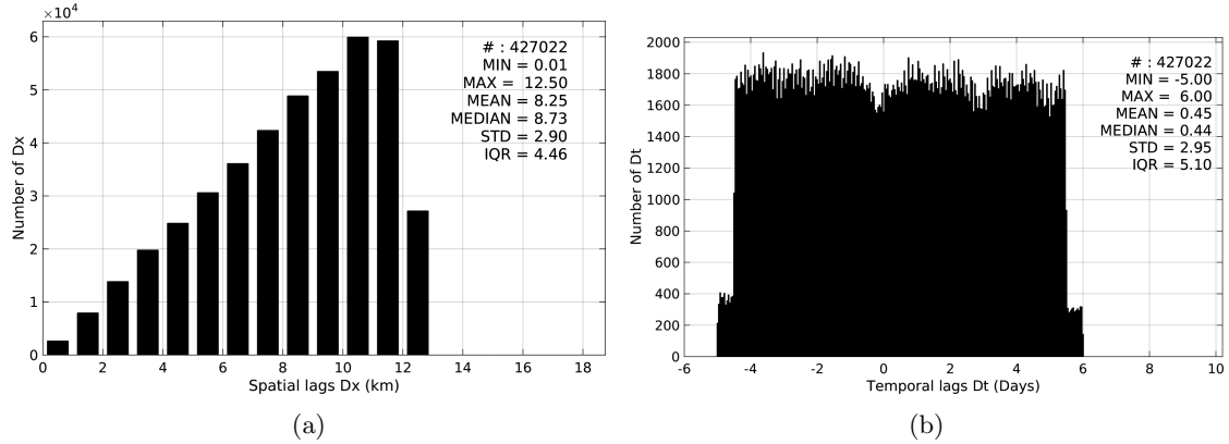
Figure 5: Histograms of the spatial (a) and temporal (b) lags between the time of the TSG-LEGOS-DM measurements and the date of the corresponding SMOS-L3-CATDS-CPDC-V3-10DAYS-25KM SSS product.
