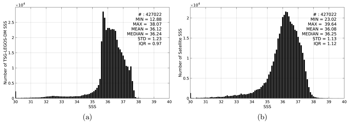
Figure 2: Histograms of SSS from TSG-LEGOS-DM (a) and SMOS-L3-CATDS-CPDC-V3-10DAYS-25KM (b) considering all match-up pairs per bins of 0.1 over the North Atlantic Ocean Pi-MEP region and for the full satellite product period.
