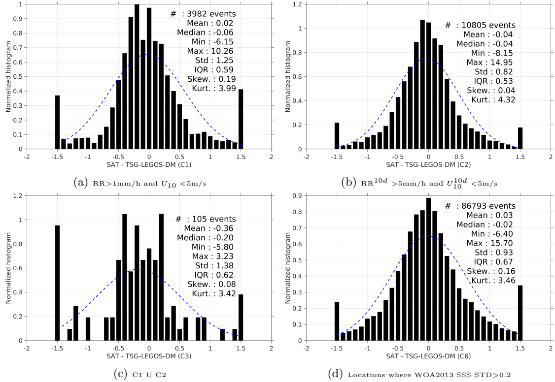
Figure 13: Normalized histogram of \Delta\text{SSS} (SMOS-L3-CATDS-CPDC-V3-10DAYS-25KM - TSG-LEGOS-DM) for 6 different subdatasets corresponding to: \text{RR} > 1\text{mm/h} and U_{10} < 5\text{m/s} (a), \text{RR}^{10d} > 5\text{mm/h} and U_{10}^{10d} < 5\text{m/s} (b), C1 U C2 (c), Locations where WOA2013 SSS STD > 0.2 (d).
