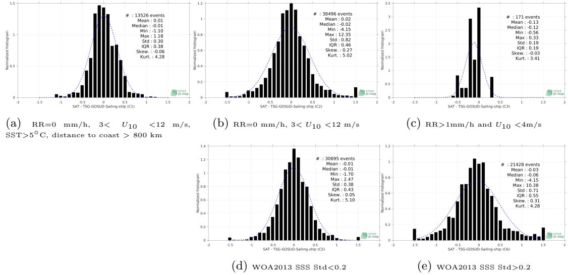
Figure 13: Normalized histogram of \Delta SSS (SMOS-L3-CATDS-CPDC-V3-10DAYS-25KM - TSG-GOSUD-Sailing-ship) for 5 different subdatasets corresponding to: RR=0 mm/h, 3 < U_{10} < 12 m/s, SST > 5°C, distance to coast > 800 km (a), RR=0 mm/h, 3 < U_{10} < 12 m/s (b), RR > 1mm/h and U_{10} < 4 m/s (c), WOA2013 SSS Std < 0.2 (d), WOA2013 SSS Std > 0.2 (e).
