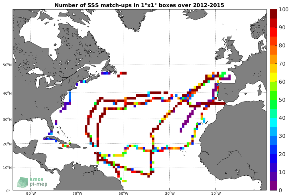
Figure 4: Number of SSS match-ups between TSG-GOSUD-Sailing-ship SSS and the SMOS-L3-CATDS-CPDC-V3-10DAYS-25KM SSS product for the North Atlantic Ocean Pi-MEP region over 1^\circ \times 1^\circ boxes and for the full satellite product period.
