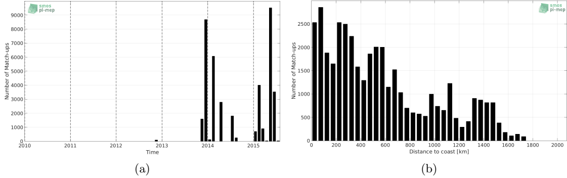
Figure 1: Number of match-ups between TSG-GOSUD-Sailing-ship and SMOS-L3-CATDS-CPDC-V3-10DAYS-25KM SSS as a function of time (a) and as function of the distance to coast (b) over the North Atlantic Ocean Pi-MEP region and for the full satellite product period.
