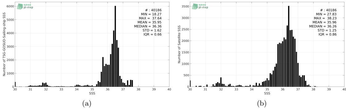
Figure 2: Histograms of SSS from TSG-GOSUD-Sailing-ship (a) and SMOS-L3-CATDS-CPDC-V3-10DAYS-25KM (b) considering all match-up pairs per bins of 0.1 over the North Atlantic Ocean Pi-MEP region and for the full satellite product period.
