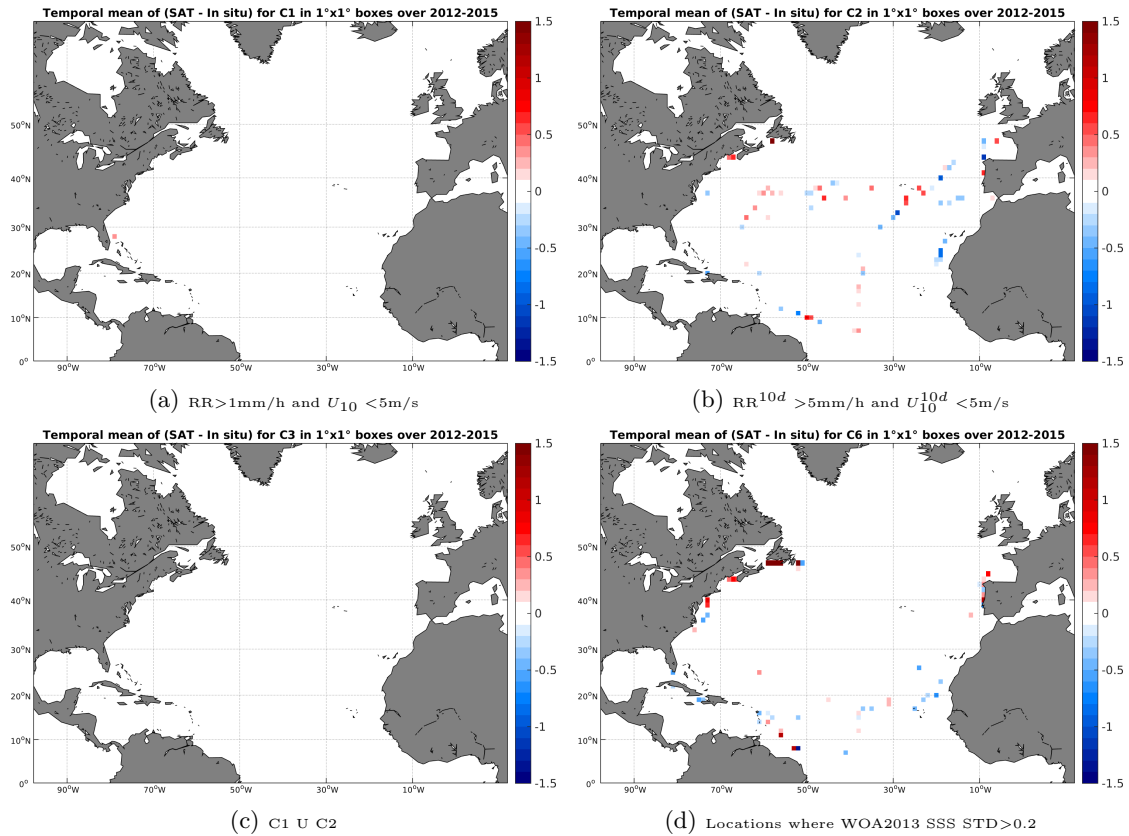
Figure 12: Temporal mean gridded over spatial boxes of size 1°x1° of \Delta SSS (SMOS-L3-CATDS-CPDC-V3-10DAYS-25KM - TSG-GOSUD-Sailing-ship) for 4 different subdatasets corresponding to:RR>1mm/h and U_{10} < 5m/s (a), RR^{10d} > 5mm/h and U_{10}^{10d} < 5m/s (b), C1 U C2 (c),Locations where WOA2013 SSS STD>0.2 (d).
