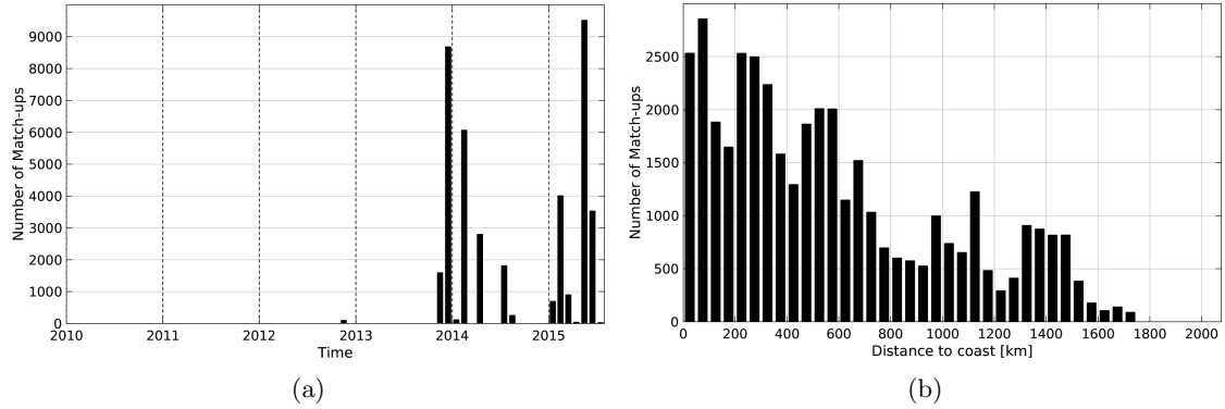
Figure 1: Number of match-ups between TSG-GOSUD-Sailing-ship and SMOS-L3-CATDS-CPDC-V3-10DAYS-25KM SSS as a function of time (a) and as function of the distance to coast (b) over the North Atlantic Ocean Pi-MEP region and for the full satellite product period.
