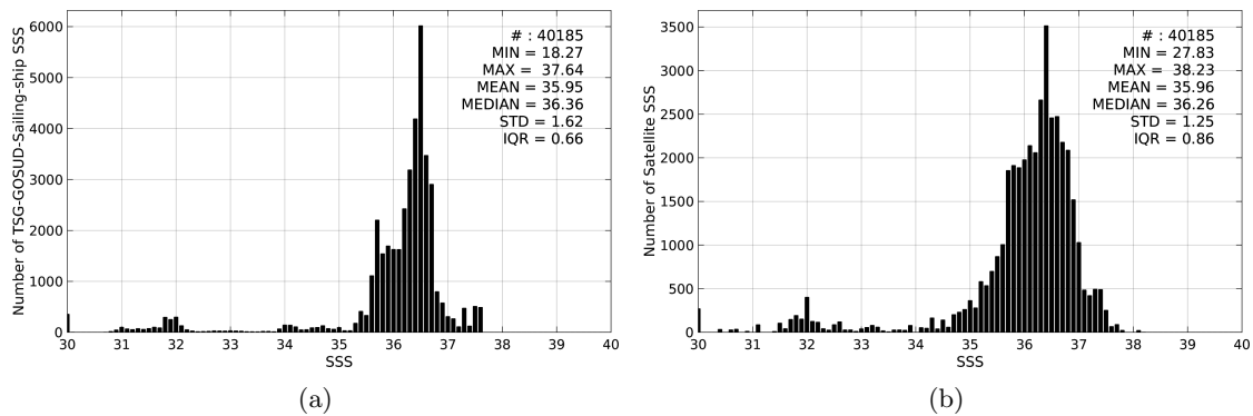
Figure 2: Histograms of SSS from TSG-GOSUD-Sailing-ship (a) and SMOS-L3-CATDS-CPDC-V3-10DAYS-25KM (b) considering all match-up pairs per bins of 0.1 over the North Atlantic Ocean Pi-MEP region and for the full satellite product period.
