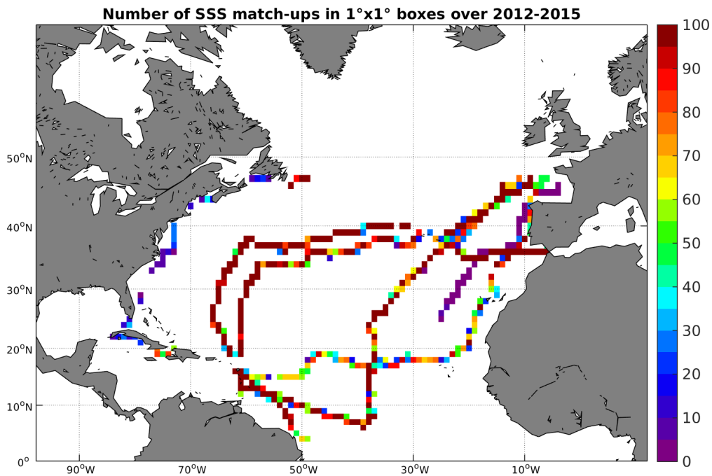
Figure 4: Number of SSS match-ups between TSG-GOSUD-Sailing-ship SSS and the SMOS-L3-CATDS-CPDC-V3-10DAYS-25KM SSS product for the North Atlantic Ocean Pi-MEP region over 1°x1° boxes and for the full satellite product period.
