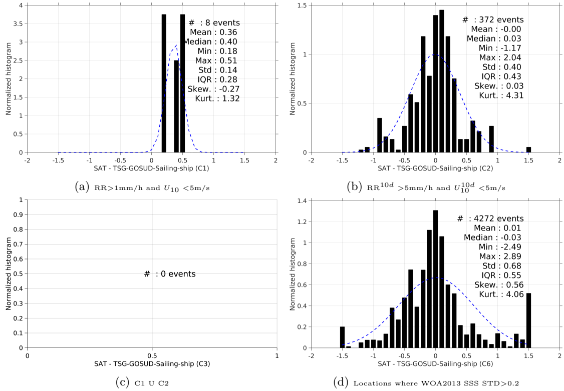
Figure 13: Normalized histogram of \Delta\text{SSS} (SMOS-L3-CATDS-CPDC-V3-10DAYS-25KM - TSG-GOSUD-Sailing-ship) for 6 different subdatasets corresponding to: RR > 1mm/h and U_{10} < 5\text{m/s} (a), RR^{10d} > 5\text{mm/h} and U_{10}^{10d} < 5\text{m/s} (b), C1 U C2 (c), Locations where WOA2013 SSS STD > 0.2 (d).
