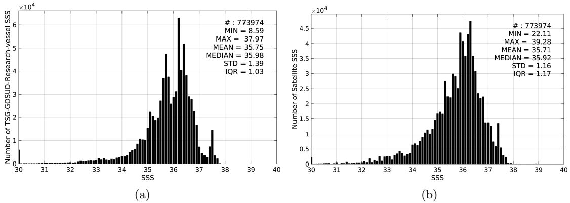
Figure 2: Histograms of SSS from TSG-GOSUD-Research-vessel (a) and SMOS-L3-CATDS-CPDC-V3-10DAYS-25KM (b) considering all match-up pairs per bins of 0.1 over the North Atlantic Ocean Pi-MEP region and for the full satellite product period.
