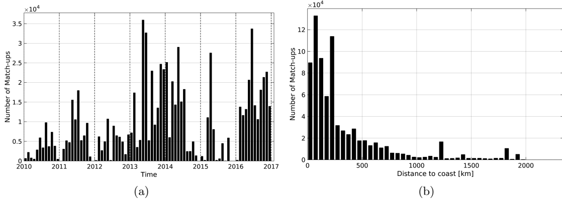
Figure 1: Number of match-ups between TSG-GOSUD-Research-vessel and SMOS-L3-CATDS-CPDC-V3-10DAYS-25KM SSS as a function of time (a) and as function of the distance to coast (b) over the North Atlantic Ocean Pi-MEP region and for the full satellite product period.
