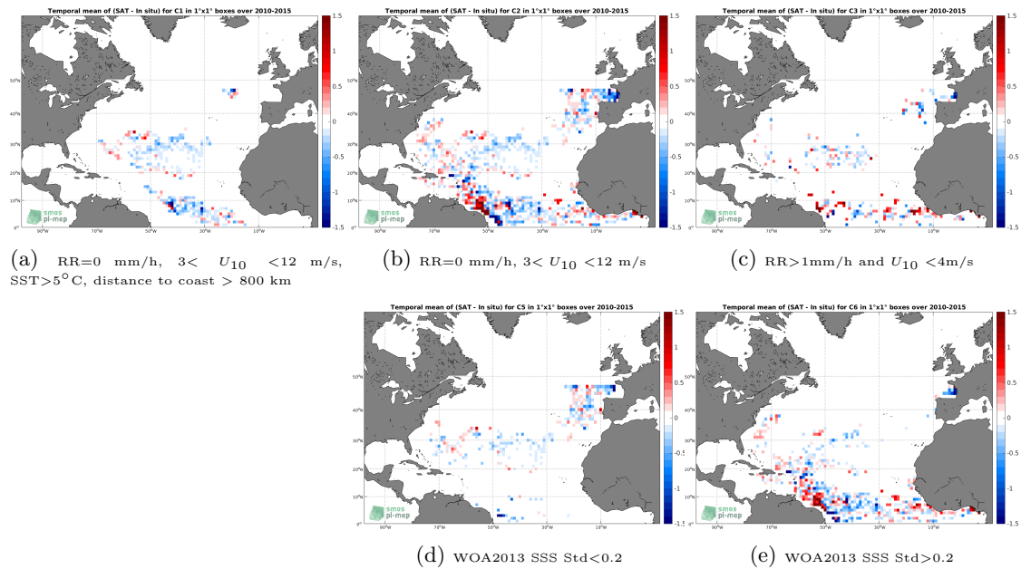
Figure 11: Temporal mean gridded over spatial boxes of size 1^\circ \times 1^\circ of \Delta SSS (SMOS-L3-CATDS-CPDC-V3-10DAYS-25KM - Surface drifters) for 5 different subdatasets corresponding to:RR=0 mm/h, 3 < U_{10} < 12 m/s, SST > 5^\circ\text{C} , distance to coast > 800 km (a), RR=0 mm/h, 3 < U_{10} < 12 m/s (b), RR > 1 mm/h and U_{10} < 4 m/s (c), WOA2013 SSS Std < 0.2 (d), WOA2013 SSS Std > 0.2 (e).
