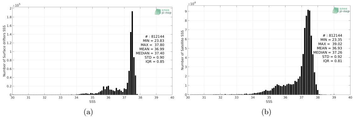
Figure 2: Histograms of SSS from Surface drifters (a) and SMOS-L3-CATDS-CPDC-V3-10DAYS-25KM (b) considering all match-up pairs per bins of 0.1 over the North Atlantic Ocean Pi-MEP region and for the full satellite product period.
