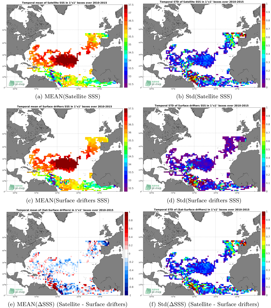
Figure 5: Temporal mean (left) and Std (right) of SSS from SMOS-L3-CATDS-CPDC-V3-10DAYS-25KM (top), Surface drifters (middle), and of \Delta SSS (Satellite - Surface drifters). Only match-up pairs are used to generate these maps.
