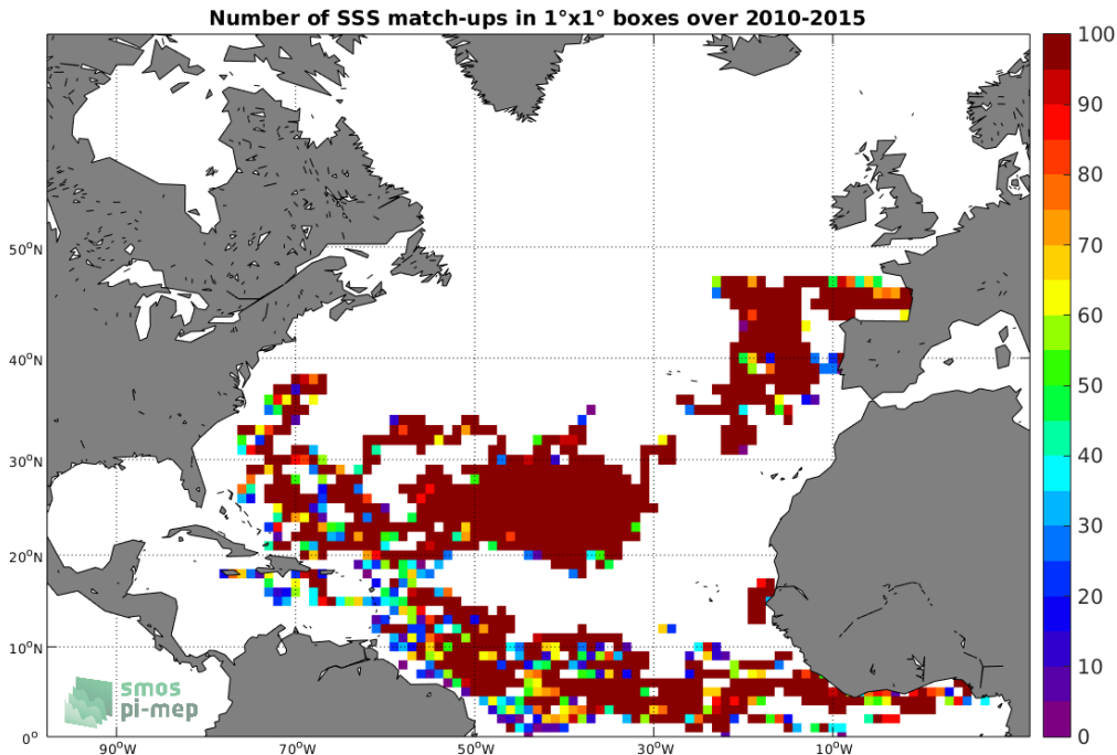
Figure 3: Number of SSS match-ups between Surface drifters SSS and the SMOS-L3-CATDS-CPDC-V3-10DAYS-25KM SSS product for the North Atlantic Ocean Pi-MEP region over 1°x1° boxes and for the full satellite product period.
