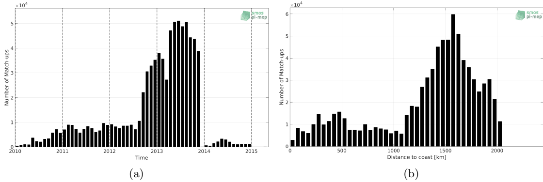
Figure 1: Number of match-ups between Surface drifters and SMOS-L3-CATDS-CPDC-V3-10DAYS-25KM SSS as a function of time (a) and as function of the distance to coast (b) over the North Atlantic Ocean Pi-MEP region and for the full satellite product period.
