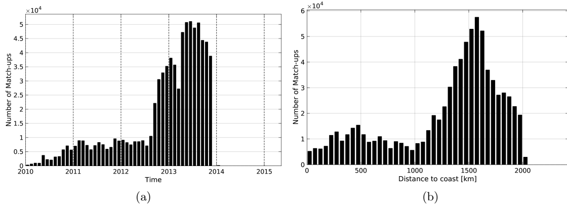
Figure 1: Number of match-ups between Surface drifters and SMOS-L3-CATDS-CPDC-V3-10DAYS-25KM SSS as a function of time (a) and as function of the distance to coast (b) over the North Atlantic Ocean Pi-MEP region and for the full satellite product period.
