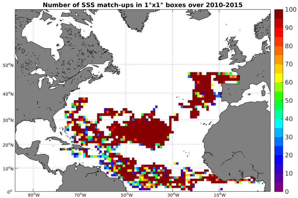
Figure 3: Number of SSS match-ups between Surface drifters SSS and the SMOS-L3-CATDS-CPDC-V3-10DAYS-25KM SSS product for the North Atlantic Ocean Pi-MEP region over 1^\circ \times 1^\circ boxes and for the full satellite product period.
