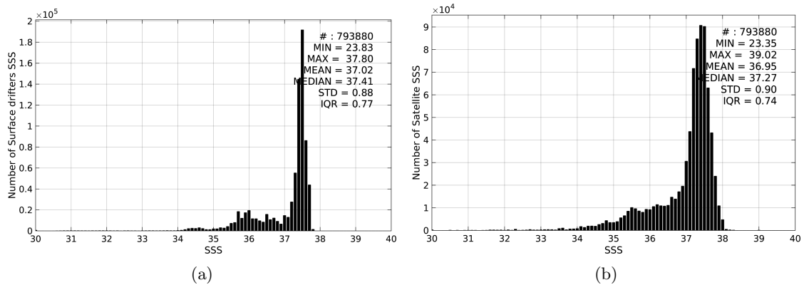
Figure 2: Histograms of SSS from Surface drifters (a) and SMOS-L3-CATDS-CPDC-V3-10DAYS-25KM (b) considering all match-up pairs per bins of 0.1 over the North Atlantic Ocean Pi-MEP region and for the full satellite product period.
