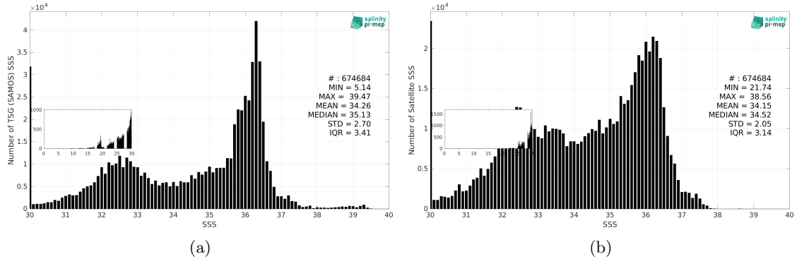
Figure 3: Histograms of SSS from TSG (SAMOS) (a) and SMOS SSS L3 v2 - 9-Days (BEC) (b) considering all match-up pairs per bins of 0.1 over the North Atlantic Ocean Pi-MEP region and for the full satellite product period.
