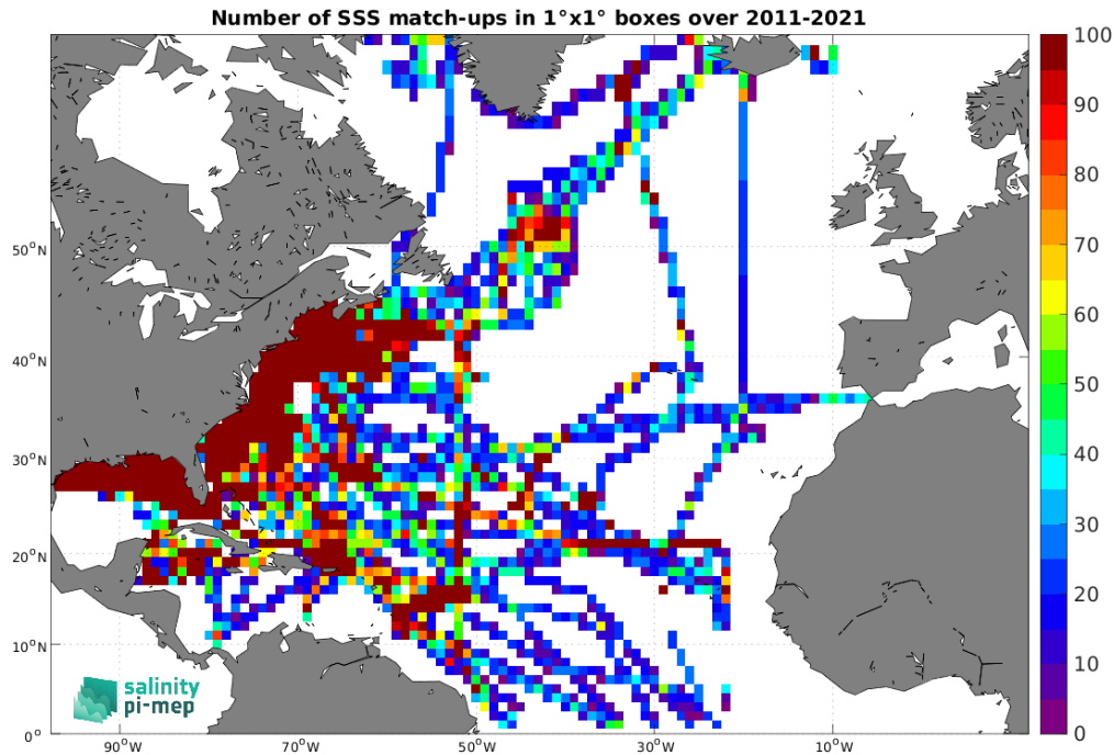
Figure 5: Number of SSS match-ups between TSG (SAMOS) SSS and the SMOS SSS L3 v2 - 9-Days (BEC) SSS product for the North Atlantic Ocean Pi-MEP region over 1^\circ \times 1^\circ boxes and for the full satellite product period.
