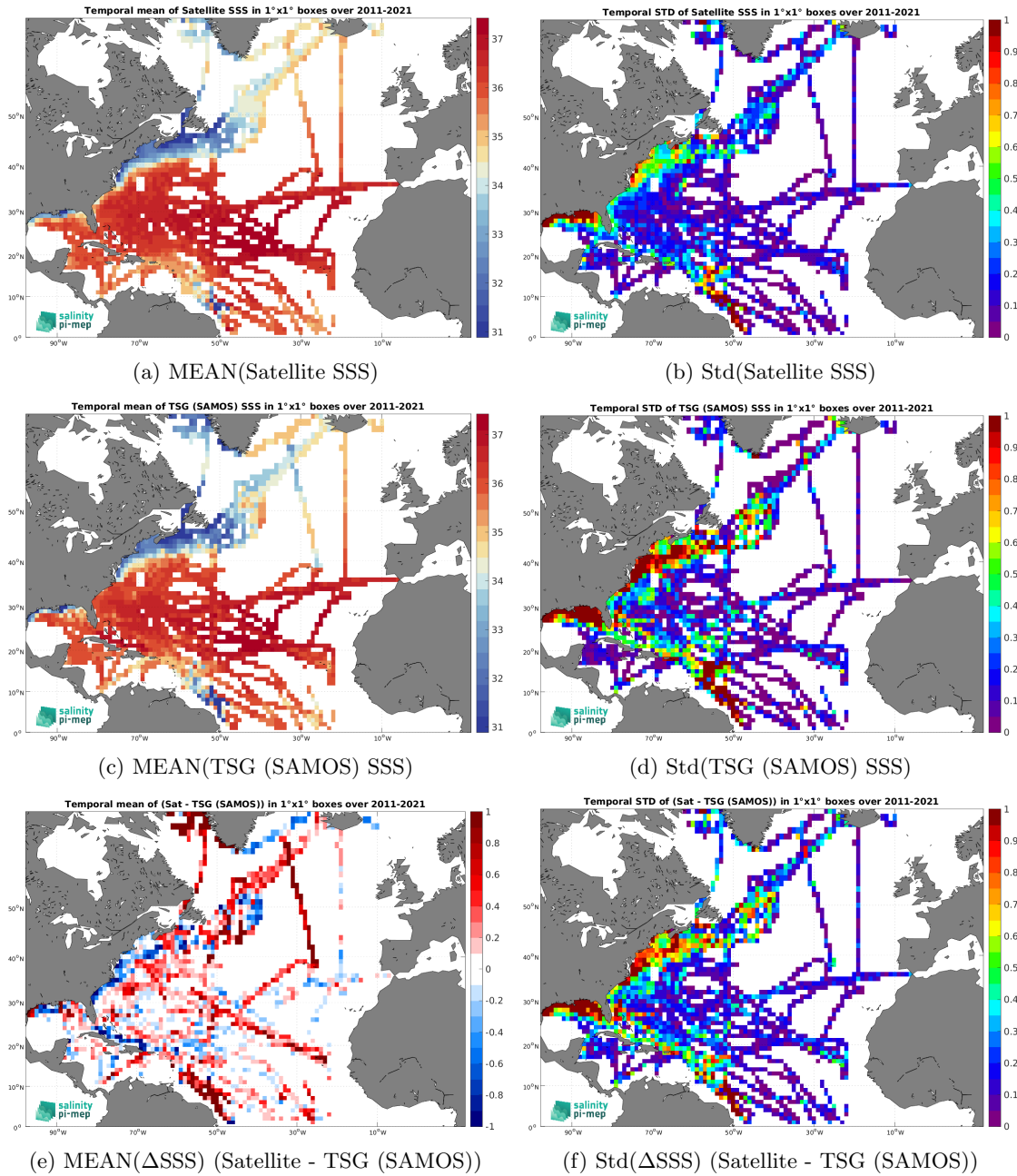
Figure 7: Temporal mean (left) and Std (right) of SSS from SMOS SSS L3 v2 - 9-Days (BEC) (top), TSG (SAMOS) (middle), and of \Delta SSS (Satellite - TSG (SAMOS)). Only match-up pairs are used to generate these maps.
