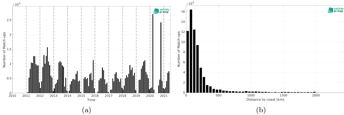
Figure 2: Number of match-ups between TSG (SAMOS) and SMOS SSS L3 v2 - 9-Days (BEC) SSS as a function of time (a) and as function of the distance to coast (b) over the North Atlantic Ocean Pi-MEP region and for the full satellite product period.
