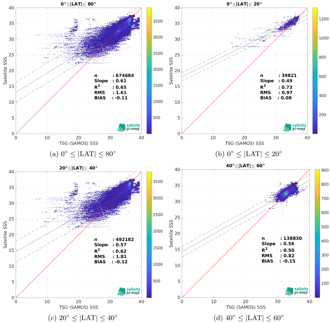
Figure 10: Contour maps of the concentration of SMOS SSS L3 v2 - 9-Days (BEC) SSS (y-axis) versus TSG (SAMOS) SSS (x-axis) at match-up pairs for different latitude bands. For each plot, the red line shows x=y . The black thin and dashed lines indicate a linear fit through the data cloud and the \pm 95\% confidence levels, respectively. The number match-up pairs n , the slope and R^2 coefficient of the linear fit, the root mean square (RMS) and the mean bias between satellite and in situ data are indicated for each latitude band in each plots.
