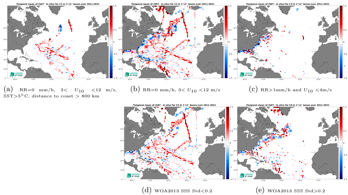
Figure 14: Temporal mean gridded over spatial boxes of size 1^\circ \times 1^\circ of \Delta\text{SSS} (SMOS SSS L3 v2 - 9-Days (BEC) - TSG (SAMOS)) for 5 different subdatasets corresponding to:RR=0 mm/h, 3 < U_{10} < 12 m/s, SST >5^\circ\text{C} , distance to coast > 800 km (a), RR=0 mm/h, 3 < U_{10} < 12 m/s (b), RR >1 mm/h and U_{10} < 4 m/s (c), WOA2013 SSS Std <0.2 (d), WOA2013 SSS Std >0.2 (e).
