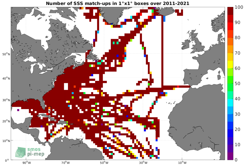
Figure 4: Number of SSS match-ups between TSG (SAMOS) SSS and the SMOS SSS L3 v2 - 9-Days (BEC) SSS product for the North Atlantic Ocean Pi-MEP region over 1^\circ \times 1^\circ boxes and for the full satellite product period.
