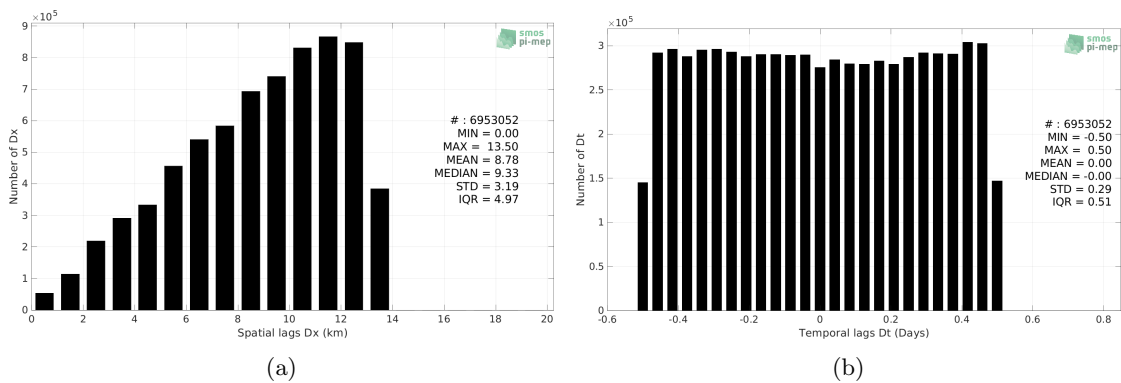
Figure 5: Histograms of the spatial (a) and temporal (b) lags between the location/time of the TSG (SAMOS) measurement and the date of the corresponding SMOS SSS L3 v2 - 9-Days (BEC) SSS pixel.
