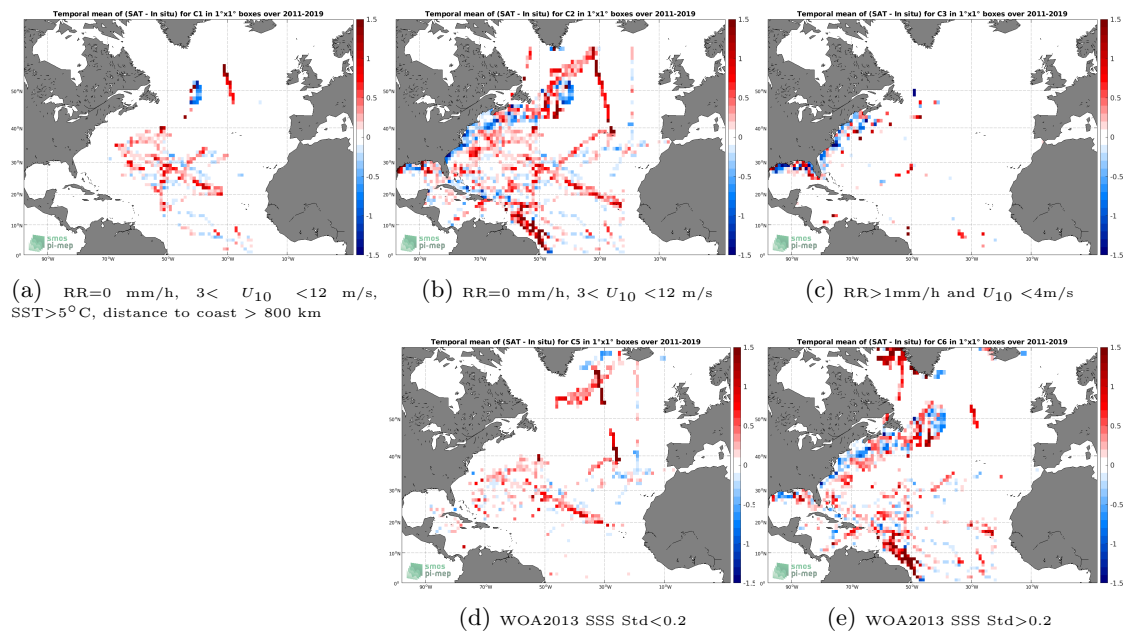
Figure 12: Temporal mean gridded over spatial boxes of size 1°x1° of \Delta SSS (SMOS SSS L3 v2 - 9-Days (BEC) - TSG (SAMOS)) for 5 different subdatasets corresponding to:RR=0 mm/h, 3 < U_{10} < 12 m/s, SST>5°C, distance to coast > 800 km (a), RR=0 mm/h, 3 < U_{10} < 12 m/s (b), RR>1mm/h and U_{10} < 4 m/s (c), WOA2013 SSS Std<0.2 (d), WOA2013 SSS Std>0.2 (e).
