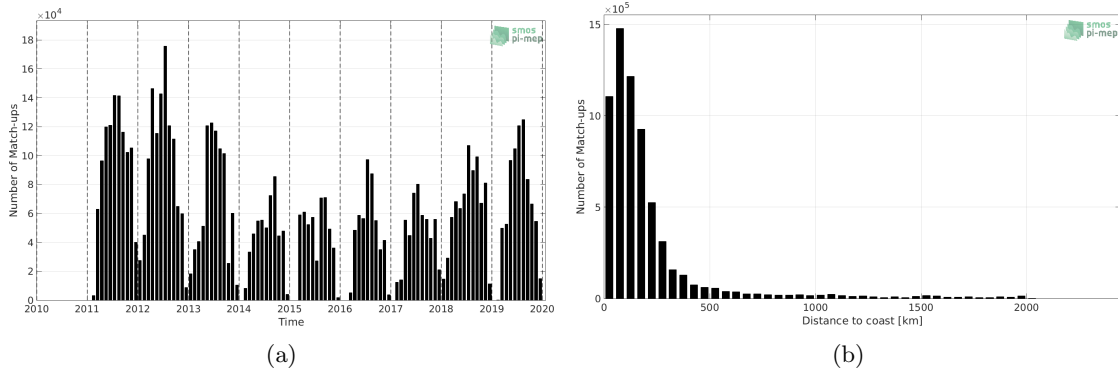
Figure 1: Number of match-ups between TSG (SAMOS) and SMOS L3 v2 - 9-Days (BEC) SSS as a function of time (a) and as function of the distance to coast (b) over the North Atlantic Ocean Pi-MEP region and for the full satellite product period.
