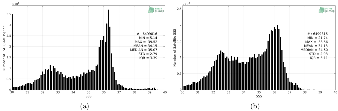
Figure 2: Histograms of SSS from TSG (SAMOS) (a) and SMOS L3 v2 - 9-Days (BEC) (b) considering all match-up pairs per bins of 0.1 over the North Atlantic Ocean Pi-MEP region and for the full satellite product period.
