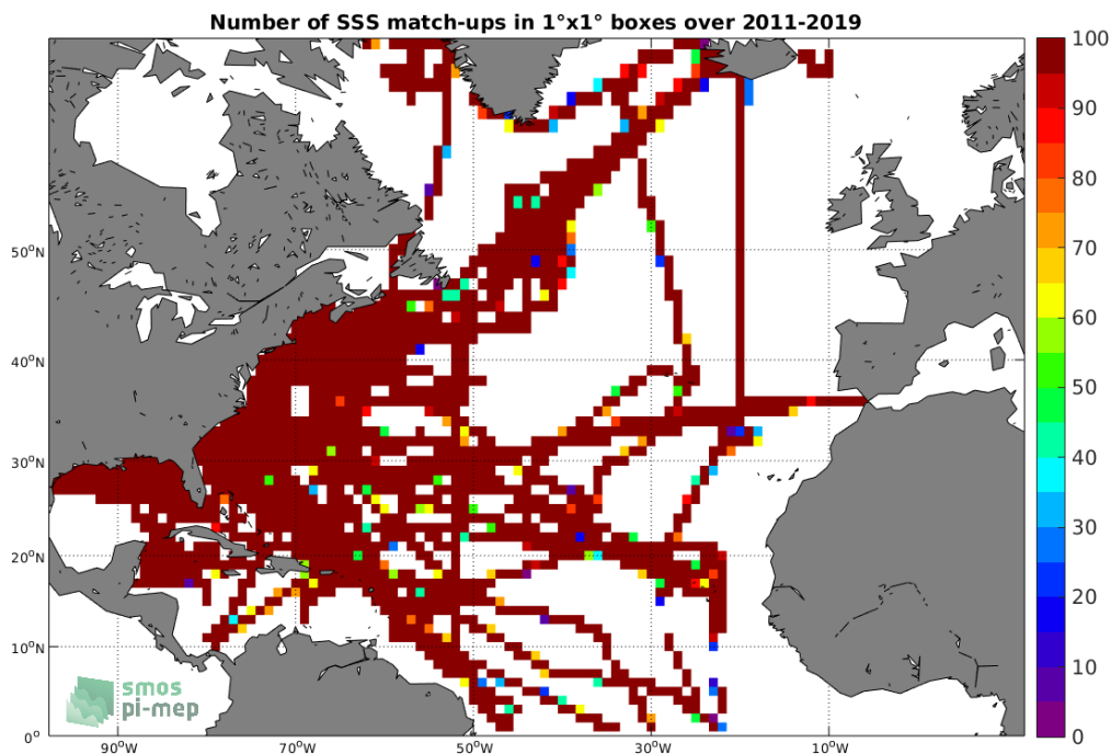
Figure 4: Number of SSS match-ups between TSG (SAMOS) SSS and the SMOS L3 v2 - 9-Days (BEC) SSS product for the North Atlantic Ocean Pi-MEP region over 1^\circ \times 1^\circ boxes and for the full satellite product period.
