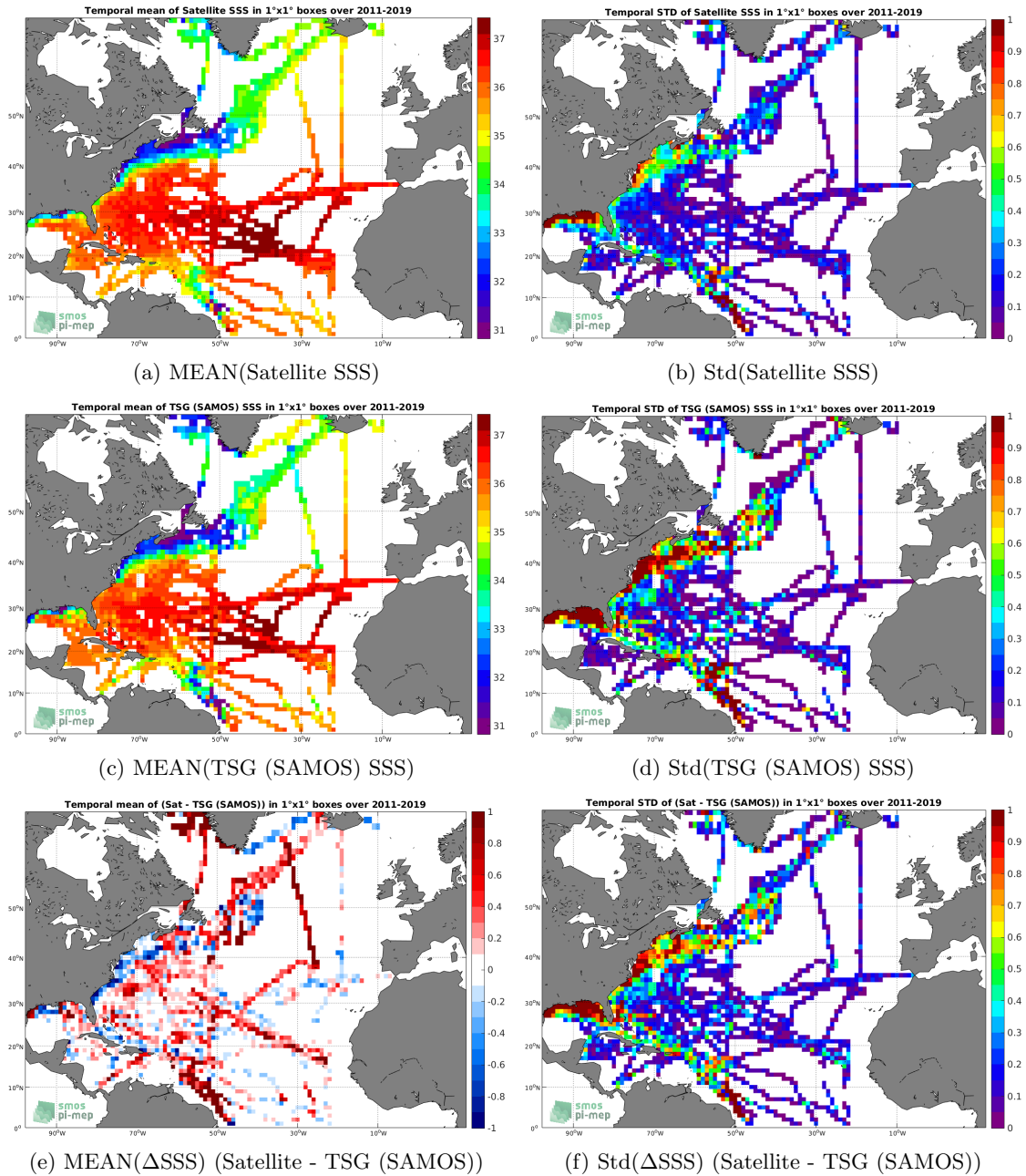
Figure 6: Temporal mean (left) and Std (right) of SSS from SMOS L3 v2 - 9-Days (BEC) (top), TSG (SAMOS) (middle), and of \Delta SSS (Satellite - TSG (SAMOS)). Only match-up pairs are used to generate these maps.
