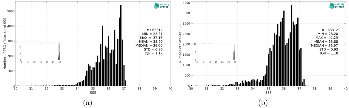
Figure 3: Histograms of SSS from TSG (Polarstern) (a) and SMOS SSS L3 v2 - 9-Days (BEC) (b) considering all match-up pairs per bins of 0.1 over the North Atlantic Ocean Pi-MEP region and for the full satellite product period.
