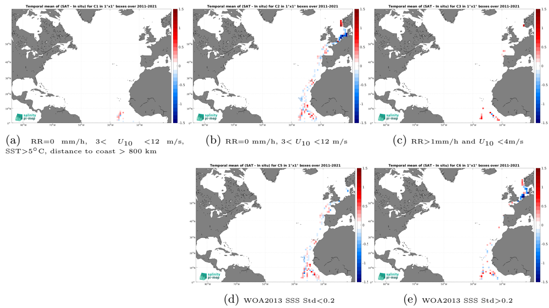
Figure 14: Temporal mean gridded over spatial boxes of size 1^\circ \times 1^\circ of \Delta\text{SSS} (SMOS SSS L3 v2 - 9-Days (BEC) - TSG (Polarstern)) for 5 different subdatasets corresponding to:RR=0 mm/h, 3 < U_{10} < 12 m/s, SST >5^\circ\text{C} , distance to coast > 800 km (a), RR=0 mm/h, 3 < U_{10} < 12 m/s (b), RR >1 mm/h and U_{10} < 4 m/s (c), WOA2013 SSS Std <0.2 (d), WOA2013 SSS Std >0.2 (e).
