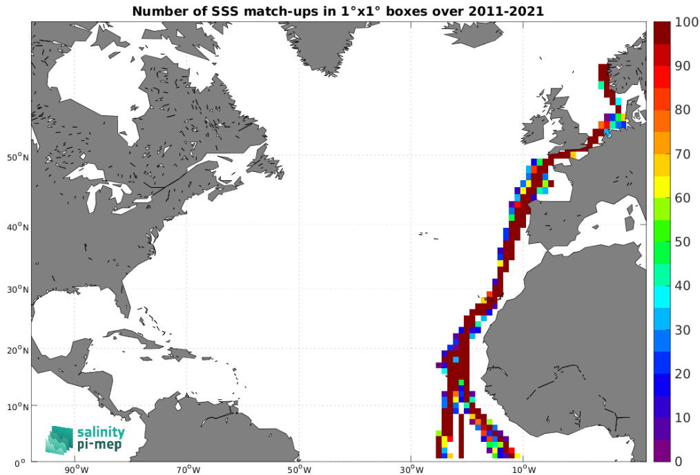
Figure 5: Number of SSS match-ups between TSG (Polarstern) SSS and the SMOS SSS L3 v2 - 9-Days (BEC) SSS product for the North Atlantic Ocean Pi-MEP region over 1^\circ \times 1^\circ boxes and for the full satellite product period.
