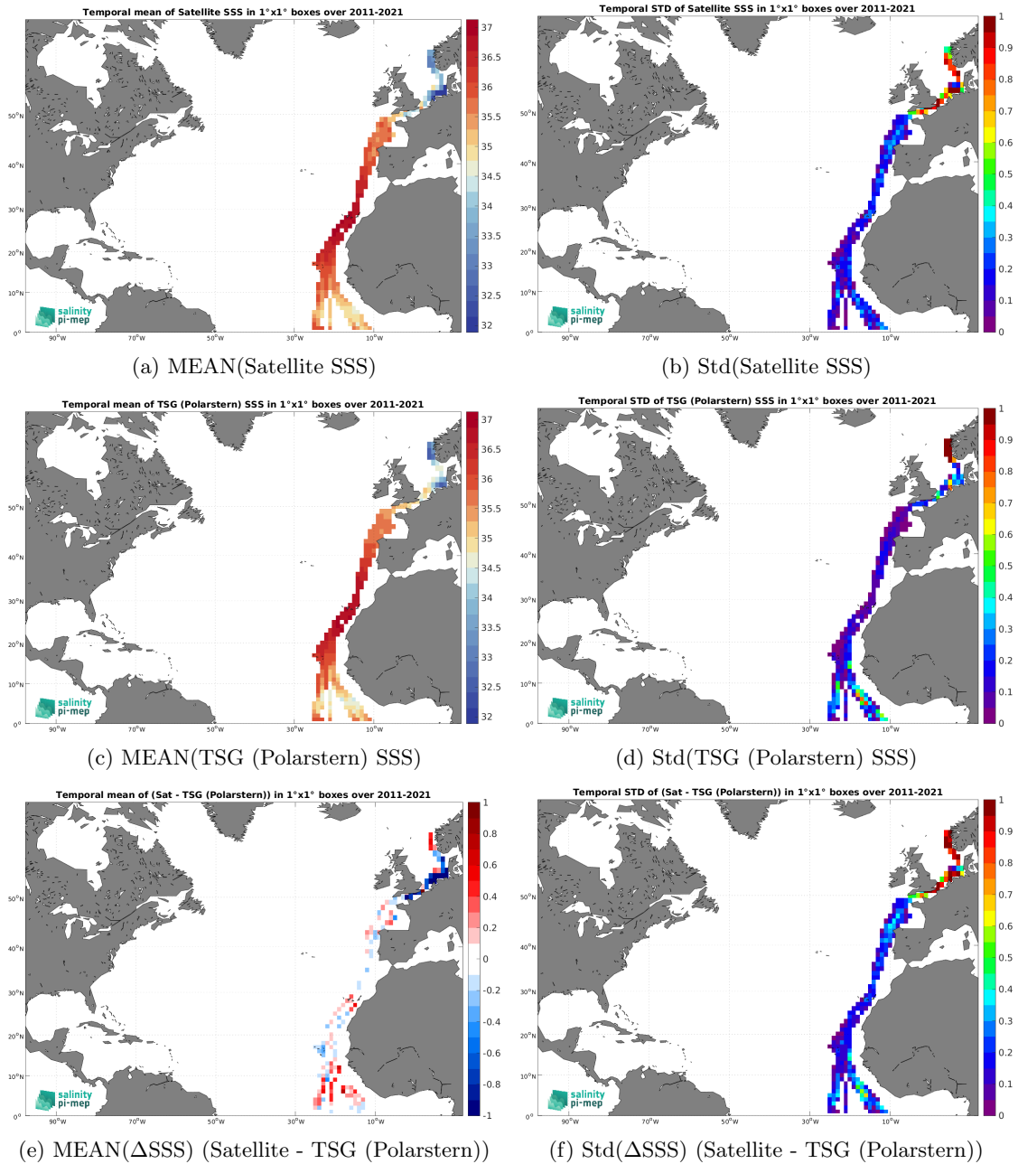
Figure 7: Temporal mean (left) and Std (right) of SSS from SMOS SSS L3 v2 - 9-Days (BEC) (top), TSG (Polarstern) (middle), and of \Delta SSS (Satellite - TSG (Polarstern)). Only match-up pairs are used to generate these maps.
