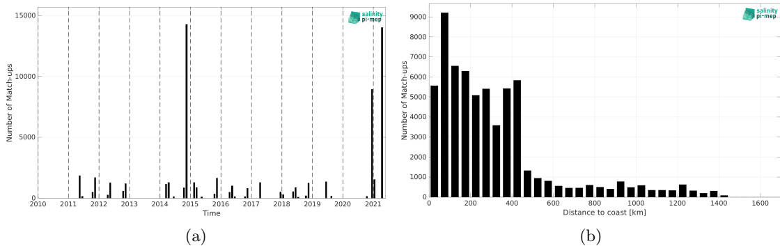
Figure 2: Number of match-ups between TSG (Polarstern) and SMOS SSS L3 v2 - 9-Days (BEC) SSS as a function of time (a) and as function of the distance to coast (b) over the North Atlantic Ocean Pi-MEP region and for the full satellite product period.
