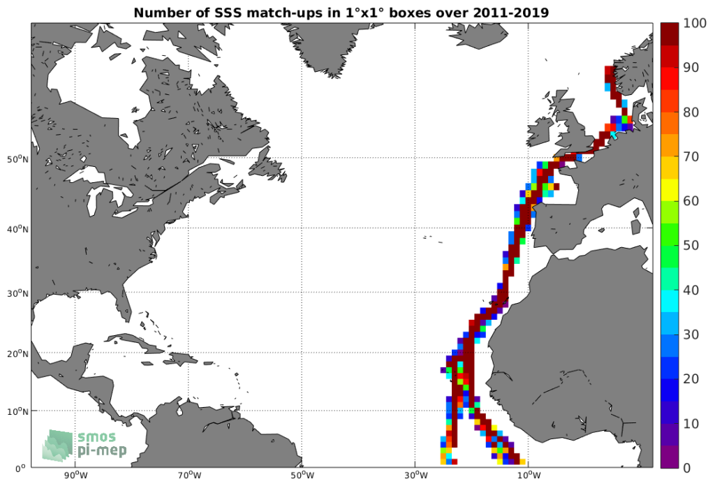
Figure 4: Number of SSS match-ups between TSG (Polarstern) SSS and the SMOS L3 v2 - 9-Days (BEC) SSS product for the North Atlantic Ocean Pi-MEP region over 1°x1° boxes and for the full satellite product period.
