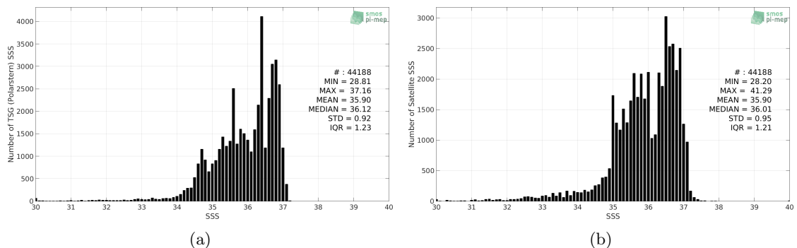
Figure 2: Histograms of SSS from TSG (Polarstern) (a) and SMOS L3 v2 - 9-Days (BEC) (b) considering all match-up pairs per bins of 0.1 over the North Atlantic Ocean Pi-MEP region and for the full satellite product period.
