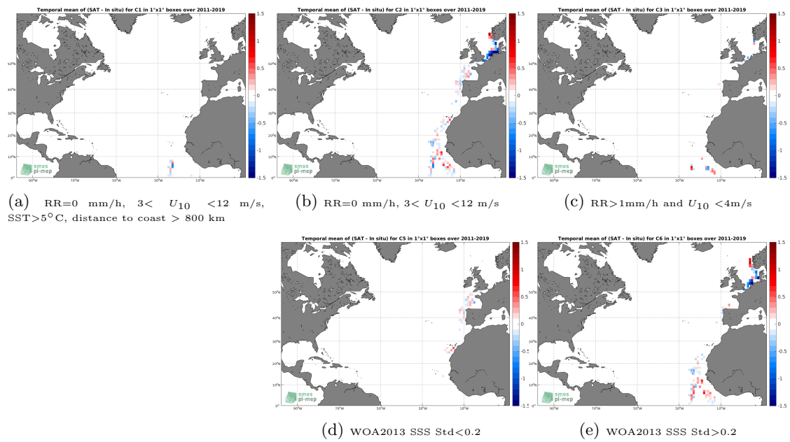
Figure 12: Temporal mean gridded over spatial boxes of size 1^\circ \times 1^\circ of \Delta SSS (SMOS L3 v2 - 9-Days (BEC) - TSG (Polarstern)) for 5 different subdatasets corresponding to:RR=0 mm/h, 3 < U_{10} < 12 m/s, SST >5^\circ\text{C} , distance to coast > 800 km (a), RR=0 mm/h, 3 < U_{10} < 12 m/s (b), RR >1 mm/h and U_{10} < 4 m/s (c), WOA2013 SSS Std <0.2 (d), WOA2013 SSS Std >0.2 (e).
