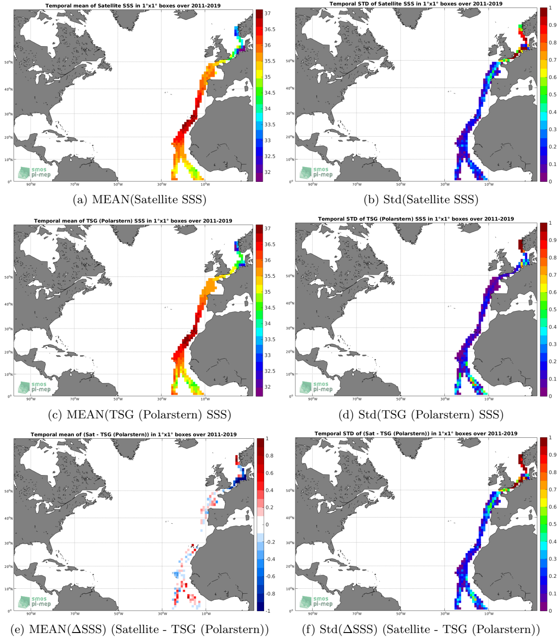
Figure 6: Temporal mean (left) and Std (right) of SSS from SMOS L3 v2 - 9-Days (BEC) (top), TSG (Polarstern) (middle), and of \Delta SSS (Satellite - TSG (Polarstern)). Only match-up pairs are used to generate these maps.
