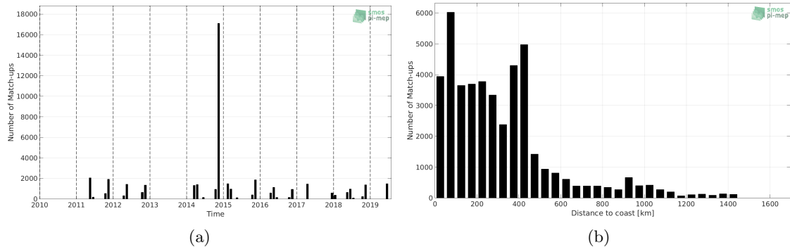
Figure 1: Number of match-ups between TSG (Polarstern) and SMOS L3 v2 - 9-Days (BEC) SSS as a function of time (a) and as function of the distance to coast (b) over the North Atlantic Ocean Pi-MEP region and for the full satellite product period.
