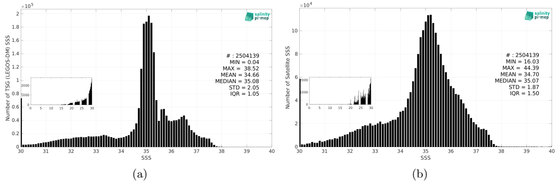
Figure 3: Histograms of SSS from TSG (LEGOS-DM) (a) and SMOS SSS L3 v2 - 9-Days (BEC) (b) considering all match-up pairs per bins of 0.1 over the North Atlantic Ocean Pi-MEP region and for the full satellite product period.
