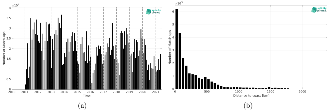
Figure 2: Number of match-ups between TSG (LEGOS-DM) and SMOS SSS L3 v2 - 9-Days (BEC) SSS as a function of time (a) and as function of the distance to coast (b) over the North Atlantic Ocean Pi-MEP region and for the full satellite product period.
