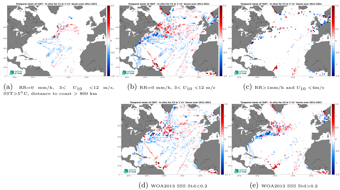
Figure 14: Temporal mean gridded over spatial boxes of size 1^\circ \times 1^\circ of \Delta\text{SSS} (SMOS SSS L3 v2 - 9-Days (BEC) - TSG (LEGOS-DM)) for 5 different subdatasets corresponding to:RR=0 mm/h, 3 < U_{10} < 12 m/s, SST > 5°C, distance to coast > 800 km (a), RR=0 mm/h, 3 < U_{10} < 12 m/s (b), RR > 1mm/h and U_{10} < 4 m/s (c), WOA2013 SSS Std < 0.2 (d), WOA2013 SSS Std > 0.2 (e).
