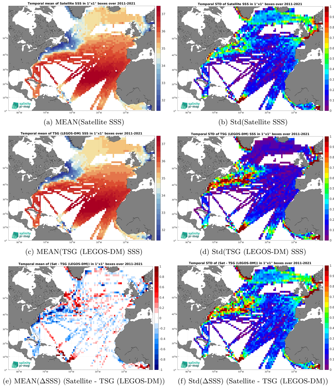
Figure 7: Temporal mean (left) and Std (right) of SSS from SMOS SSS L3 v2 - 9-Days (BEC) (top), TSG (LEGOS-DM) (middle), and of \Delta SSS (Satellite - TSG (LEGOS-DM)). Only match-up pairs are used to generate these maps.
