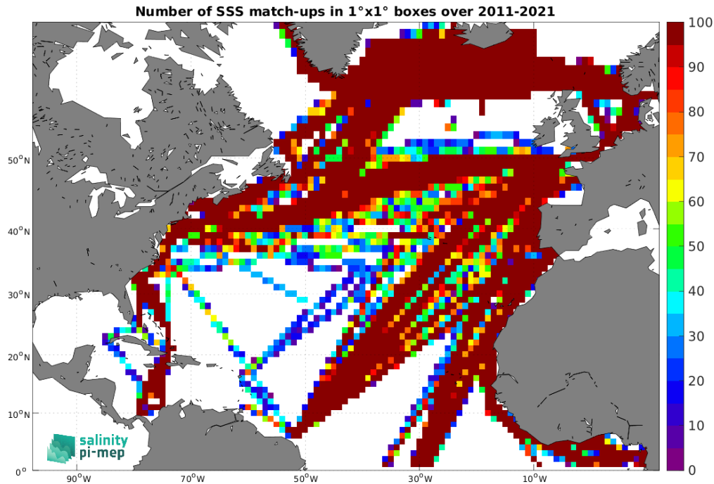
Figure 5: Number of SSS match-ups between TSG (LEGOS-DM) SSS and the SMOS SSS L3 v2 - 9-Days (BEC) SSS product for the North Atlantic Ocean Pi-MEP region over 1^\circ \times 1^\circ boxes and for the full satellite product period.
