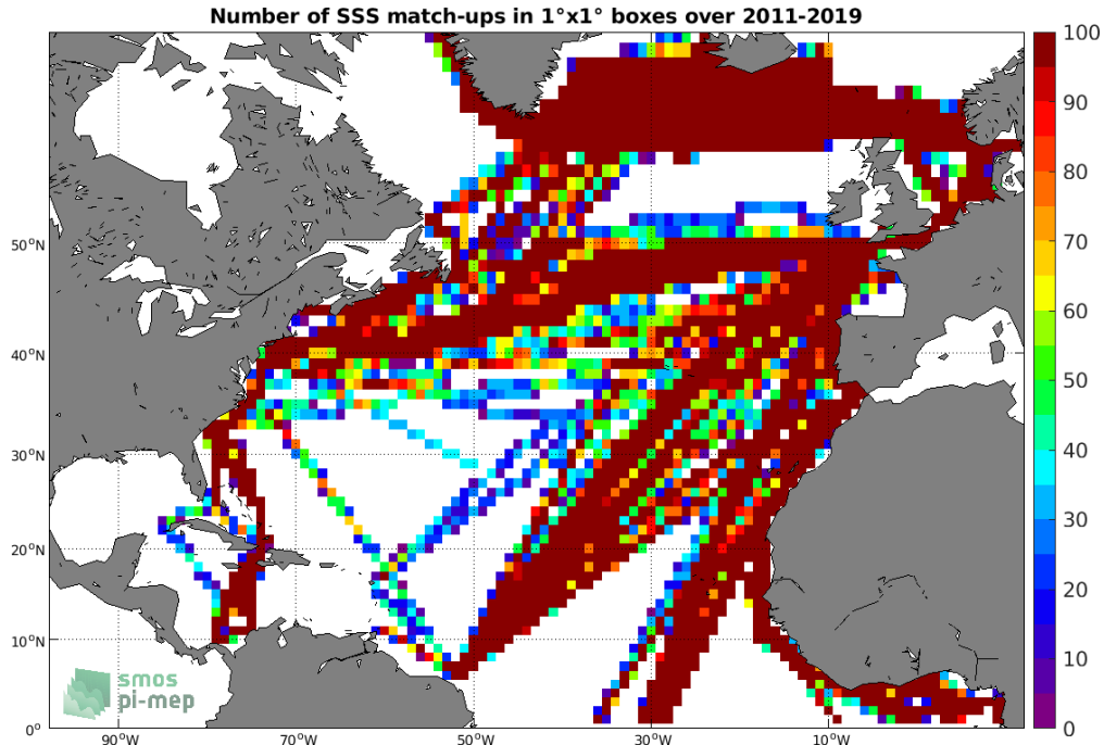
Figure 4: Number of SSS match-ups between TSG (LEGOS-DM) SSS and the SMOS SSS L3 v2 - 9-Days (BEC) SSS product for the North Atlantic Ocean Pi-MEP region over 1^{\circ} \times 1^{\circ} boxes and for the full satellite product period.
