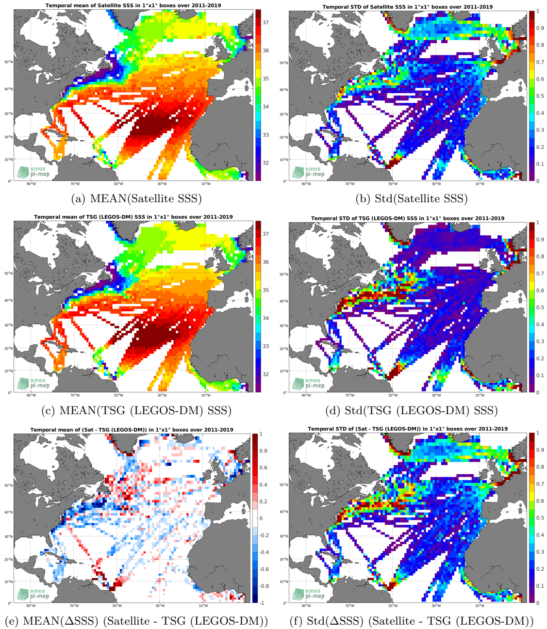
Figure 6: Temporal mean (left) and Std (right) of SSS from SMOS SSS L3 v2 - 9-Days (BEC) (top), TSG (LEGOS-DM) (middle), and of \Delta SSS (Satellite - TSG (LEGOS-DM)). Only match-pairs are used to generate these maps.
