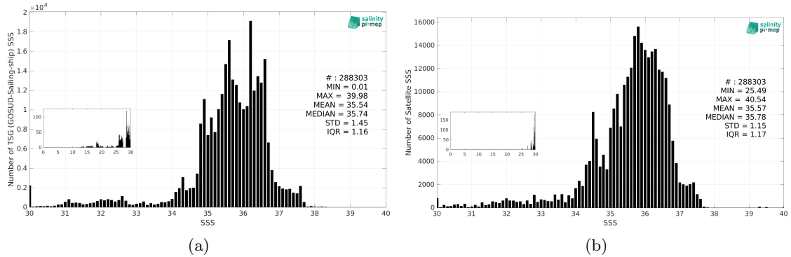
Figure 3: Histograms of SSS from TSG (GOSUD-Sailing-ship) (a) and SMOS SSS L3 v2 - 9-Days (BEC) (b) considering all match-up pairs per bins of 0.1 over the North Atlantic Ocean Pi-MEP region and for the full satellite product period.
