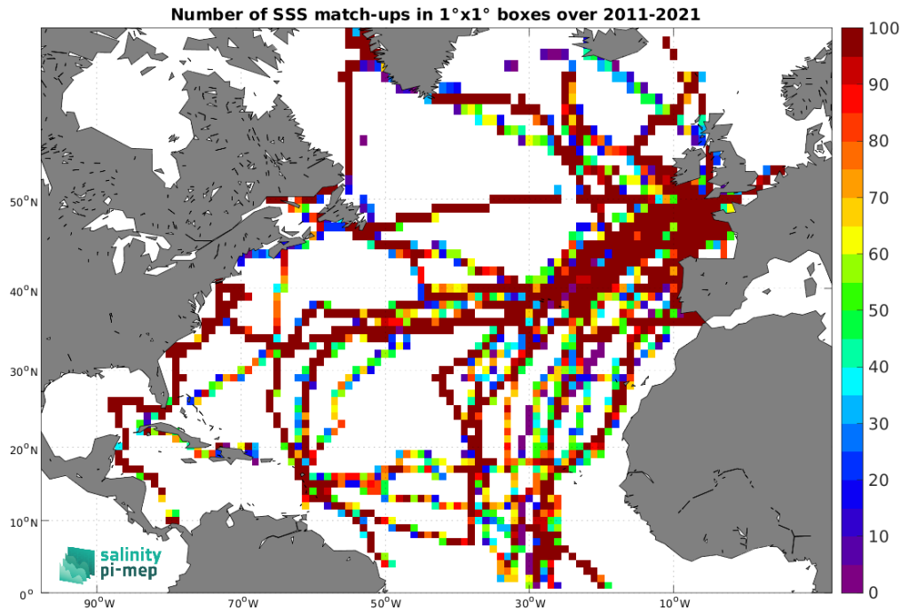
Figure 5: Number of SSS match-ups between TSG (GOSUD-Sailing-ship) SSS and the SMOS SSS L3 v2 - 9-Days (BEC) SSS product for the North Atlantic Ocean Pi-MEP region over 1^\circ \times 1^\circ boxes and for the full satellite product period.
