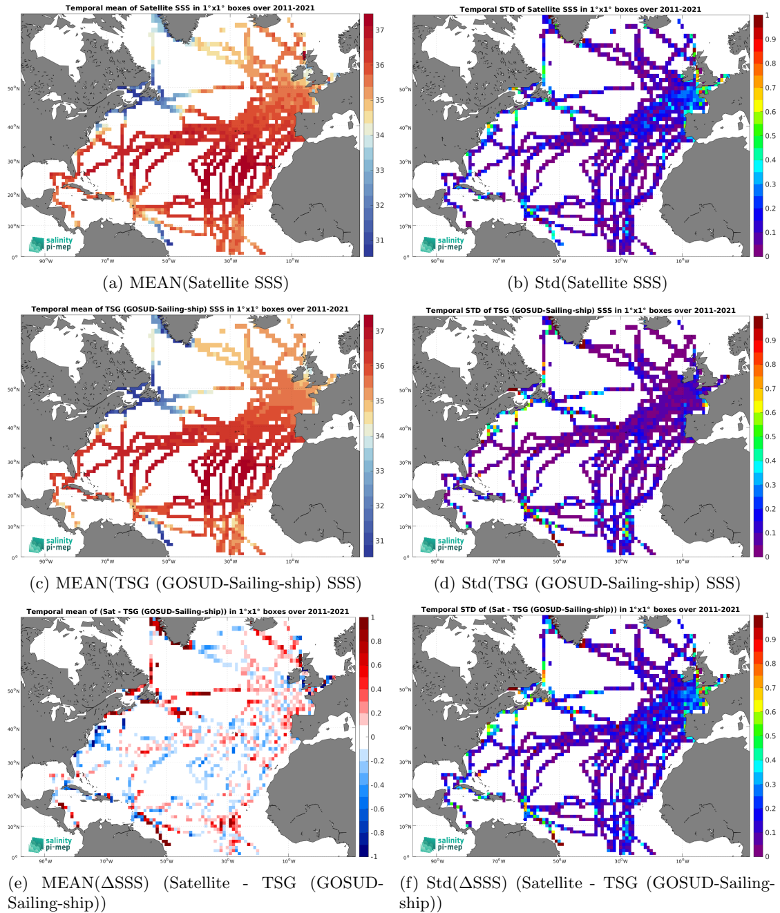
Figure 7: Temporal mean (left) and Std (right) of SSS from SMOS SSS L3 v2 - 9-Days (BEC) (top), TSG (GOSUD-Sailing-ship) (middle), and of \Delta SSS (Satellite - TSG (GOSUD-Sailing-ship)). Only match-up pairs are used to generate these maps.
