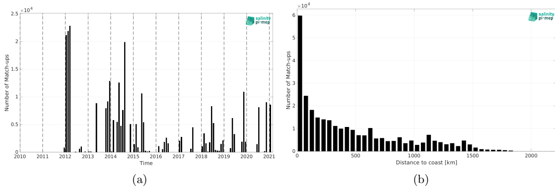
Figure 2: Number of match-ups between TSG (GOSUD-Sailing-ship) and SMOS SSS L3 v2 - 9-Days (BEC) SSS as a function of time (a) and as function of the distance to coast (b) over the North Atlantic Ocean Pi-MEP region and for the full satellite product period.
