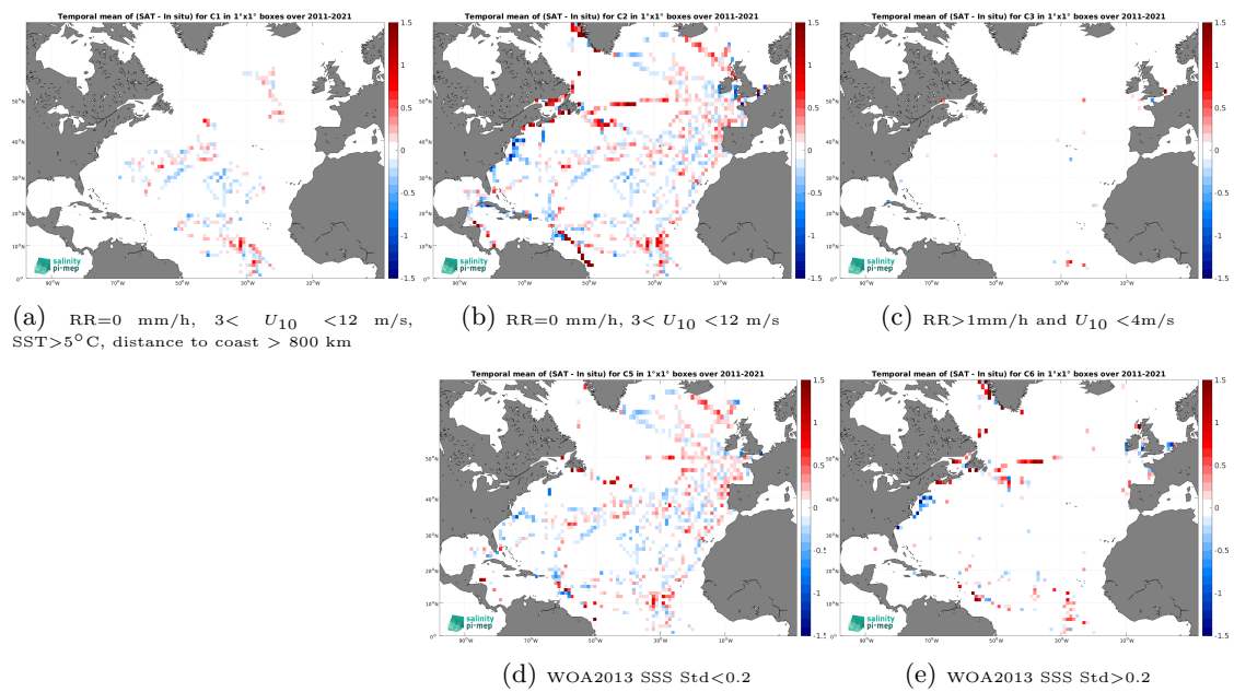
Figure 14: Temporal mean gridded over spatial boxes of size 1^\circ \times 1^\circ of \Delta\text{SSS} (SMOS SSS L3 v2 - 9-Days (BEC) - TSG (GOSUD-Sailing-ship)) for 5 different subdatasets corresponding to:RR=0 mm/h, 3 < U_{10} < 12 m/s, SST >5^\circ\text{C} , distance to coast > 800 km (a), RR=0 mm/h, 3 < U_{10} < 12 m/s (b), RR >1 mm/h and U_{10} < 4 m/s (c), WOA2013 SSS Std <0.2 (d), WOA2013 SSS Std >0.2 (e).
