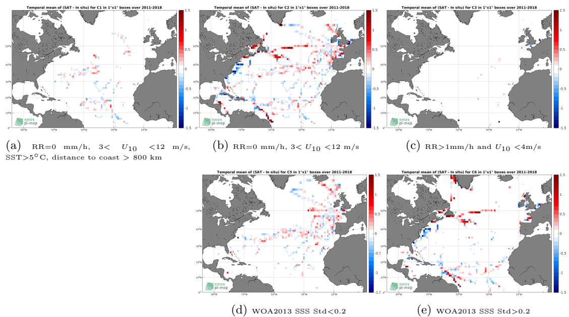
Figure 12: Temporal mean gridded over spatial boxes of size 1°x1° of \Delta\text{SSS} (SMOS SSS L3 v2 - 9-Days (BEC) - TSG (GOSUD-Sailing-ship)) for 5 different subdatasets corresponding to:RR=0 mm/h, 3 < U_{10} < 12 m/s, SST>5°C, distance to coast > 800 km (a), RR=0 mm/h, 3 < U_{10} < 12 m/s (b), RR>1mm/h and U_{10} < 4 m/s (c), WOA2013 SSS Std<0.2 (d), WOA2013 SSS Std>0.2 (e).
