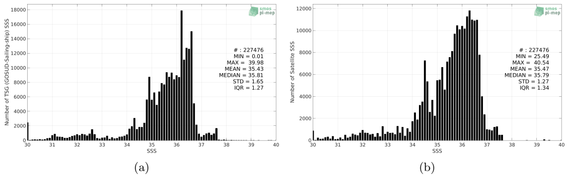
Figure 2: Histograms of SSS from TSG (GOSUD-Sailing-ship) (a) and SMOS SSS L3 v2 - 9-Days (BEC) (b) considering all match-up pairs per bins of 0.1 over the North Atlantic Ocean Pi-MEP region and for the full satellite product period.
