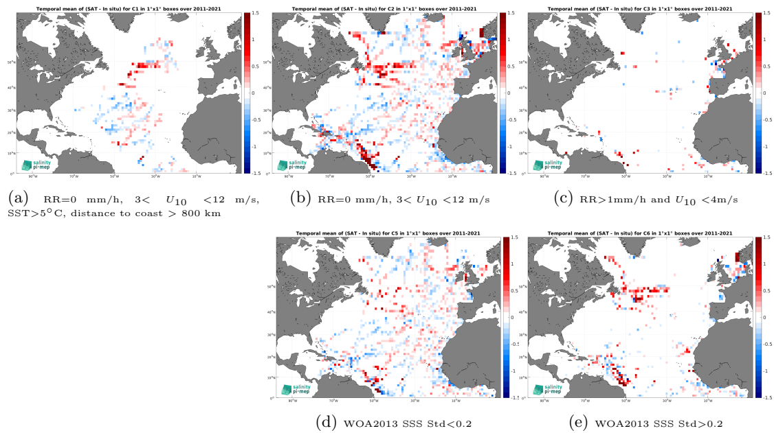
Figure 14: Temporal mean gridded over spatial boxes of size 1^\circ \times 1^\circ of \Delta\text{SSS} (SMOS SSS L3 v2 - 9-Days (BEC) - TSG (GOSUD-Research-vessel)) for 5 different subdatasets corresponding to:RR=0 mm/h, 3 < U_{10} < 12 m/s, SST>5°C, distance to coast > 800 km (a), RR=0 mm/h, 3 < U_{10} < 12 m/s (b), RR>1mm/h and U_{10} < 4 m/s (c), WOA2013 SSS Std<0.2 (d), WOA2013 SSS Std>0.2 (e).
