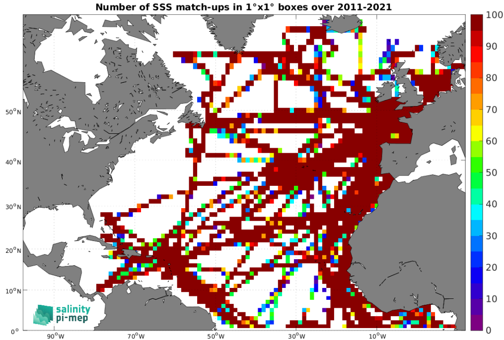
Figure 5: Number of SSS match-ups between TSG (GOSUD-Research-vessel) SSS and the SMOS SSS L3 v2 - 9-Days (BEC) SSS product for the North Atlantic Ocean Pi-MEP region over 1^\circ \times 1^\circ boxes and for the full satellite product period.
