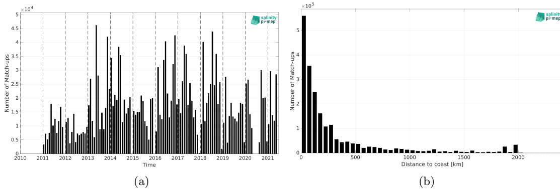
Figure 2: Number of match-ups between TSG (GOSUD-Research-vessel) and SMOS SSS L3 v2 - 9-Days (BEC) SSS as a function of time (a) and as function of the distance to coast (b) over the North Atlantic Ocean Pi-MEP region and for the full satellite product period.
