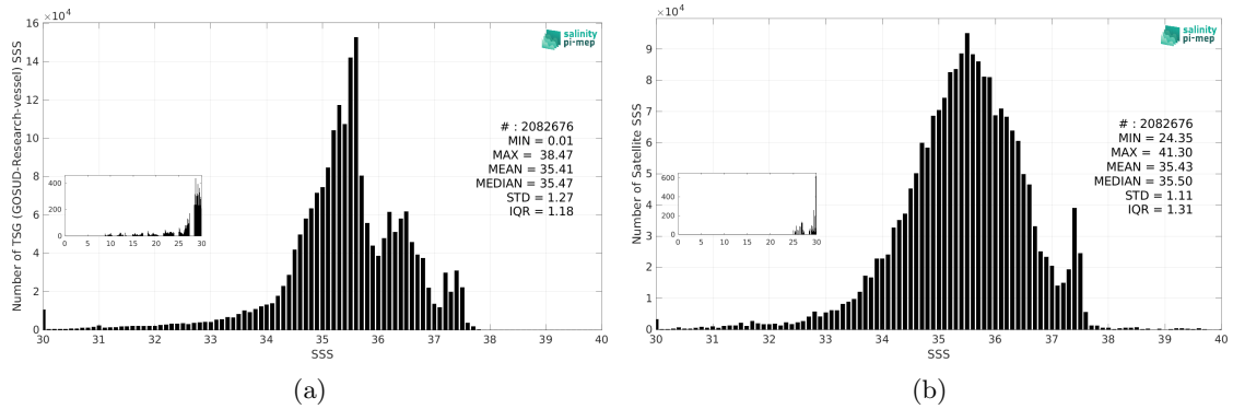
Figure 3: Histograms of SSS from TSG (GOSUD-Research-vessel) (a) and SMOS SSS L3 v2 - 9-Days (BEC) (b) considering all match-up pairs per bins of 0.1 over the North Atlantic Ocean Pi-MEP region and for the full satellite product period.
