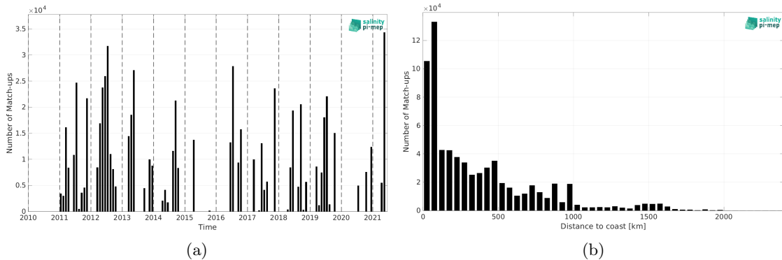
Figure 2: Number of match-ups between TSG (CSIC-UTM) and SMOS SSS L3 v2 - 9-Days (BEC) SSS as a function of time (a) and as function of the distance to coast (b) over the North Atlantic Ocean Pi-MEP region and for the full satellite product period.
