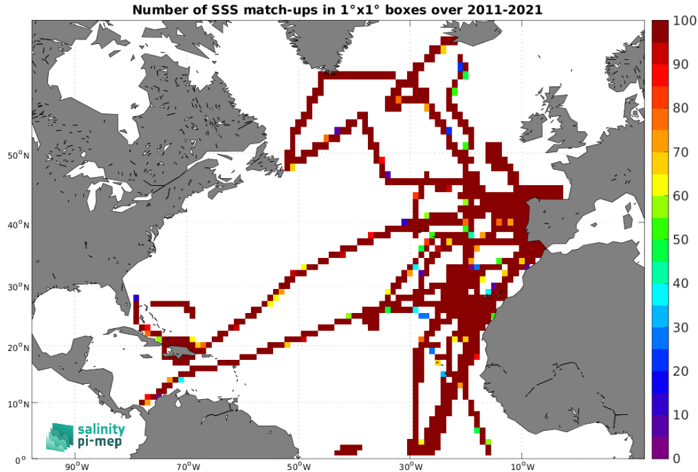
Figure 5: Number of SSS match-ups between TSG (CSIC-UTM) SSS and the SMOS SSS L3 v2 - 9-Days (BEC) SSS product for the North Atlantic Ocean Pi-MEP region over 1^\circ \times 1^\circ boxes and for the full satellite product period.
