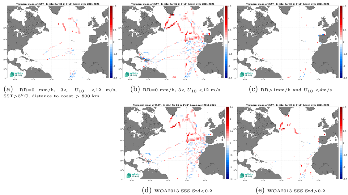
Figure 14: Temporal mean gridded over spatial boxes of size 1^\circ \times 1^\circ of \Delta\text{SSS} (SMOS SSS L3 v2 - 9-Days (BEC) - TSG (CSIC-UTM)) for 5 different subdatasets corresponding to:RR=0 mm/h, 3 < U_{10} < 12 m/s, SST >5^\circ\text{C} , distance to coast > 800 km (a), RR=0 mm/h, 3 < U_{10} < 12 m/s (b), RR >1 mm/h and U_{10} < 4 m/s (c), WOA2013 SSS Std <0.2 (d), WOA2013 SSS Std >0.2 (e).
