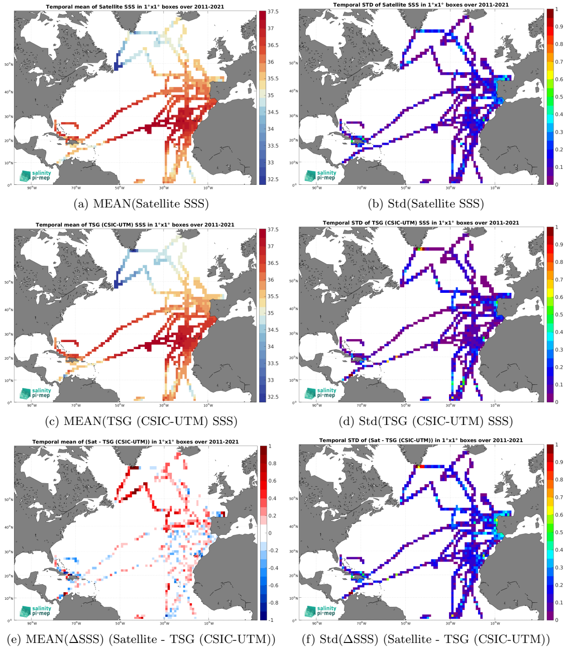
Figure 7: Temporal mean (left) and Std (right) of SSS from SMOS SSS L3 v2 - 9-Days (BEC) (top), TSG (CSIC-UTM) (middle), and of \Delta SSS (Satellite - TSG (CSIC-UTM)). Only match-up pairs are used to generate these maps.
