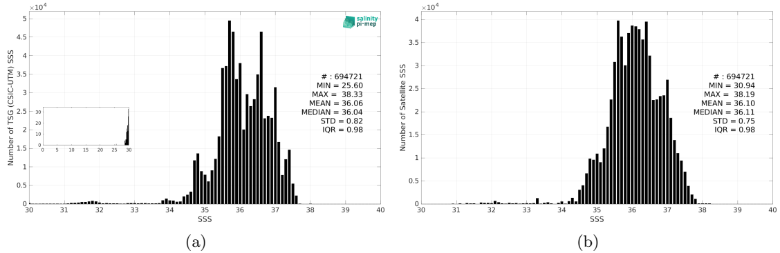
Figure 3: Histograms of SSS from TSG (CSIC-UTM) (a) and SMOS SSS L3 v2 - 9-Days (BEC) (b) considering all match-up pairs per bins of 0.1 over the North Atlantic Ocean Pi-MEP region and for the full satellite product period.
