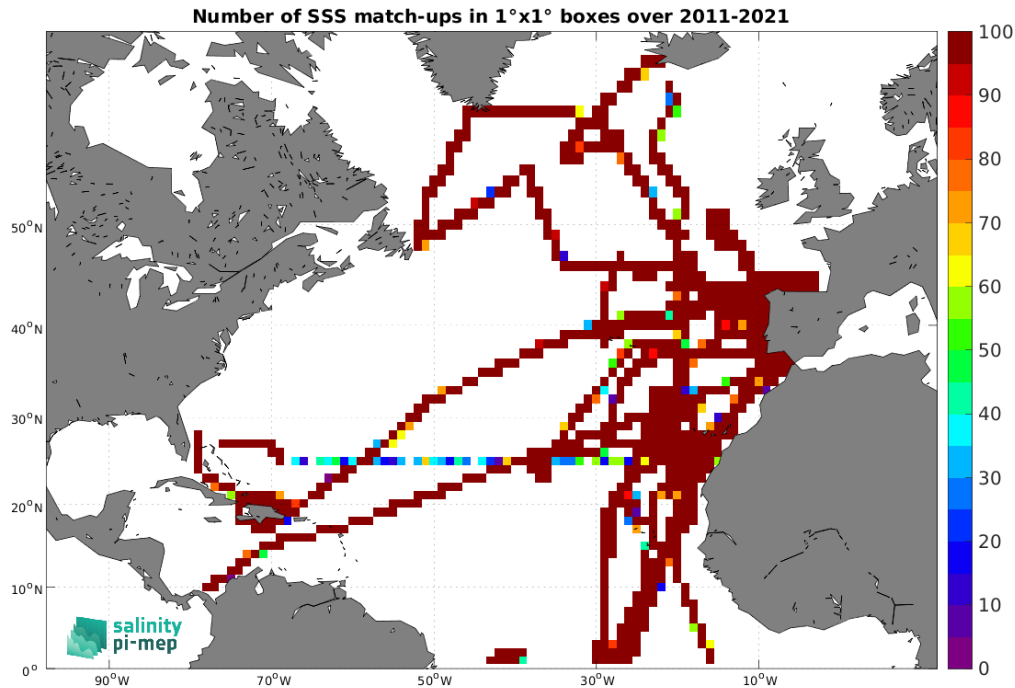
Figure 4: Number of SSS match-ups between TSG (CSIC-UTM) SSS and the SMOS SSS L3 v2 - 9-Days (BEC) SSS product for the North Atlantic Ocean Pi-MEP region over 1^\circ \times 1^\circ boxes and for the full satellite product period.
