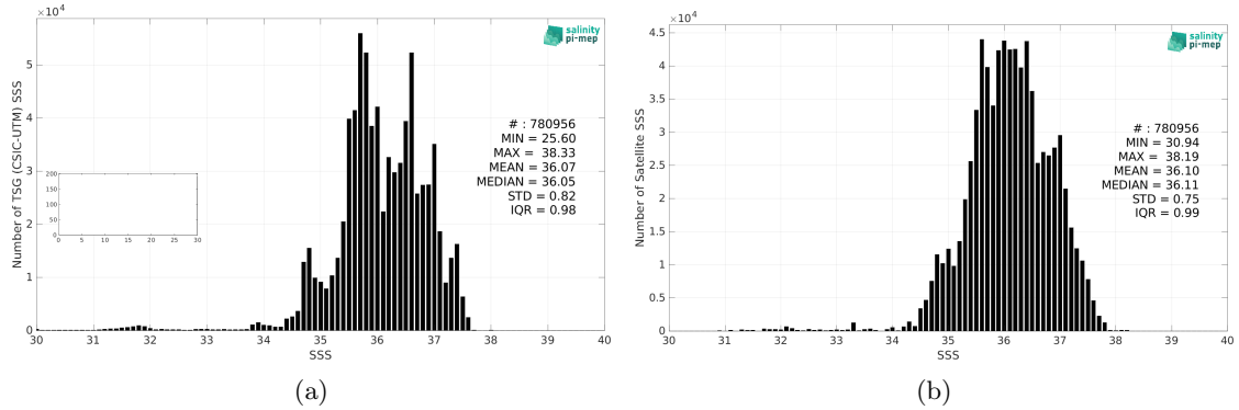
Figure 2: Histograms of SSS from TSG (CSIC-UTM) (a) and SMOS SSS L3 v2 - 9-Days (BEC) (b) considering all match-up pairs per bins of 0.1 over the North Atlantic Ocean Pi-MEP region and for the full satellite product period.
