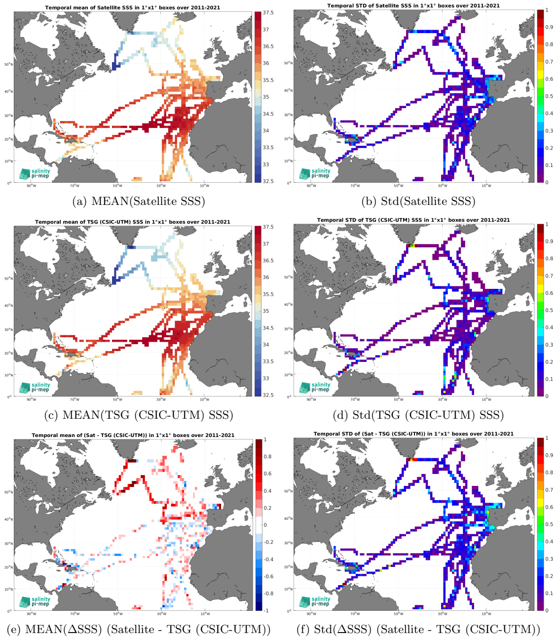
Figure 6: Temporal mean (left) and Std (right) of SSS from SMOS SSS L3 v2 - 9-Days (BEC) (top), TSG (CSIC-UTM) (middle), and of \Delta SSS (Satellite - TSG (CSIC-UTM)). Only match-up pairs are used to generate these maps.
