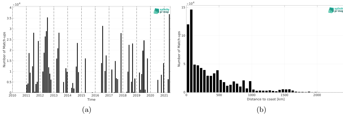
Figure 1: Number of match-ups between TSG (CSIC-UTM) and SMOS SSS L3 v2 - 9-Days (BEC) SSS as a function of time (a) and as function of the distance to coast (b) over the North Atlantic Ocean Pi-MEP region and for the full satellite product period.
