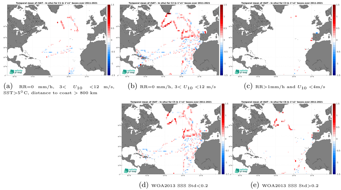
Figure 12: Temporal mean gridded over spatial boxes of size 1^\circ \times 1^\circ of \Delta\text{SSS} (SMOS SSS L3 v2 - 9-Days (BEC) - TSG (CSIC-UTM)) for 5 different subdatasets corresponding to:RR=0 mm/h, 3 < U_{10} < 12 m/s, SST >5^\circ\text{C} , distance to coast > 800 km (a), RR=0 mm/h, 3 < U_{10} < 12 m/s (b), RR >1 mm/h and U_{10} < 4 m/s (c), WOA2013 SSS Std <0.2 (d), WOA2013 SSS Std >0.2 (e).
