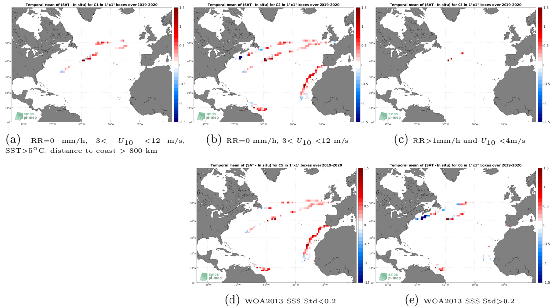
Figure 12: Temporal mean gridded over spatial boxes of size 1^\circ \times 1^\circ of \Delta SSS (SMOS SSS L3 v2 - 9-Days (BEC) - Saildrone) for 5 different subdatasets corresponding to:RR=0 mm/h, 3 < U_{10} < 12 m/s, SST >5^\circ C, distance to coast > 800 km (a), RR=0 mm/h, 3 < U_{10} < 12 m/s (b), RR >1 mm/h and U_{10} < 4 m/s (c), WOA2013 SSS Std <0.2 (d), WOA2013 SSS Std >0.2 (e).
