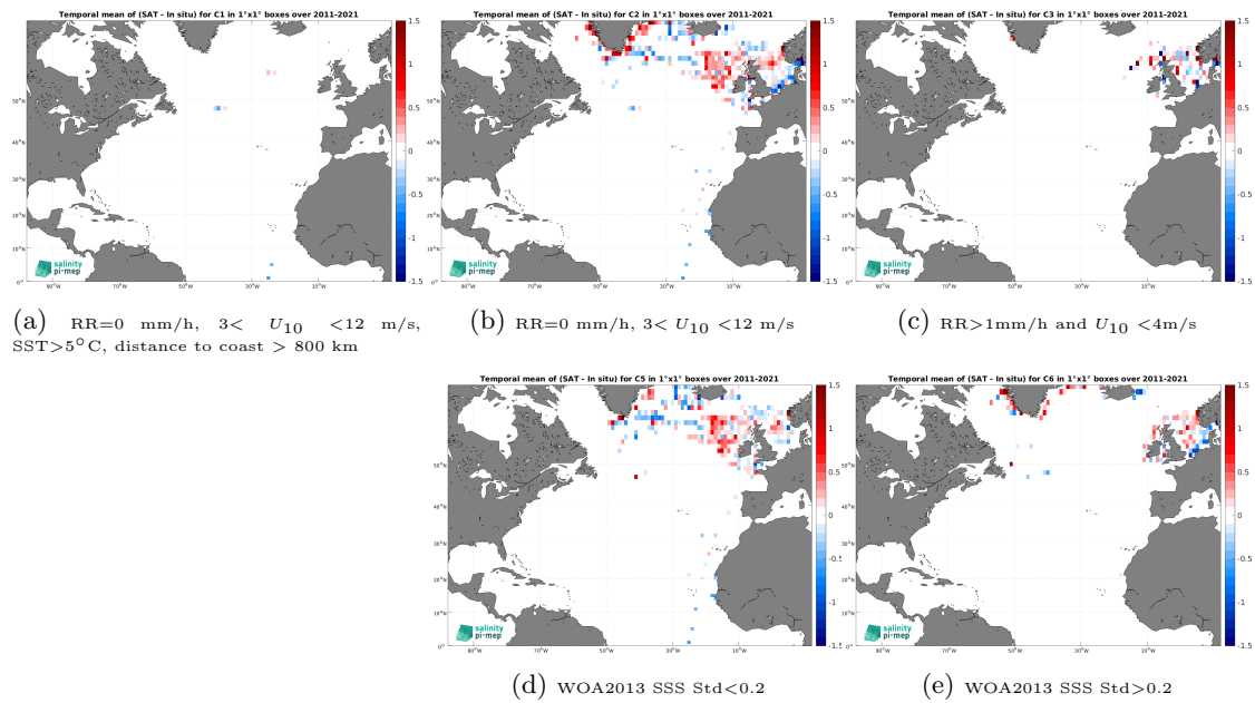
Figure 14: Temporal mean gridded over spatial boxes of size 1^\circ \times 1^\circ of \Delta\text{SSS} (SMOS SSS L3 v2 - 9-Days (BEC) - ICES) for 5 different subdatasets corresponding to:RR=0 mm/h, 3 < U_{10} < 12 m/s, SST>5°C, distance to coast > 800 km (a), RR=0 mm/h, 3 < U_{10} < 12 m/s (b), RR>1mm/h and U_{10} < 4 m/s (c), WOA2013 SSS Std<0.2 (d), WOA2013 SSS Std>0.2 (e).
