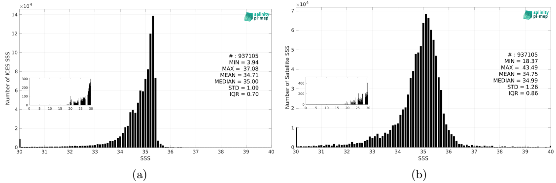
Figure 3: Histograms of SSS from ICES (a) and SMOS SSS L3 v2 - 9-Days (BEC) (b) considering all match-up pairs per bins of 0.1 over the North Atlantic Ocean Pi-MEP region and for the full satellite product period.
