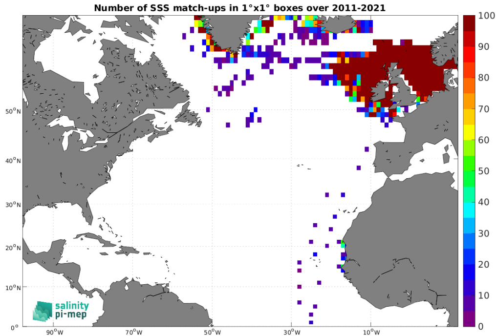
Figure 5: Number of SSS match-ups between ICES SSS and the SMOS SSS L3 v2 - 9-Days (BEC) SSS product for the North Atlantic Ocean Pi-MEP region over 1^\circ \times 1^\circ boxes and for the full satellite product period.
