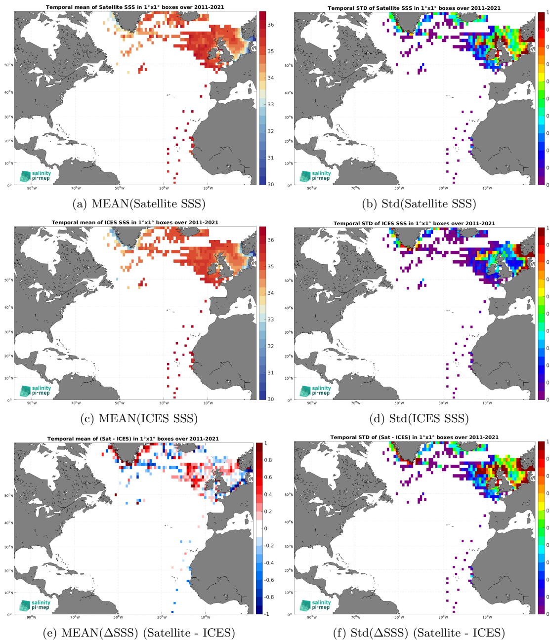
Figure 7: Temporal mean (left) and Std (right) of SSS from SMOS SSS L3 v2 - 9-Days (BEC) (top), ICES (middle), and of \Delta SSS (Satellite - ICES). Only match-up pairs are used to generate these maps.
