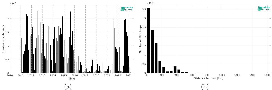
Figure 2: Number of match-ups between ICES and SMOS SSS L3 v2 - 9-Days (BEC) SSS as a function of time (a) and as function of the distance to coast (b) over the North Atlantic Ocean Pi-MEP region and for the full satellite product period.
