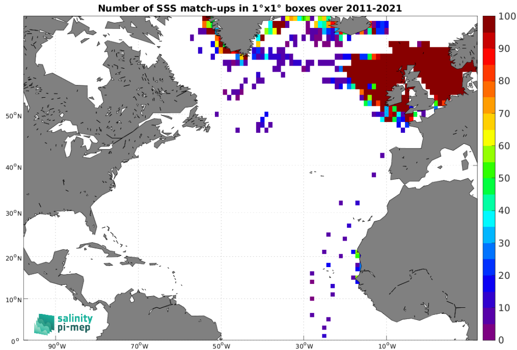
Figure 4: Number of SSS match-ups between ICES SSS and the SMOS SSS L3 v2 - 9-Days (BEC) SSS product for the North Atlantic Ocean Pi-MEP region over 1^\circ \times 1^\circ boxes and for the full satellite product period.
