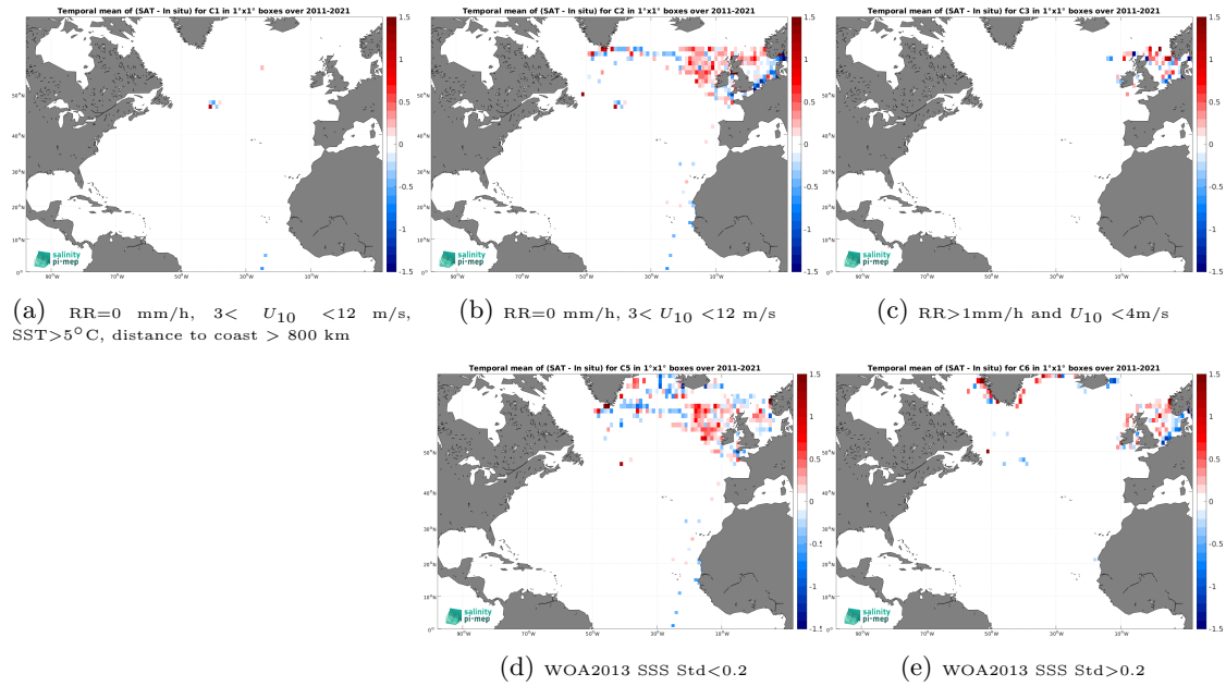
Figure 12: Temporal mean gridded over spatial boxes of size 1^\circ \times 1^\circ of \Delta SSS (SMOS SSS L3 v2 - 9-Days (BEC) - ICES) for 5 different subdatasets corresponding to:RR=0 mm/h, 3 < U_{10} < 12 m/s, SST >5^\circ\text{C} , distance to coast > 800 km (a), RR=0 mm/h, 3 < U_{10} < 12 m/s (b), RR >1 mm/h and U_{10} < 4 m/s (c), WOA2013 SSS Std <0.2 (d), WOA2013 SSS Std >0.2 (e).
