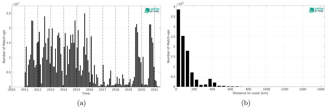
Figure 1: Number of match-ups between ICES and SMOS SSS L3 v2 - 9-Days (BEC) SSS as a function of time (a) and as function of the distance to coast (b) over the North Atlantic Ocean Pi-MEP region and for the full satellite product period.
