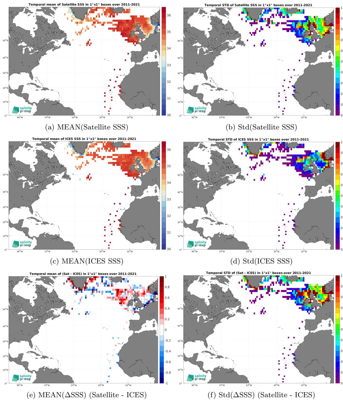
Figure 6: Temporal mean (left) and Std (right) of SSS from SMOS SSS L3 v2 - 9-Days (BEC) (top), ICES (middle), and of \Delta SSS (Satellite - ICES). Only match-up pairs are used to generate these maps.
