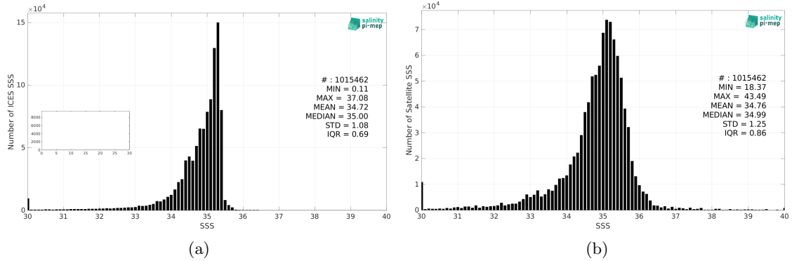
Figure 2: Histograms of SSS from ICES (a) and SMOS SSS L3 v2 - 9-Days (BEC) (b) considering all match-up pairs per bins of 0.1 over the North Atlantic Ocean Pi-MEP region and for the full satellite product period.
