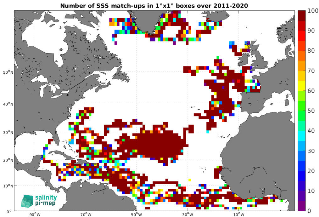
Figure 4: Number of SSS match-ups between Surface drifters SSS and the SMOS SSS L3 v2 - 9-Days (BEC) SSS product for the North Atlantic Ocean Pi-MEP region over 1^\circ \times 1^\circ boxes and for the full satellite product period.
