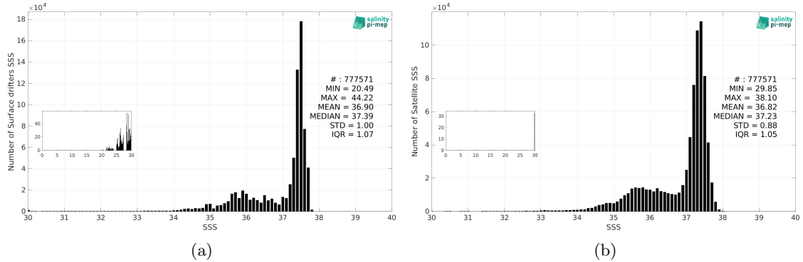
Figure 3: Histograms of SSS from Surface drifters (a) and SMOS SSS L3 v2 - 9-Days (BEC) (b) considering all match-up pairs per bins of 0.1 over the North Atlantic Ocean Pi-MEP region and for the full satellite product period.
