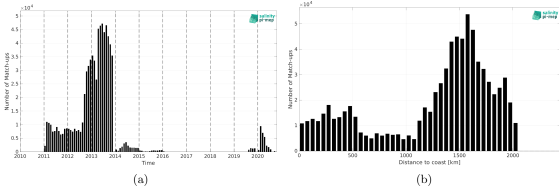
Figure 2: Number of match-ups between Surface drifters and SMOS SSS L3 v2 - 9-Days (BEC) SSS as a function of time (a) and as function of the distance to coast (b) over the North Atlantic Ocean Pi-MEP region and for the full satellite product period.
