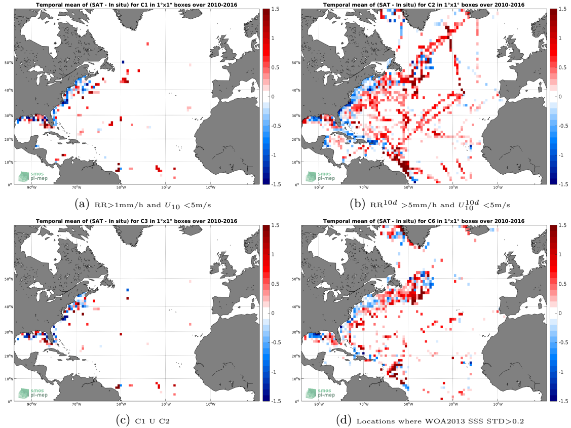
Figure 12: Temporal mean gridded over spatial boxes of size 1^\circ \times 1^\circ of \Delta SSS (SMOS-L3-BEC-OA-V1-9DAYS-0.25DEG - TSG-SAMOS) for 4 different subdatasets corresponding to:RR>1mm/h and U_{10} < 5\text{m/s} (a), RR^{10d} > 5\text{mm/h} and U_{10}^{10d} < 5\text{m/s} (b), C1 U C2 (c),Locations where WOA2013 SSS STD>0.2 (d).
