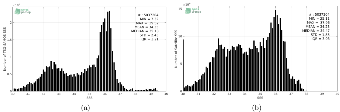
Figure 2: Histograms of SSS from TSG-SAMOS (a) and SMOS-L3-BEC-OA-V1-9DAYS-0.25DEG (b) considering all match-up pairs per bins of 0.1 over the North Atlantic Ocean Pi-MEP region and for the full satellite product period.
