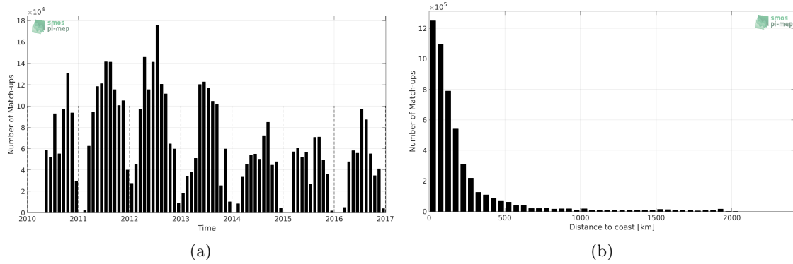
Figure 1: Number of match-ups between TSG-SAMOS and SMOS-L3-BEC-OA-V1-9DAYS-0.25DEG SSS as a function of time (a) and as function of the distance to coast (b) over the North Atlantic Ocean Pi-MEP region and for the full satellite product period.
