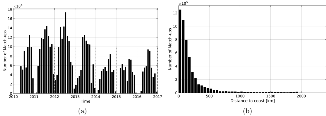
Figure 1: Number of match-ups between TSG-SAMOS and SMOS-L3-BEC-OA-V1-9DAYS-0.25DEG SSS as a function of time (a) and as function of the distance to coast (b) over the North Atlantic Ocean Pi-MEP region and for the full satellite product period.
