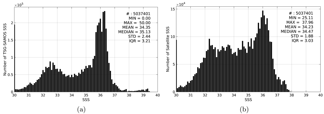
Figure 2: Histograms of SSS from TSG-SAMOS (a) and SMOS-L3-BEC-OA-V1-9DAYS-0.25DEG (b) considering all match-up pairs per bins of 0.1 over the North Atlantic Ocean Pi-MEP region and for the full satellite product period.
