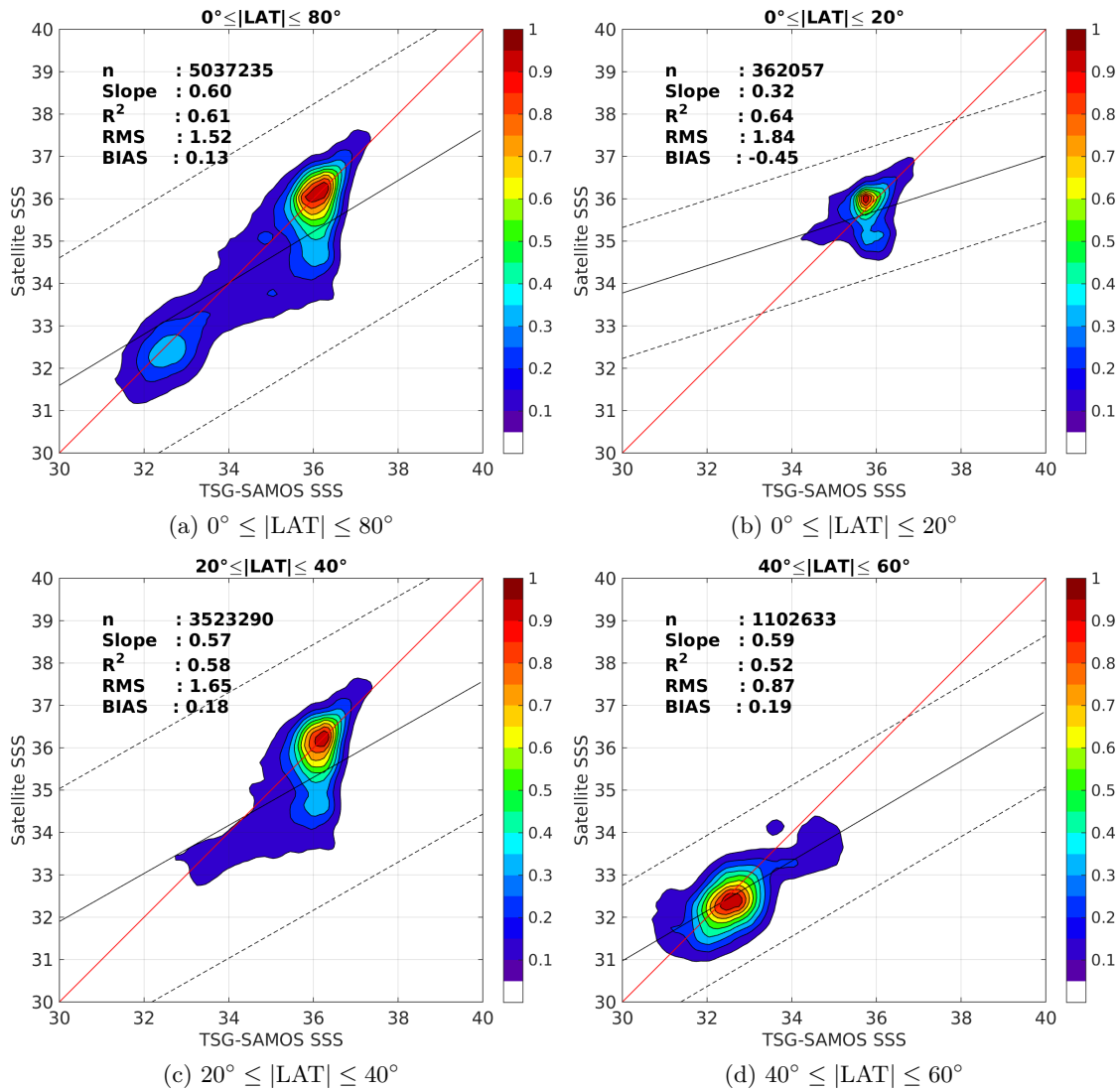
Figure 9: Contour maps of the concentration of SMOS-L3-BEC-OA-V1-9DAYS-0.25DEG SSS (y-axis) versus TSG-SAMOS SSS (x-axis) at match-up pairs for different latitude bands. For each plot, the red line shows x=y . The black thin and dashed lines indicate a linear fit through the data cloud and the \pm 95\% confidence levels, respectively. The number match-up pairs n , the slope and R^2 coefficient of the linear fit, the root mean square (RMS) and the mean bias between satellite and in situ data are indicated for each latitude band in each plots.
