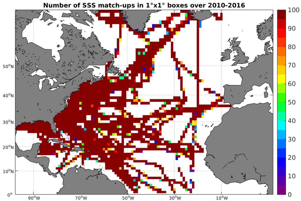
Figure 4: Number of SSS match-ups between TSG-SAMOS SSS and the SMOS-L3-BEC-OA-V1-9DAYS-0.25DEG SSS product for the North Atlantic Ocean Pi-MEP region over 1^\circ \times 1^\circ boxes and for the full satellite product period.
