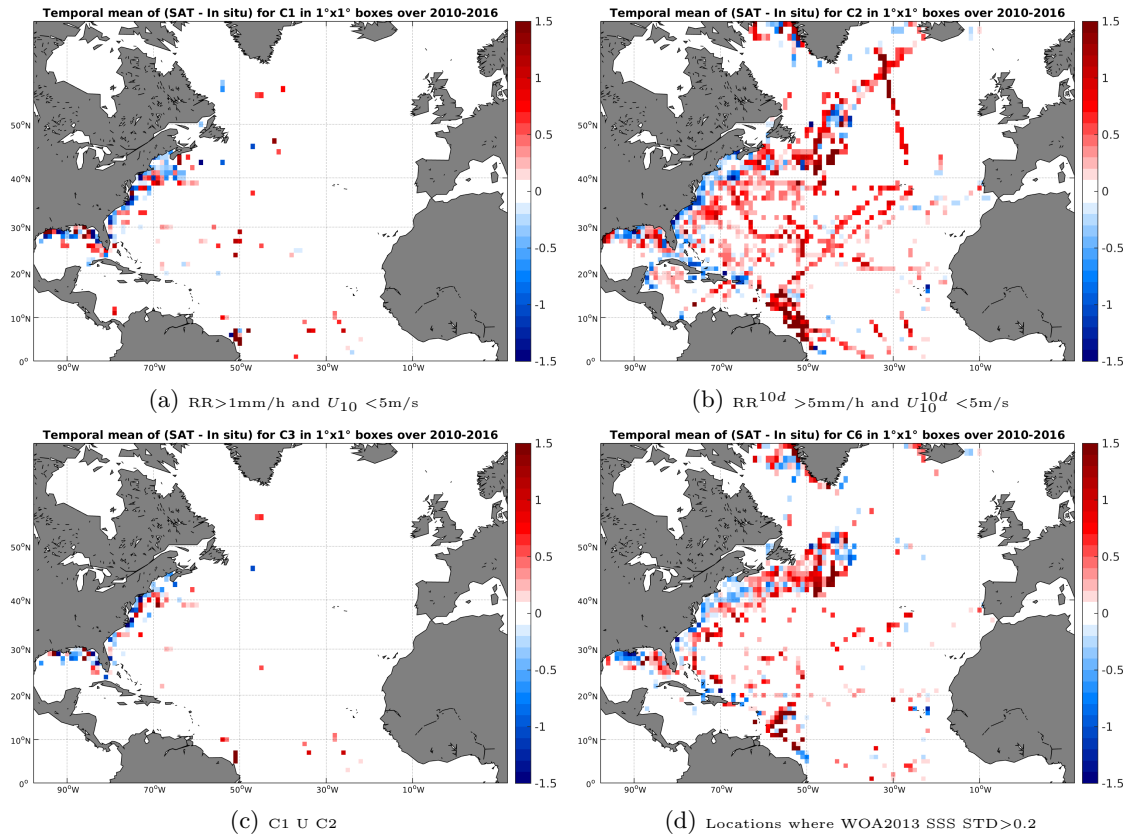
Figure 12: Temporal mean gridded over spatial boxes of size 1^\circ \times 1^\circ of \Delta SSS (SMOS-L3-BEC-OA-V1-9DAYS-0.25DEG - TSG-SAMOS) for 4 different subdatasets corresponding to: RR > 1\text{mm/h} and U_{10} < 5\text{m/s} (a), RR^{10d} > 5\text{mm/h} and U_{10}^{10d} < 5\text{m/s} (b), C1 U C2 (c), Locations where WOA2013 SSS STD > 0.2 (d).
