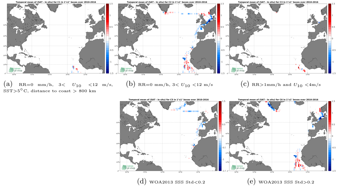
Figure 12: Temporal mean gridded over spatial boxes of size 1^\circ \times 1^\circ of \Delta SSS (SMOS-L3-BEC-OA-V1-9DAYS-0.25DEG - TSG-POLARSTERN) for 5 different subdatasets corresponding to: RR=0 mm/h, 3 < U_{10} < 12 m/s, SST > 5^\circ C , distance to coast > 800 km (a), RR=0 mm/h, 3 < U_{10} < 12 m/s (b), RR > 1 mm/h and U_{10} < 4 m/s (c), WOA2013 SSS Std < 0.2 (d), WOA2013 SSS Std > 0.2 (e).
