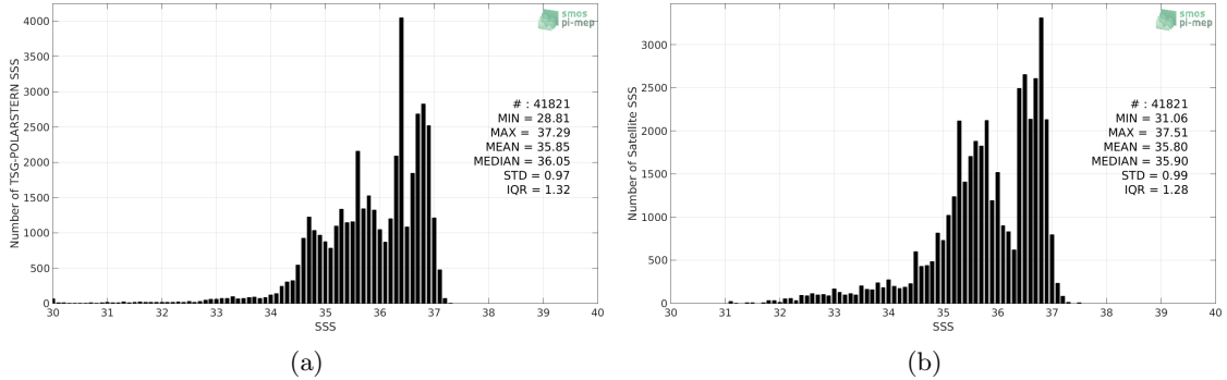
Figure 2: Histograms of SSS from TSG-POLARSTERN (a) and SMOS-L3-BEC-OA-V1-9DAYS-0.25DEG (b) considering all match-up pairs per bins of 0.1 over the North Atlantic Ocean Pi-MEP region and for the full satellite product period.
