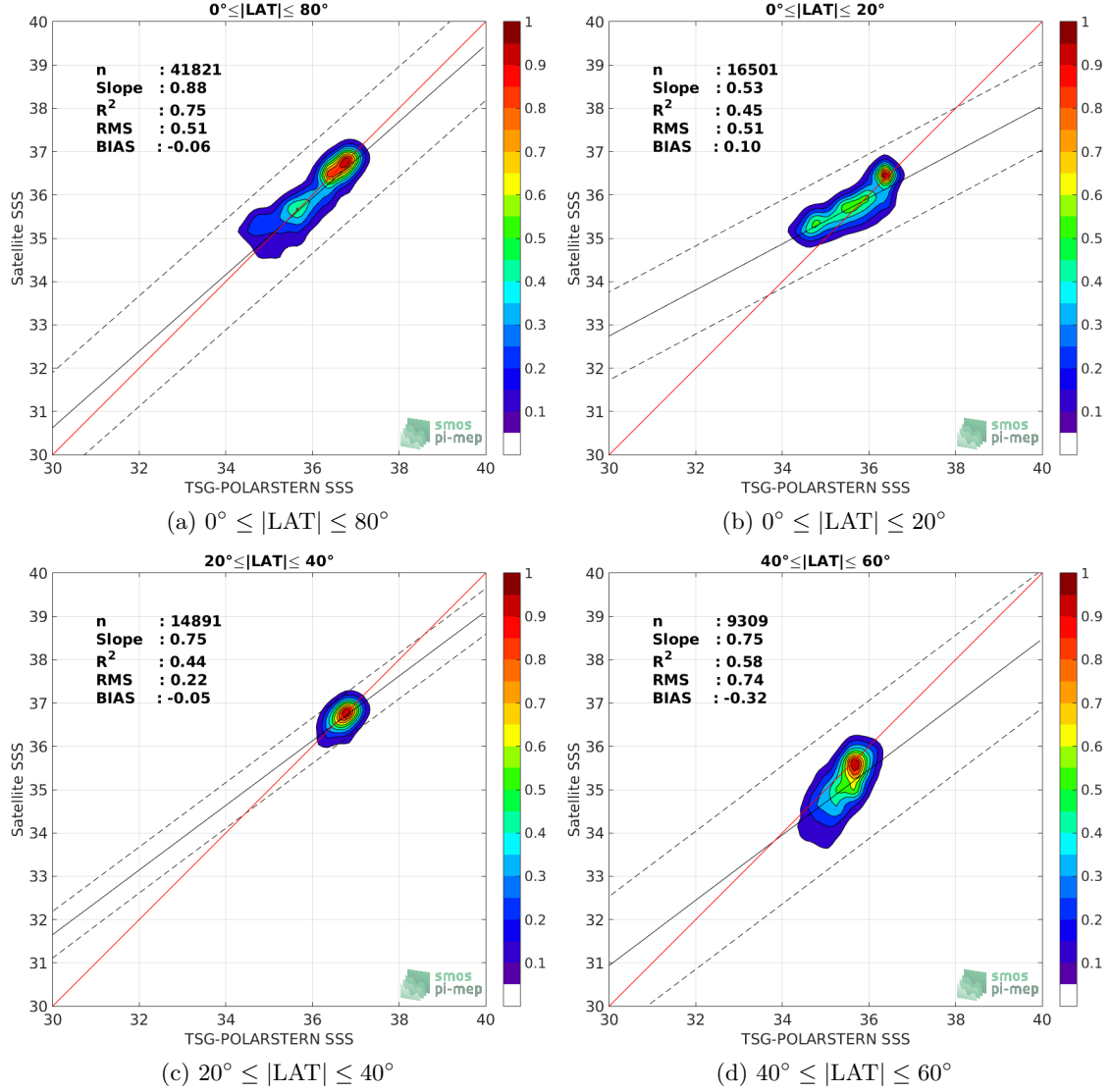
Figure 9: Contour maps of the concentration of SMOS-L3-BEC-OA-V1-9DAYS-0.25DEG SSS (y-axis) versus TSG-POLARSTERN SSS (x-axis) at match-up pairs for different latitude bands. For each plot, the red line shows x=y . The black thin and dashed lines indicate a linear fit through the data cloud and the \pm 95\% confidence levels, respectively. The number match-up pairs n , the slope and R^2 coefficient of the linear fit, the root mean square (RMS) and the mean bias between satellite and in situ data are indicated for each latitude band in each plots.
