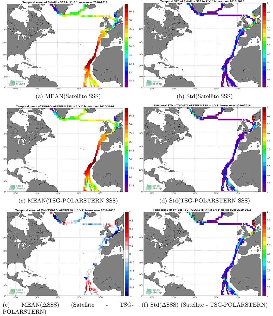
Figure 6: Temporal mean (left) and Std (right) of SSS from SMOS-L3-BEC-OA-V1-9DAYS-0.25DEG (top), TSG-POLARSTERN (middle), and of \Delta SSS (Satellite - TSG-POLARSTERN). Only match-up pairs are used to generate these maps.
