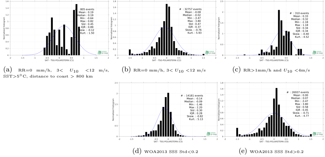
Figure 13: Normalized histogram of \Delta SSS (SMOS-L3-BEC-OA-V1-9DAYS-0.25DEG - TSG-POLARSTERN) for 5 different subdatasets corresponding to: RR=0 mm/h, 3 < U_{10} < 12 m/s, SST>5°C, distance to coast > 800 km (a), RR=0 mm/h, 3 < U_{10} < 12 m/s (b), RR>1mm/h and U_{10} < 4 m/s (c), WOA2013 SSS Std<0.2 (d), WOA2013 SSS Std>0.2 (e).
