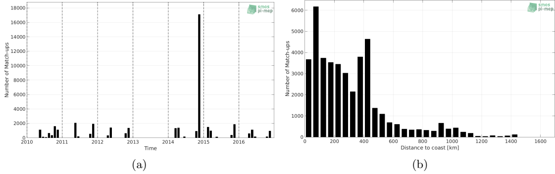
Figure 1: Number of match-ups between TSG-POLARSTERN and SMOS-L3-BEC-OA-V1-9DAYS-0.25DEG SSS as a function of time (a) and as function of the distance to coast (b) over the North Atlantic Ocean Pi-MEP region and for the full satellite product period.
