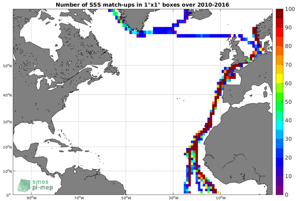
Figure 4: Number of SSS match-ups between TSG-POLARSTERN SSS and the SMOS-L3-BEC-OA-V1-9DAYS-0.25DEG SSS product for the North Atlantic Ocean Pi-MEP region over 1^\circ \times 1^\circ boxes and for the full satellite product period.
