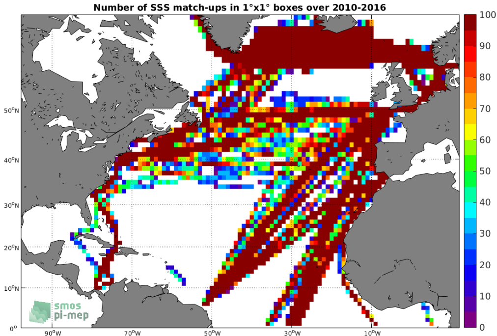
Figure 4: Number of SSS match-ups between TSG-LEGOS-DM SSS and the SMOS-L3-BECEOA-V1-9DAYS-0.25DEG SSS product for the North Atlantic Ocean Pi-MEP region over 1^\circ \times 1^\circ boxes and for the full satellite product period.
