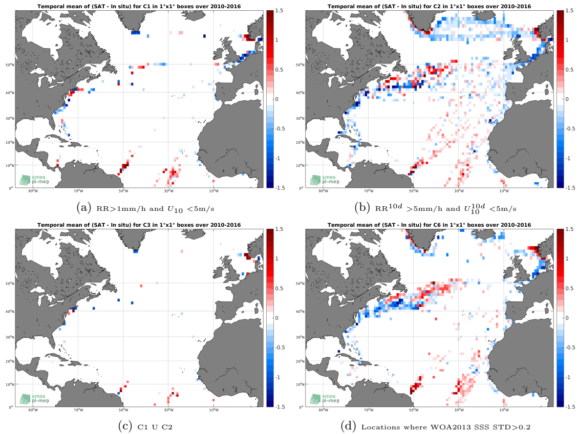
Figure 12: Temporal mean gridded over spatial boxes of size 1^\circ \times 1^\circ of \Delta SSS (SMOS-L3-BEC-OA-V1-9DAYS-0.25DEG - TSG-LEGOS-DM) for 4 different subdatasets corresponding to: RR > 1\text{mm/h} and U_{10} < 5\text{m/s} (a), RR^{10d} > 5\text{mm/h} and U_{10}^{10d} < 5\text{m/s} (b), C1 U C2 (c), Locations where WOA2013 SSS STD > 0.2 (d).
