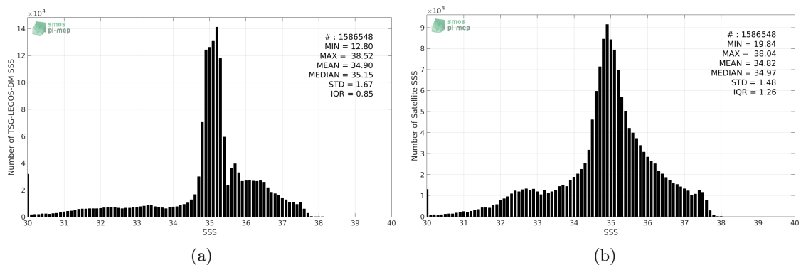
Figure 2: Histograms of SSS from TSG-LEGOS-DM (a) and SMOS-L3-BEC-OA-V1-9DAYS-0.25DEG (b) considering all match-up pairs per bins of 0.1 over the North Atlantic Ocean Pi-MEP region and for the full satellite product period.
