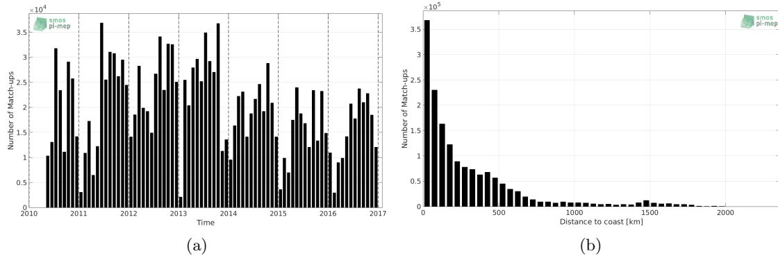
Figure 1: Number of match-ups between TSG-LEGOS-DM and SMOS-L3-BEC-OA-V1-9DAYS-0.25DEG SSS as a function of time (a) and as function of the distance to coast (b) over the North Atlantic Ocean Pi-MEP region and for the full satellite product period.
