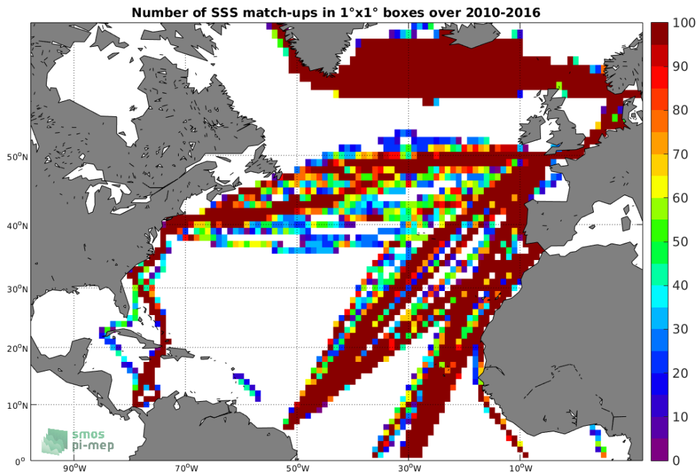
Figure 4: Number of SSS match-ups between TSG-LEGOS-DM SSS and the SMOS-L3-BEC-OA-V1-9DAYS-0.25DEG SSS product for the North Atlantic Ocean Pi-MEP region over 1^\circ \times 1^\circ boxes and for the full satellite product period.
