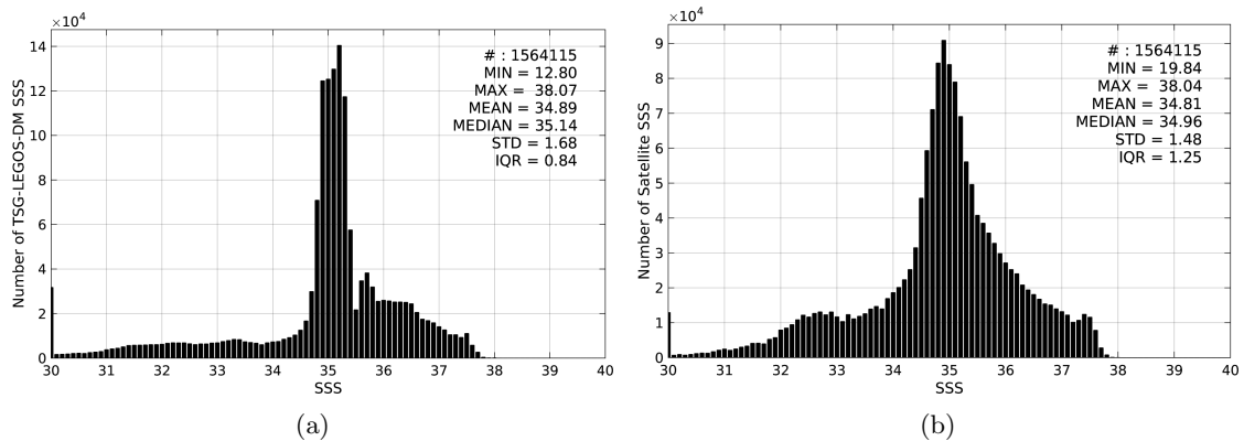
Figure 2: Histograms of SSS from TSG-LEGOS-DM (a) and SMOS-L3-BEC-OA-V1-9DAYS-0.25DEG (b) considering all match-up pairs per bins of 0.1 over the North Atlantic Ocean Pi-MEP region and for the full satellite product period.
