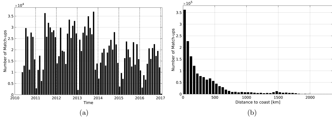
Figure 1: Number of match-ups between TSG-LEGOS-DM and SMOS-L3-BEC-OA-V1-9DAYS-0.25DEG SSS as a function of time (a) and as function of the distance to coast (b) over the North Atlantic Ocean Pi-MEP region and for the full satellite product period.
