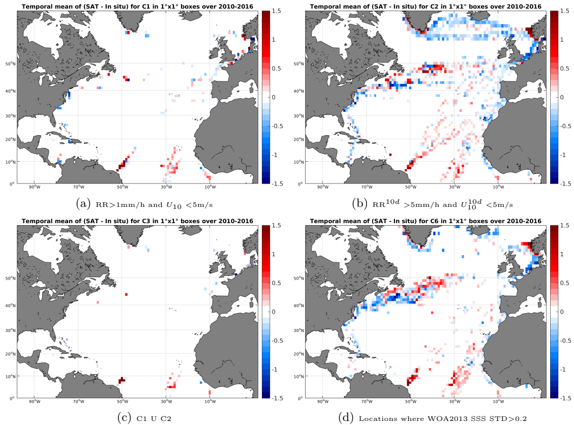
Figure 12: Temporal mean gridded over spatial boxes of size 1^\circ \times 1^\circ of \Delta SSS (SMOS-L3-BEC-OA-V1-9DAYS-0.25DEG - TSG-LEGOS-DM) for 4 different subdatasets corresponding to: RR > 1 mm/h and U_{10} < 5 m/s (a), RR 10d > 5 mm/h and U_{10}^{10d} < 5 m/s (b), C1 U C2 (c), Locations where WOA2013 SSS STD > 0.2 (d).
