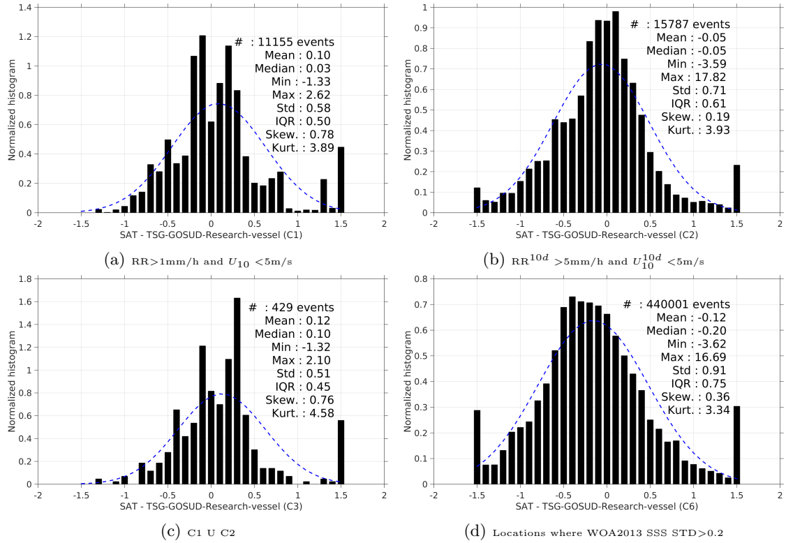
Figure 13: Normalized histogram of \Delta\text{SSS} (SMOS-L3-BEC-OA-V1-9DAYS-0.25DEG - TSG-GOSUD-Research-vessel) for 6 different subdatasets corresponding to: \text{RR} > 1\text{mm/h} and U_{10} < 5\text{m/s} (a), \text{RR}^{10d} > 5\text{mm/h} and U_{10}^{10d} < 5\text{m/s} (b), C1 U C2 (c), Locations where WOA2013 SSS STD > 0.2 (d).
