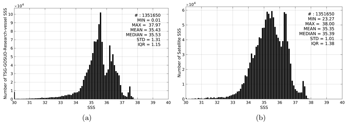
Figure 2: Histograms of SSS from TSG-GOSUD-Research-vessel (a) and SMOS-L3-BEC-OA-V1-9DAYS-0.25DEG (b) considering all match-up pairs per bins of 0.1 over the North Atlantic Ocean Pi-MEP region and for the full satellite product period.
