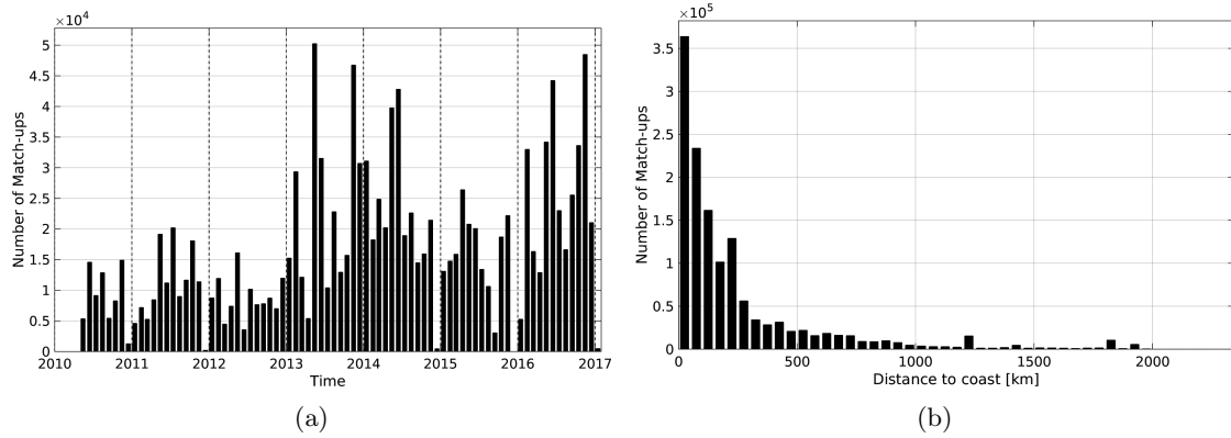
Figure 1: Number of match-ups between TSG-GOSUD-Research-vessel and SMOS-L3-BEC-OA-V1-9DAYS-0.25DEG SSS as a function of time (a) and as function of the distance to coast (b) over the North Atlantic Ocean Pi-MEP region and for the full satellite product period.
