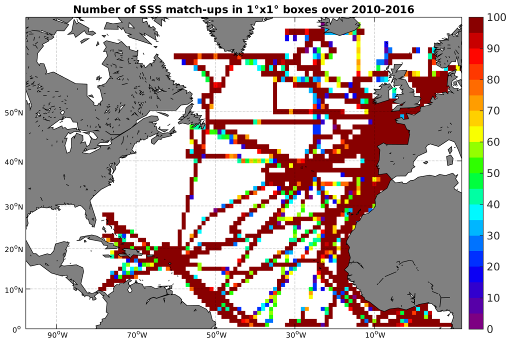
Figure 4: Number of SSS match-ups between TSG-GOSUD-Research-vessel SSS and the SMOS-L3-BEC-OA-V1-9DAYS-0.25DEG SSS product for the North Atlantic Ocean Pi-MEP region over 1^{\circ} \times 1^{\circ} boxes and for the full satellite product period.
