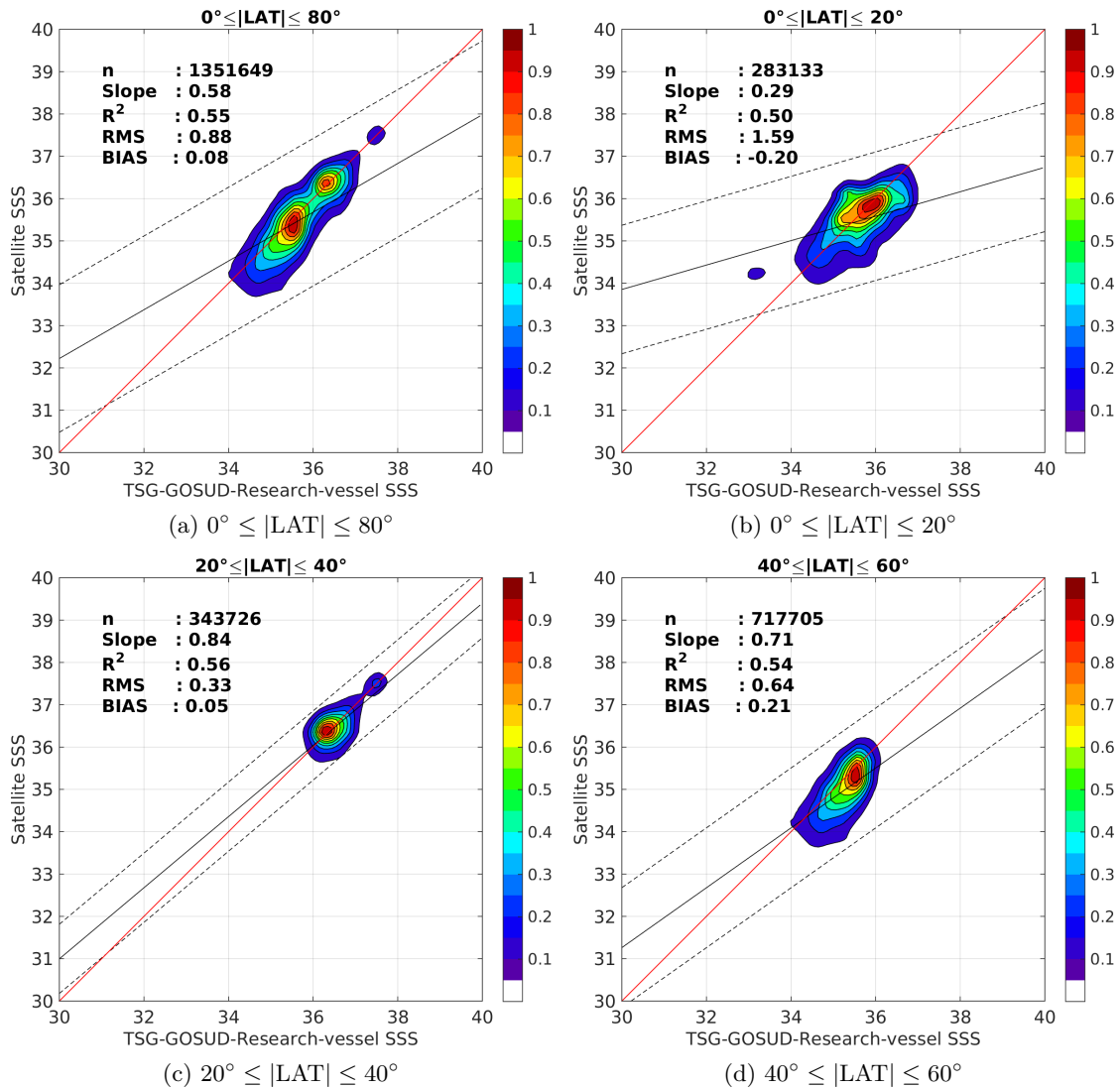
Figure 9: Contour maps of the concentration of SMOS-L3-BEC-OA-V1-9DAYS-0.25DEG SSS (y-axis) versus TSG-GOSUD-Research-vessel SSS (x-axis) at match-up pairs for different latitude bands. For each plot, the red line shows x=y . The black thin and dashed lines indicate a linear fit through the data cloud and the \pm 95\% confidence levels, respectively. The number match-up pairs n , the slope and R^2 coefficient of the linear fit, the root mean square (RMS) and the mean bias between satellite and in situ data are indicated for each latitude band in each plots.
