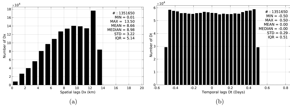
Figure 5: Histograms of the spatial (a) and temporal (b) lags between the time of the TSG-GOSUD-Research-vessel measurements and the date of the corresponding SMOS-L3-BEC-OA-V1-9DAYS-0.25DEG SSS product.
