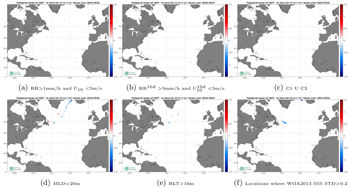
Figure 12: Temporal mean gridded over spatial boxes of size 1^\circ \times 1^\circ of \Delta SSS (SMOS-L3-BEC-OA-V1-9DAYS-0.25DEG - Sea mammals) for 6 different subdatasets corresponding to: RR > 1\text{mm/h} and U_{10} < 5\text{m/s} (a), RR^{10d} > 5\text{mm/h} and U_{10}^{10d} < 5\text{m/s} (b), C1 U C2 (c), MLD < 20\text{m} (d), BLT > 10\text{m} (e), Locations where WOA2013 SSS STD > 0.2 (f).
