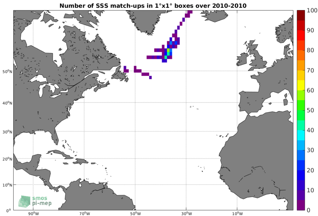
Figure 4: Number of SSS match-ups between Sea mammals SSS and the SMOS-L3-BEC-OA-V1-9DAYS-0.25DEG SSS product for the North Atlantic Ocean Pi-MEP region over 1°x1° boxes and for the full satellite product period.
