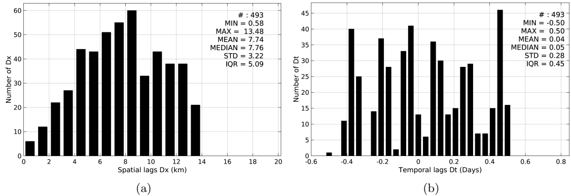
Figure 5: Histograms of the spatial (a) and temporal (b) lags between the time of the Sea mammals measurements and the date of the corresponding SMOS-L3-BEC-OA-V1-9DAYS-0.25DEG SSS product.
