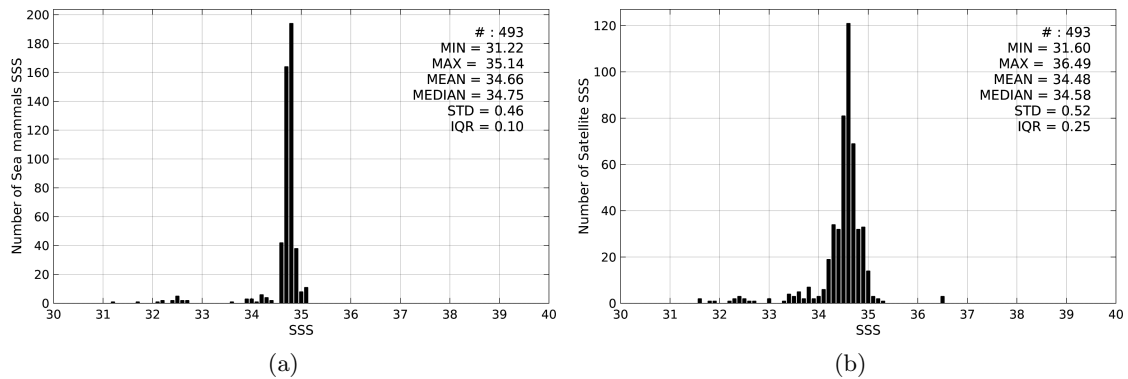
Figure 2: Histograms of SSS from Sea mammals (a) and SMOS-L3-BEC-OA-V1-9DAYS-0.25DEG (b) considering all match-up pairs per bins of 0.1 over the North Atlantic Ocean Pi-MEP region and for the full satellite product period.
