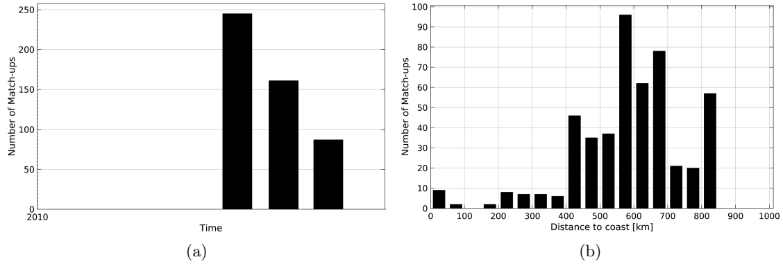
Figure 1: Number of match-ups between Sea mammals and SMOS-L3-BEC-OA-V1-9DAYS-0.25DEG SSS as a function of time (a) and as function of the distance to coast (b) over the North Atlantic Ocean Pi-MEP region and for the full satellite product period.
