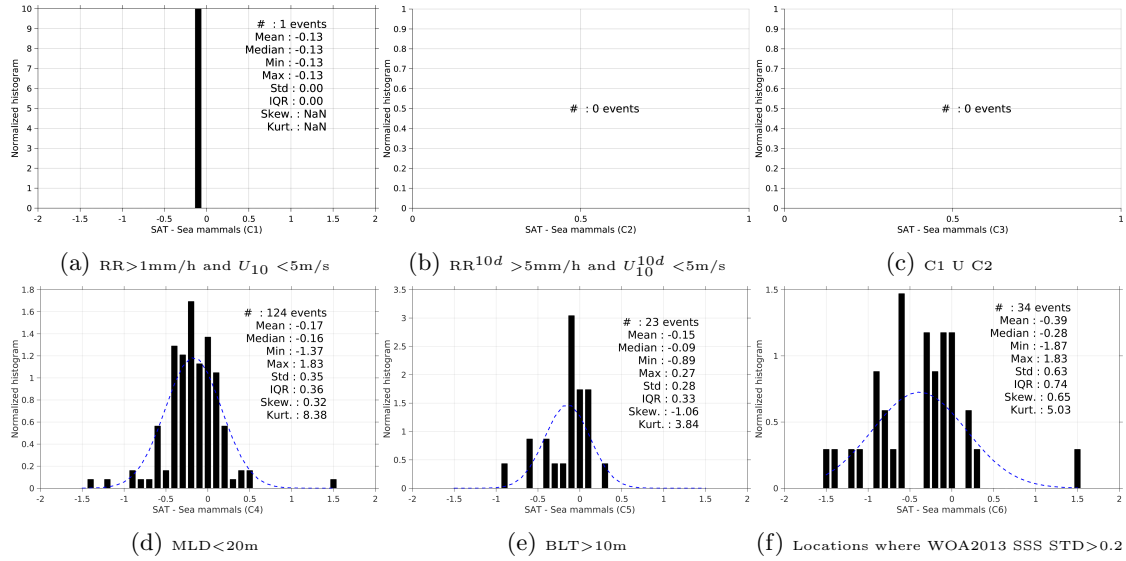
Figure 13: Normalized histogram of \Delta SSS (SMOS-L3-BEC-OA-V1-9DAYS-0.25DEG - Sea mammals) for 6 different subdatasets corresponding to: RR>1mm/h and U_{10} < 5\text{m/s} (a), RR 10d >5mm/h and U_{10}^{10d} < 5\text{m/s} (b), C1 U C2 (c),MLD<20m (d),BLT>10m (e),Locations where WOA2013 SSS STD>0.2 (f).
