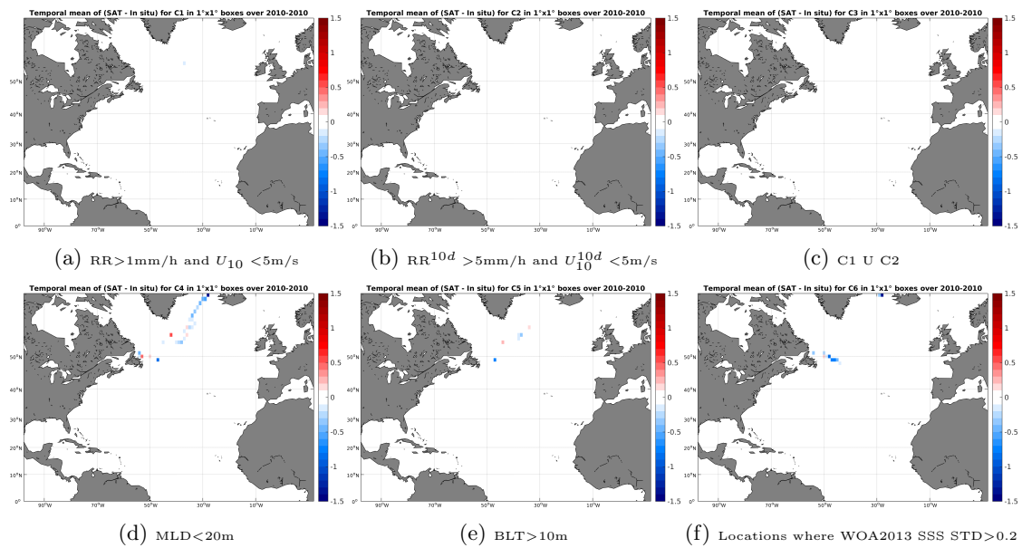
Figure 12: Temporal mean gridded over spatial boxes of size 1^\circ \times 1^\circ of \Delta SSS (SMOS-L3-BEC-OA-V1-9DAYS-0.25DEG - Sea mammals) for 6 different subdatasets corresponding to:RR > 1 mm/h and U_{10} < 5 m/s (a), RR 10d > 5 mm/h and U_{10}^{10d} < 5 m/s (b), C1 U C2 (c),MLD < 20 m (d),BLT > 10 m (e),Locations where WOA2013 SSS STD > 0.2 (f).
