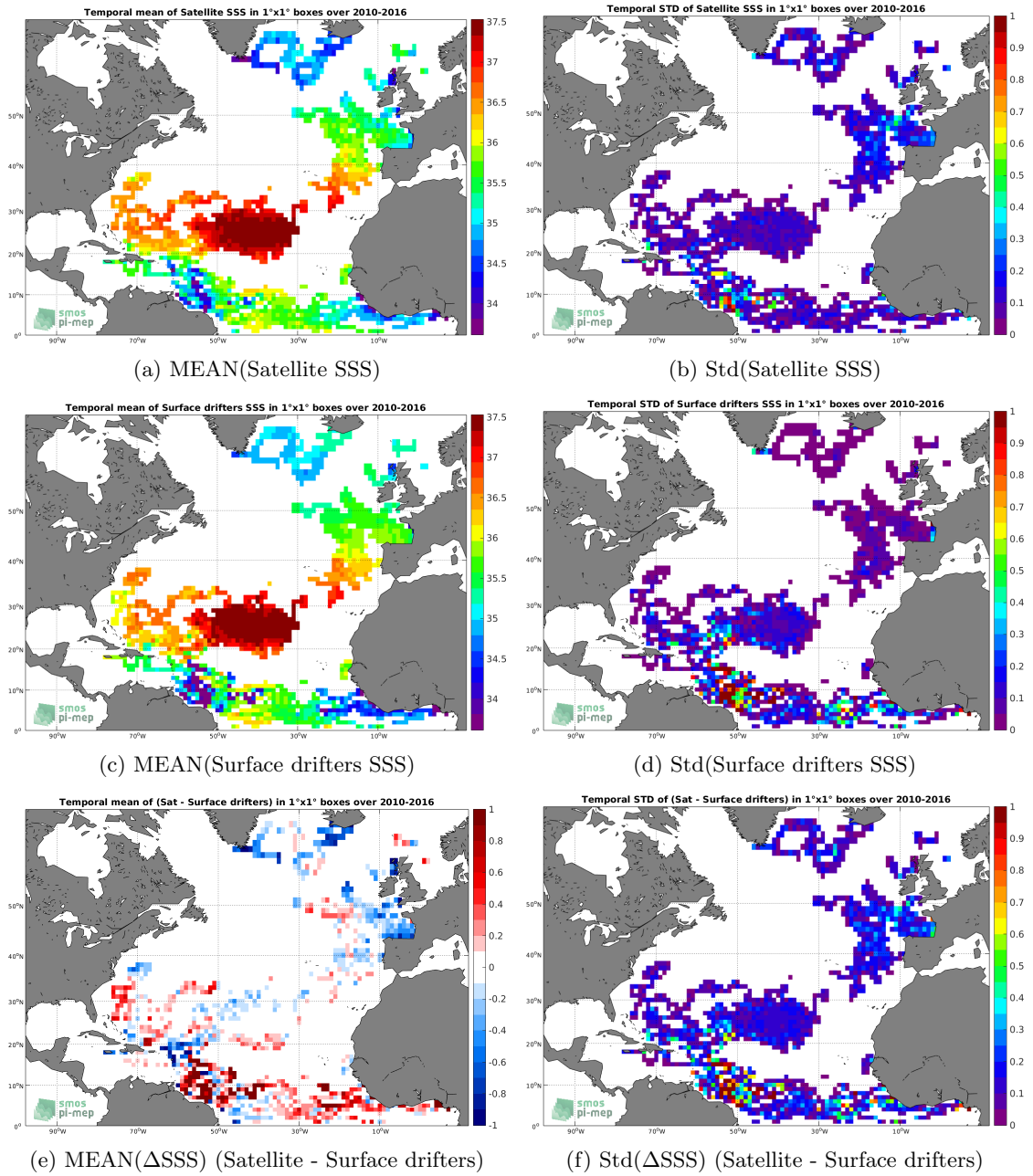
Figure 5: Temporal mean (left) and Std (right) of SSS from SMOS-L3-BEC-OA-V1-9DAYS-0.25DEG (top), Surface drifters (middle), and of \Delta SSS (Satellite - Surface drifters). Only match-up pairs are used to generate these maps.
