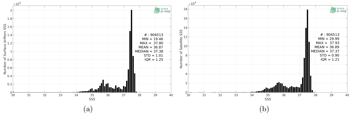
Figure 2: Histograms of SSS from Surface drifters (a) and SMOS-L3-BEC-OA-V1-9DAYS-0.25DEG (b) considering all match-up pairs per bins of 0.1 over the North Atlantic Ocean Pi-MEP region and for the full satellite product period.
