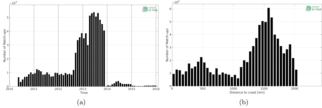
Figure 1: Number of match-ups between Surface drifters and SMOS-L3-BEC-OA-V1-9DAYS-0.25DEG SSS as a function of time (a) and as function of the distance to coast (b) over the North Atlantic Ocean Pi-MEP region and for the full satellite product period.
