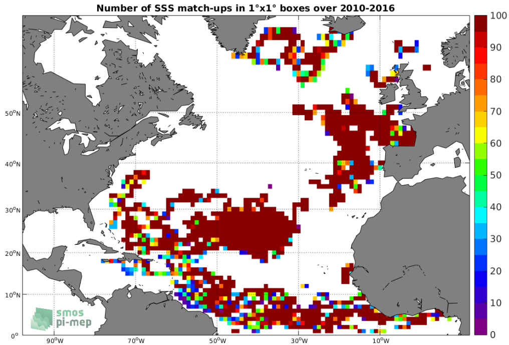
Figure 3: Number of SSS match-ups between Surface drifters SSS and the SMOS-L3-BEC-OA-V1-9DAYS-0.25DEG SSS product for the North Atlantic Ocean Pi-MEP region over 1^\circ \times 1^\circ boxes and for the full satellite product period.
