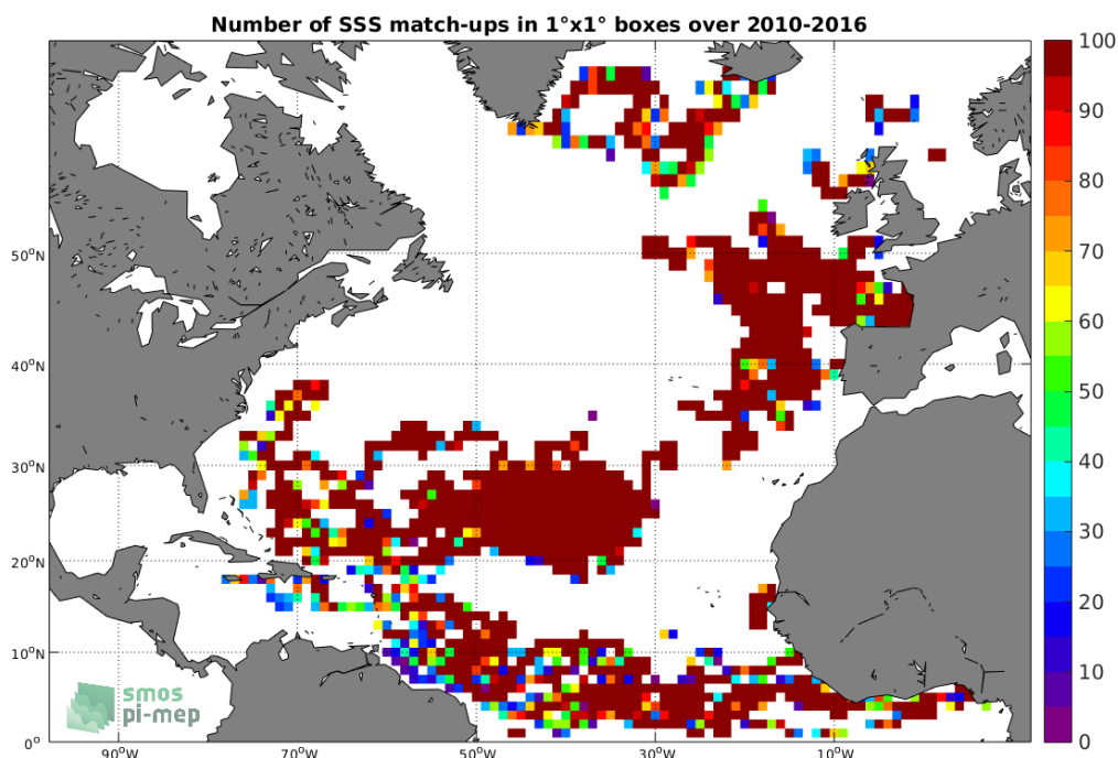
Figure 3: Number of SSS match-ups between Surface drifters SSS and the SMOS-L3-BEC-OA-V1-9DAYS-0.25DEG SSS product for the North Atlantic Ocean Pi-MEP region over 1^{\circ} \times 1^{\circ} boxes and for the full satellite product period.
