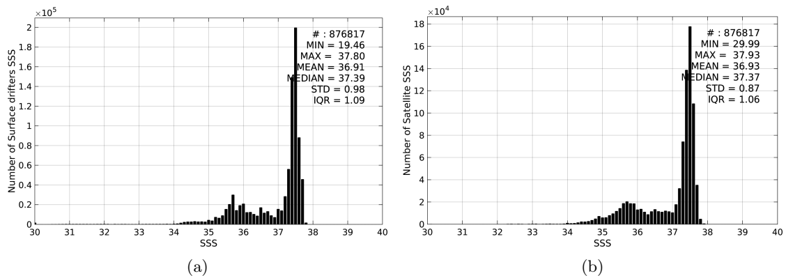
Figure 2: Histograms of SSS from Surface drifters (a) and SMOS-L3-BEC-OA-V1-9DAYS-0.25DEG (b) considering all match-up pairs per bins of 0.1 over the North Atlantic Ocean Pi-MEP region and for the full satellite product period.
