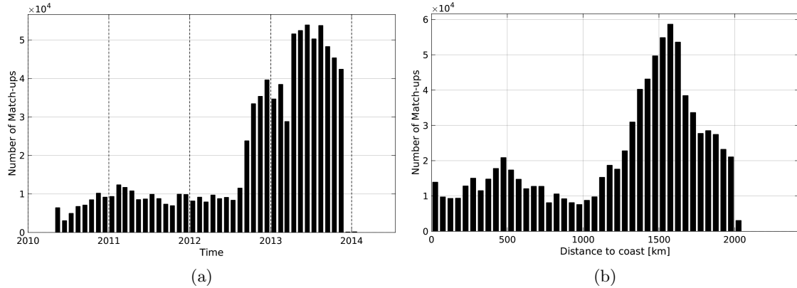
Figure 1: Number of match-ups between Surface drifters and SMOS-L3-BEC-OA-V1-9DAYS-0.25DEG SSS as a function of time (a) and as function of the distance to coast (b) over the North Atlantic Ocean Pi-MEP region and for the full satellite product period.
