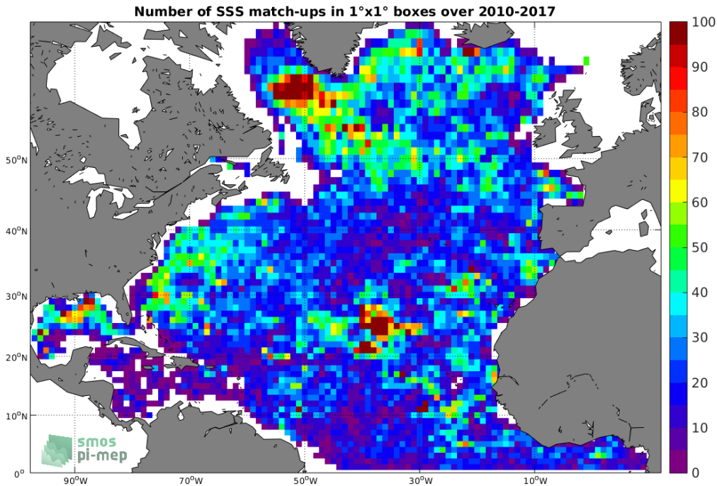
Figure 4: Number of SSS match-ups between Argo SSS and the SMOS-L3-BEC-OA-V1-9DAYS-0.25DEG SSS product for the North Atlantic Ocean Pi-MEP region over 1°x1° boxes and for the full satellite product period.
