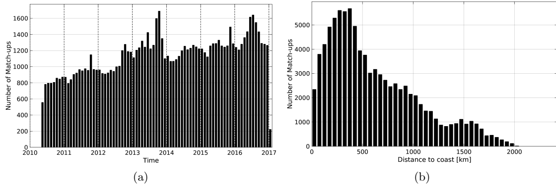
Figure 1: Number of match-ups between Argo and SMOS-L3-BEC-OA-V1-9DAYS-0.25DEG SSS as a function of time (a) and as function of the distance to coast (b) over the North Atlantic Ocean Pi-MEP region and for the full satellite product period.
