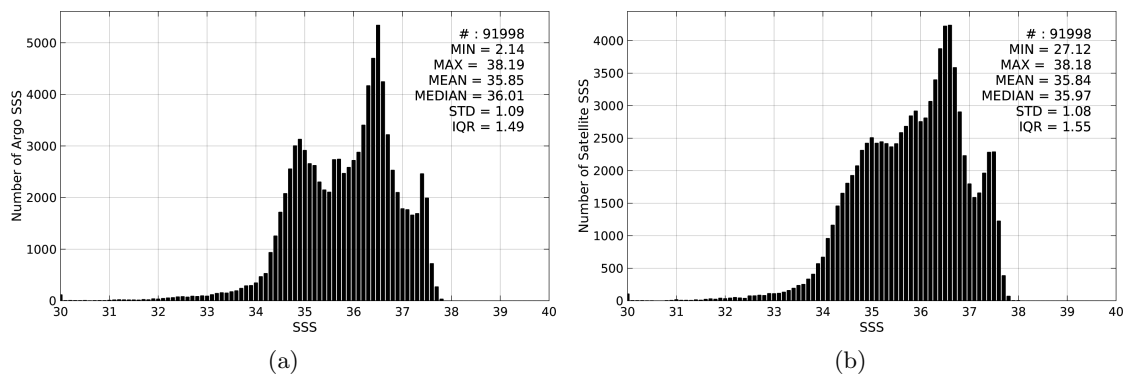
Figure 2: Histograms of SSS from Argo (a) and SMOS-L3-BEC-OA-V1-9DAYS-0.25DEG (b) considering all match-up pairs per bins of 0.1 over the North Atlantic Ocean Pi-MEP region and for the full satellite product period.
