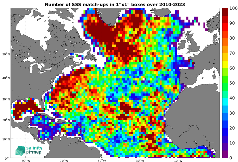
Figure 4: Number of SSS match-ups between Argo SSS and the SMOS SSS L2-AVERAGED v700 (ESA) SSS product for the North Atlantic Ocean Pi-MEP region over 1^\circ \times 1^\circ boxes and for the full satellite product period.
