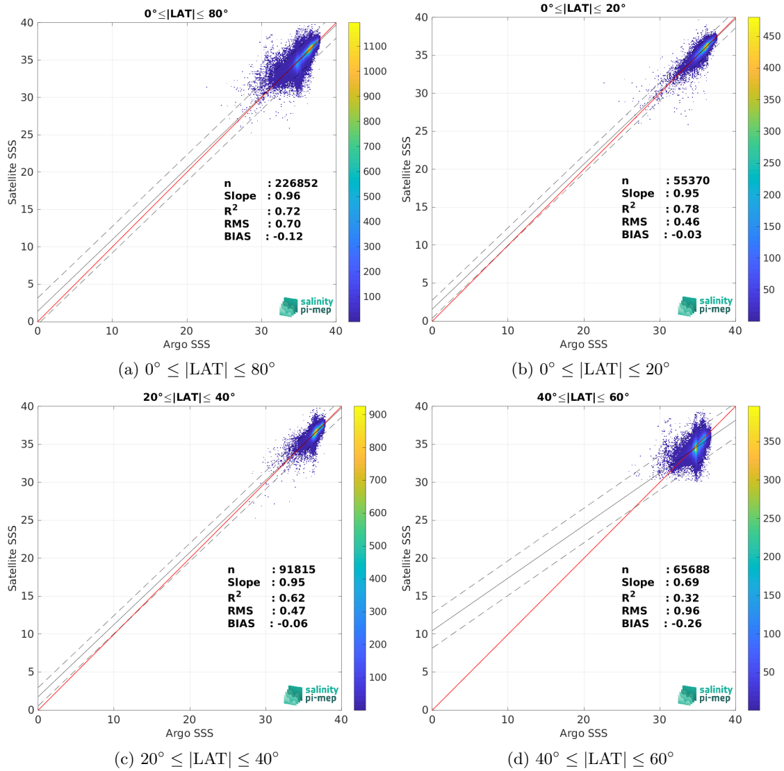
Figure 9: Contour maps of the concentration of SMOS SSS L2-AVERAGED v700 (ESA) SSS (y-axis) versus Argo SSS (x-axis) at match-up pairs for different latitude bands. For each plot, the red line shows x=y . The black thin and dashed lines indicate a linear fit through the data cloud and the \pm 95\% confidence levels, respectively. The number match-up pairs n , the slope and R^2 coefficient of the linear fit, the root mean square (RMS) and the mean bias between satellite and in situ data are indicated for each latitude band in each plots.
