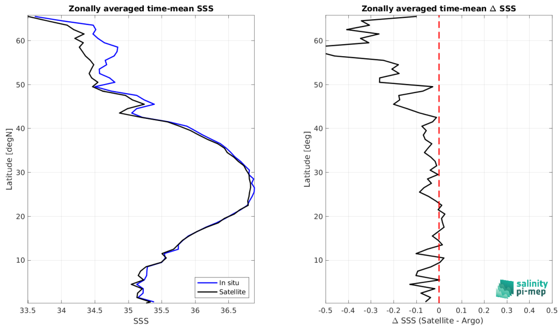
Figure 8: Left panel: Zonal mean SSS from SMOS SSS L2-AVERAGED v700 (ESA) satellite product (black) and from Argo (blue). Right panel: Zonal mean of \Delta SSS (Satellite - Argo) for all the collected Pi-MEP match-up pairs estimated over the full satellite product period.
