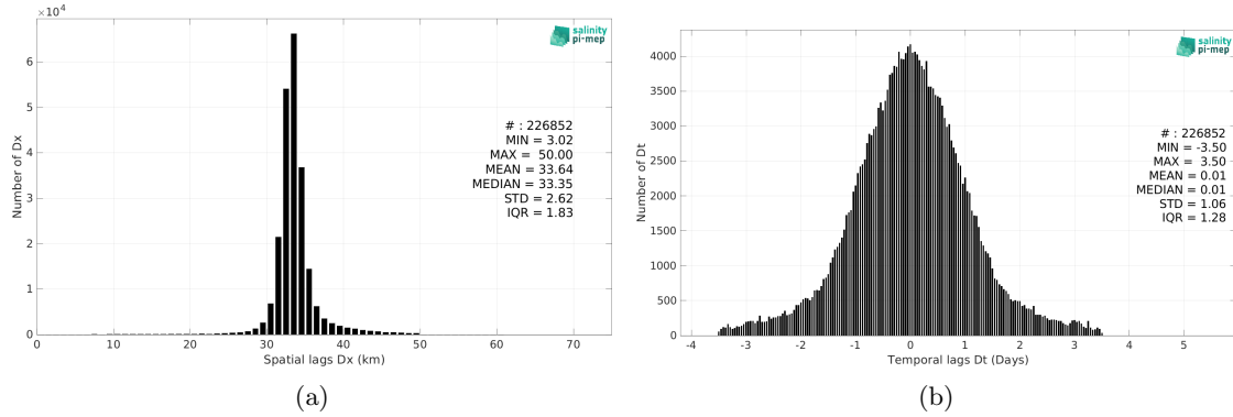
Figure 5: Histograms of the spatial (a) and temporal (b) lags between the location/time of the Argo measurement and the date of the corresponding SMOS SSS L2-AVERAGED v700 (ESA) SSS pixel.
