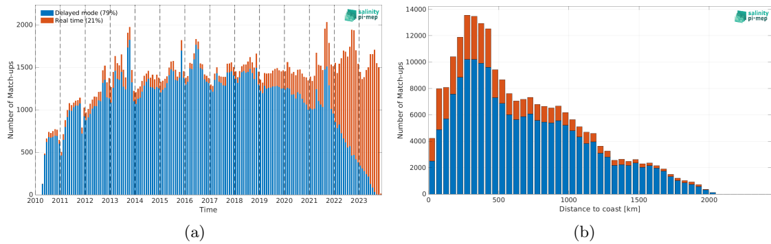
Figure 1: Number of match-ups between Argo and SMOS SSS L2-AVERAGED v700 (ESA) SSS as a function of time (a) and as function of the distance to coast (b) over the North Atlantic Ocean Pi-MEP region and for the full satellite product period.
