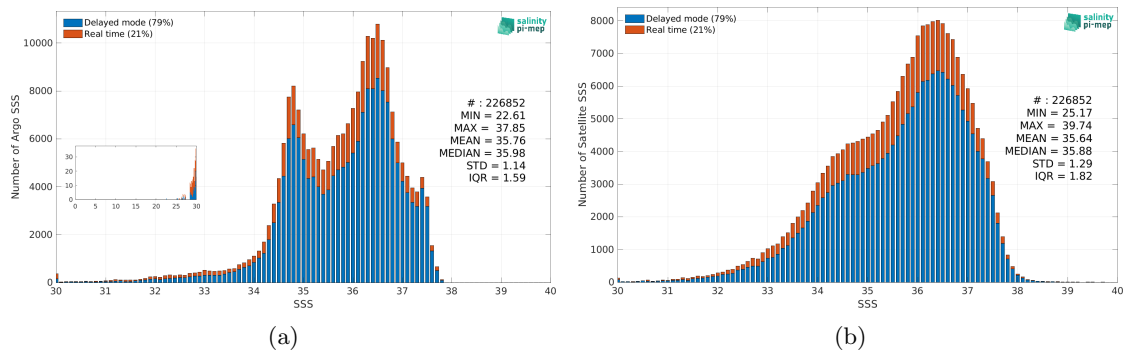
Figure 2: Histograms of SSS from Argo (a) and SMOS SSS L2-AVERAGED v700 (ESA) (b) considering all match-up pairs per bins of 0.1 over the North Atlantic Ocean Pi-MEP region and for the full satellite product period.
