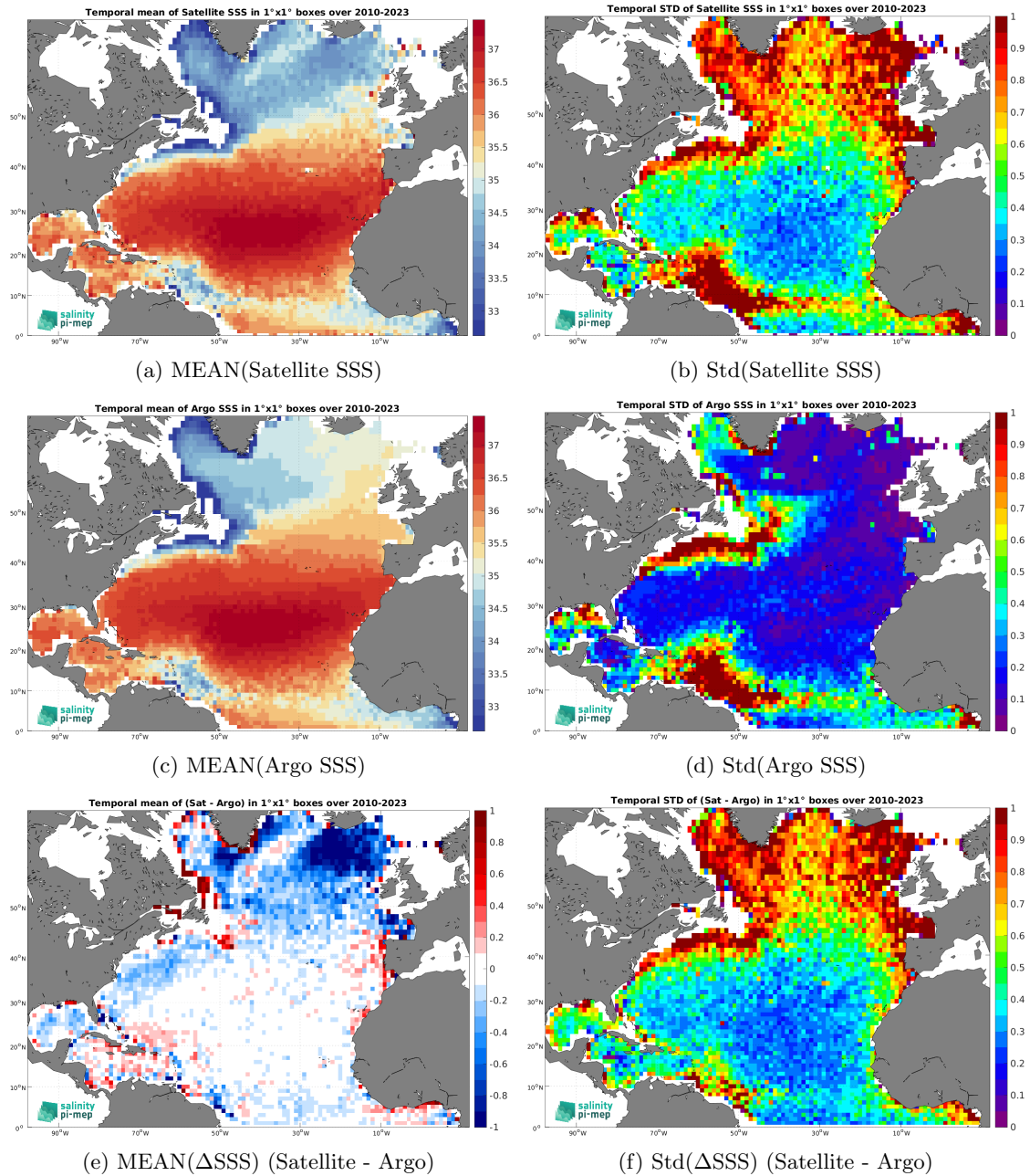
Figure 6: Temporal mean (left) and Std (right) of SSS from SMOS SSS L2-AVERAGED v700 (ESA) (top), Argo (middle), and of \Delta SSS (Satellite - Argo). Only match-up pairs are used to generate these maps.
