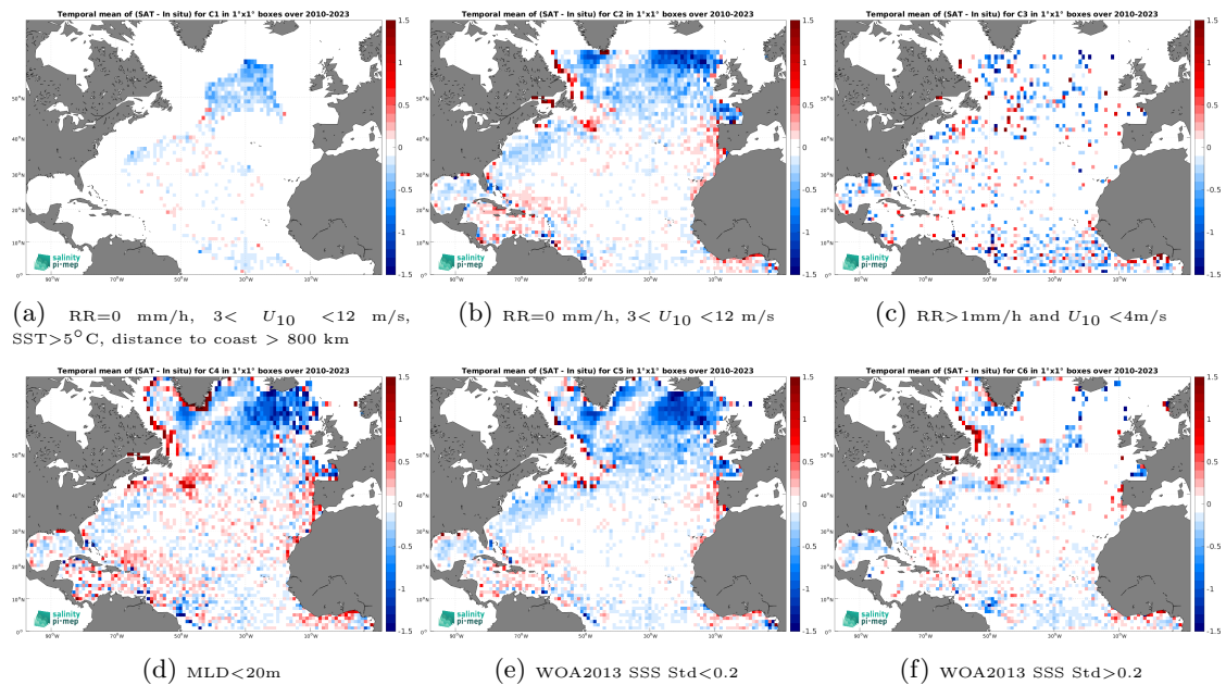
Figure 12: Temporal mean gridded over spatial boxes of size 1^\circ \times 1^\circ of \Delta SSS (SMOS SSS L2-AVERAGED v700 (ESA) - Argo) for 6 different subdatasets corresponding to:RR=0 mm/h, 3 < U_{10} < 12 m/s, SST > 5^\circ\text{C} , distance to coast > 800 km (a), RR=0 mm/h, 3 < U_{10} < 12 m/s (b), RR > 1 mm/h and U_{10} < 4 m/s (c),MLD < 20 m (d),WOA2013 SSS Std < 0.2 (e),WOA2013 SSS Std > 0.2 (f).
