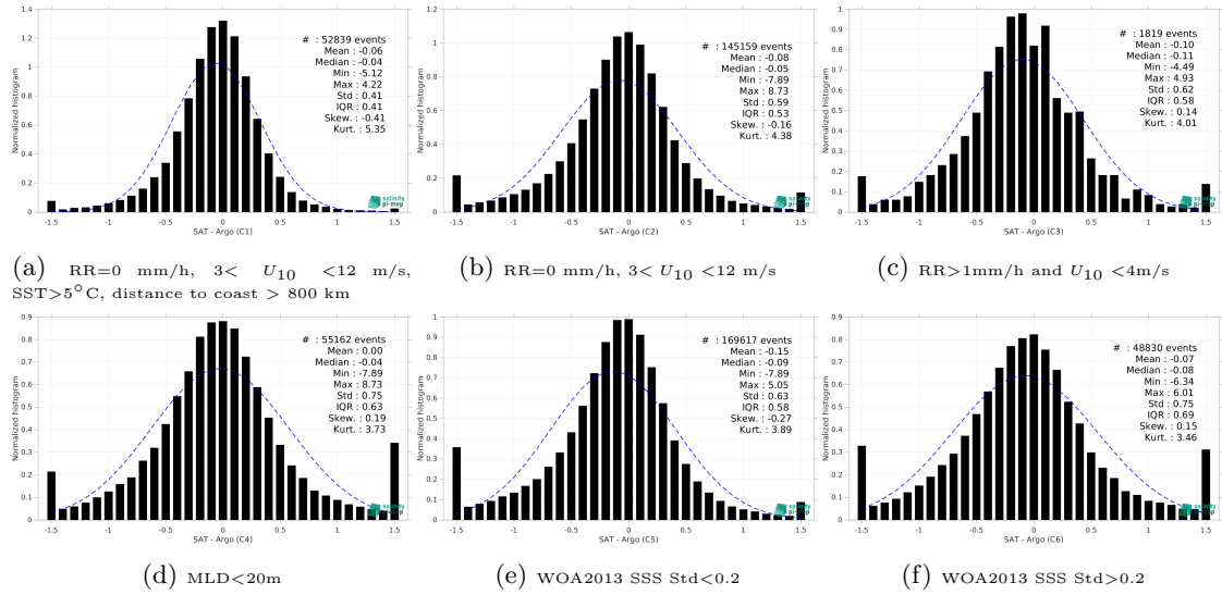
Figure 13: Normalized histogram of \Delta SSS (SMOS SSS L2-AVERAGED v700 (ESA) - Argo) for 6 different subdatasets corresponding to: RR=0 mm/h, 3 < U_{10} < 12 m/s, SST>5°C, distance to coast > 800 km (a), RR=0 mm/h, 3 < U_{10} < 12 m/s (b), RR>1mm/h and U_{10} < 4 m/s (c), MLD<20m (d), WOA2013 SSS Std<0.2 (e), WOA2013 SSS Std>0.2 (f).
