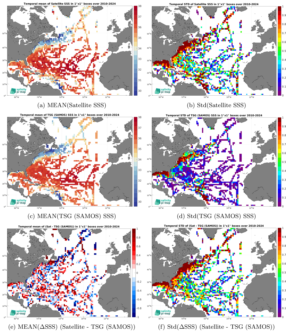
Figure 7: Temporal mean (left) and Std (right) of SSS from SMOS SSS L2 v700 (ESA) (top), TSG (SAMOS) (middle), and of \Delta SSS (Satellite - TSG (SAMOS)). Only match-up pairs are used to generate these maps.
