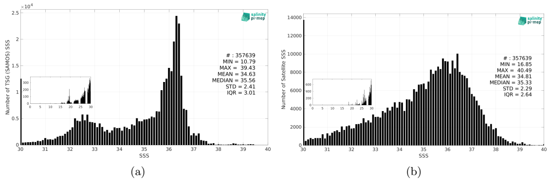
Figure 3: Histograms of SSS from TSG (SAMOS) (a) and SMOS SSS L2 v700 (ESA) (b) considering all match-up pairs per bins of 0.1 over the North Atlantic Ocean Pi-MEP region and for the full satellite product period.
