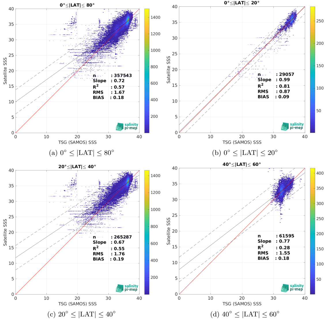
Figure 10: Contour maps of the concentration of SMOS SSS L2 v700 (ESA) SSS (y-axis) versus TSG (SAMOS) SSS (x-axis) at match-up pairs for different latitude bands. For each plot, the red line shows x=y . The black thin and dashed lines indicate a linear fit through the data cloud and the \pm 95\% confidence levels, respectively. The number match-up pairs n , the slope and R^2 coefficient of the linear fit, the root mean square (RMS) and the mean bias between satellite and in situ data are indicated for each latitude band in each plots.
