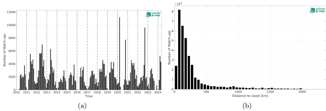
Figure 2: Number of match-ups between TSG (SAMOS) and SMOS SSS L2 v700 (ESA) SSS as a function of time (a) and as function of the distance to coast (b) over the North Atlantic Ocean Pi-MEP region and for the full satellite product period.
