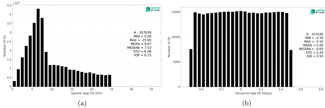
Figure 6: Histograms of the spatial (a) and temporal (b) lags between the location/time of the TSG (SAMOS) measurement and the date of the corresponding SMOS SSS L2 v700 (ESA) SSS pixel.
