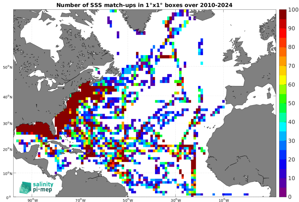
Figure 5: Number of SSS match-ups between TSG (SAMOS) SSS and the SMOS SSS L2 v700 (ESA) SSS product for the North Atlantic Ocean Pi-MEP region over 1^\circ \times 1^\circ boxes and for the full satellite product period.
