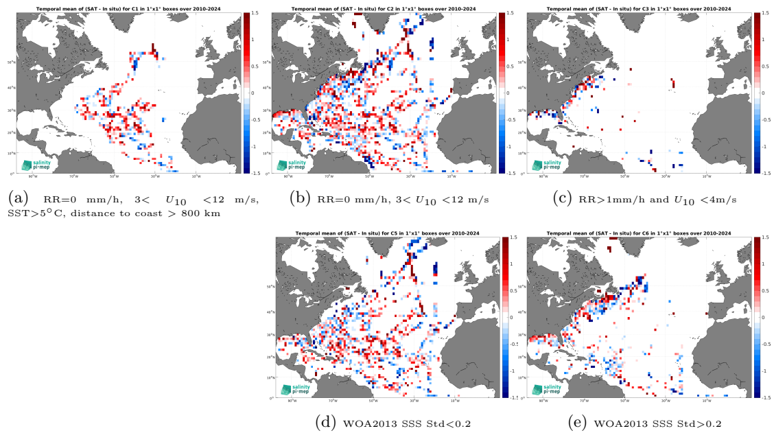
Figure 14: Temporal mean gridded over spatial boxes of size 1^\circ \times 1^\circ of \Delta SSS (SMOS SSS L2 v700 (ESA) - TSG (SAMOS)) for 5 different subdatasets corresponding to:RR=0 mm/h, 3 < U_{10} < 12 m/s, SST>5°C, distance to coast > 800 km (a), RR=0 mm/h, 3 < U_{10} < 12 m/s (b), RR>1mm/h and U_{10} < 4 m/s (c), WOA2013 SSS Std<0.2 (d), WOA2013 SSS Std>0.2 (e).
